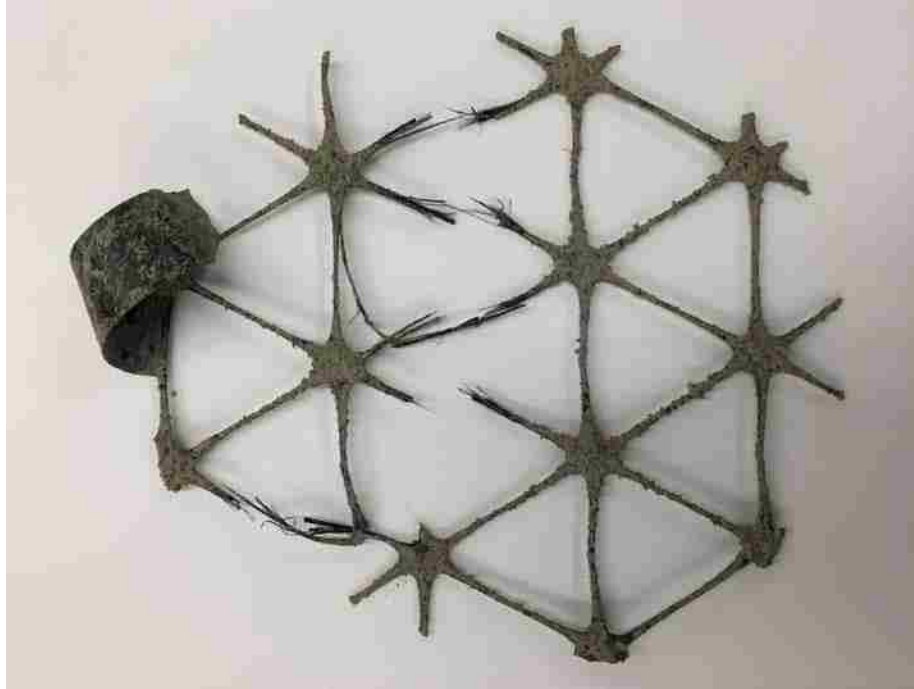
Figure 4-2: Geogrid rib failure.
