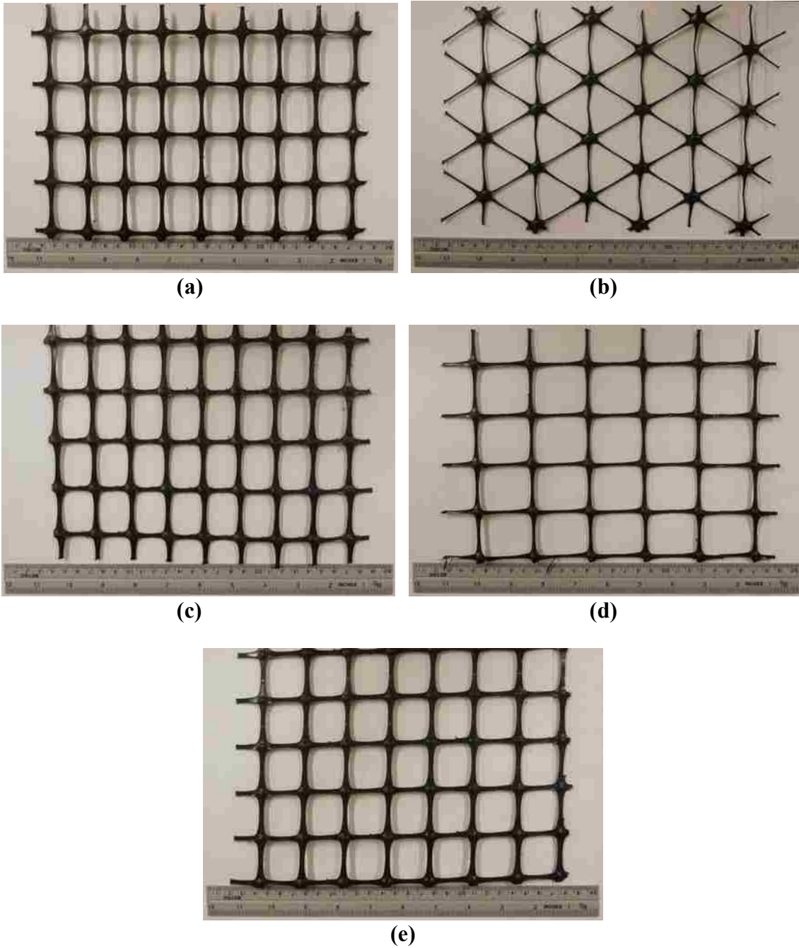
Figure 3-4: Geogrid products used in this research: (a) A, (b) B, (c) C, (d) D, and (e) E.
