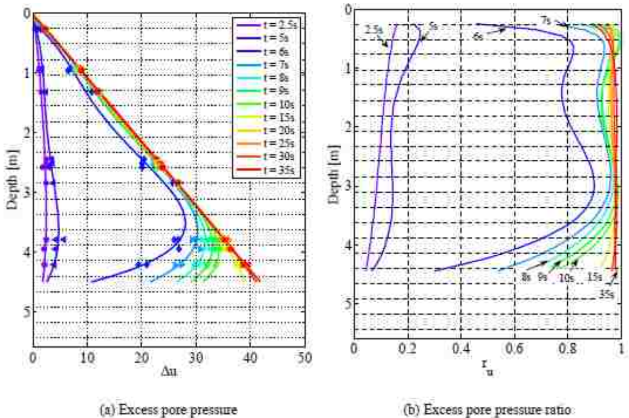
Figure 2-13 Excess Pore Pressure Profiles for LG0 (Bethapudi 2008).
