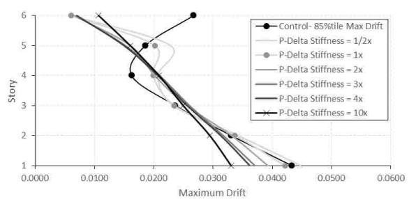
Figure D-58. Average & 85%tile maximum drifts for 2× ES at level 6, 6S.
