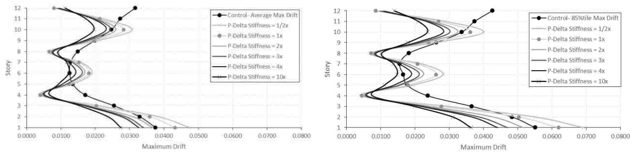
Figure F-14. Average & 85%tile maximum drifts for 4× ES at level 4, 8, & 12, 12S.
