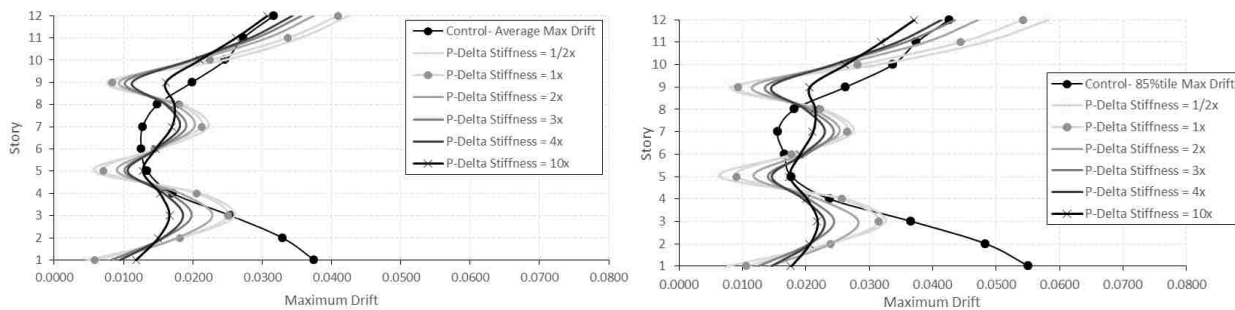
Figure F-2. Average & 85%tile maximum drifts for 2 \times ES at level 1, 5, & 9, 12S.
