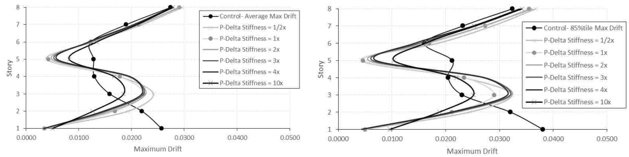
Figure E-4. Average & 85%tile maximum drifts for 3× ES at level 1&5, 8S.
