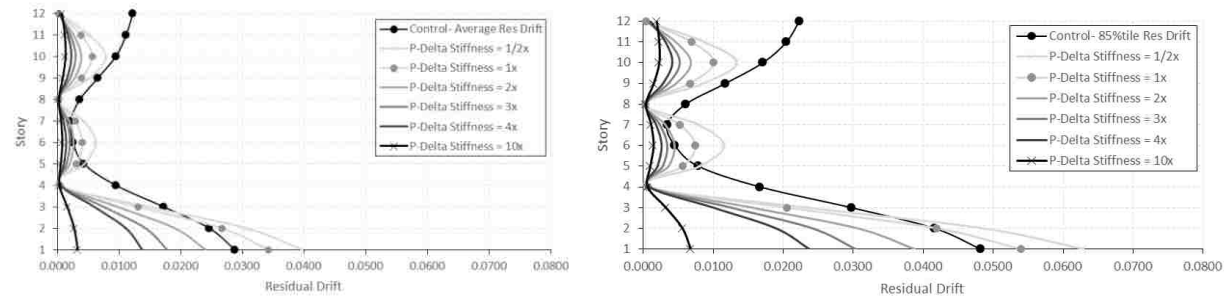
Figure F-13. Average & 85%tile residual drifts for 4× ES at level 4, 8, & 12, 12S.
