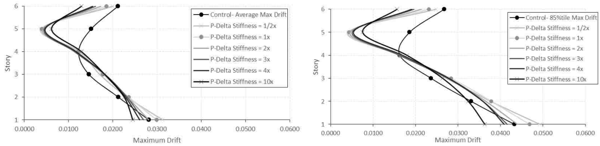
Figure D-52. Average & 85%tile maximum drifts for 3× ES at level 5, 6S.
