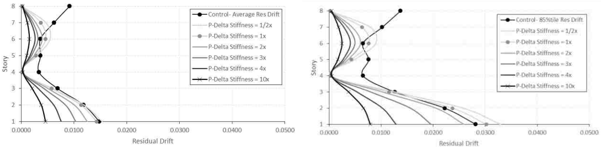
Figure E-13. Average & 85%tile residual drifts for 4× ES at level 4&8, 8S.
