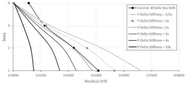
Figure C-15. Average & 85%tile residual drifts for 10× ES at level 4, 4S.
