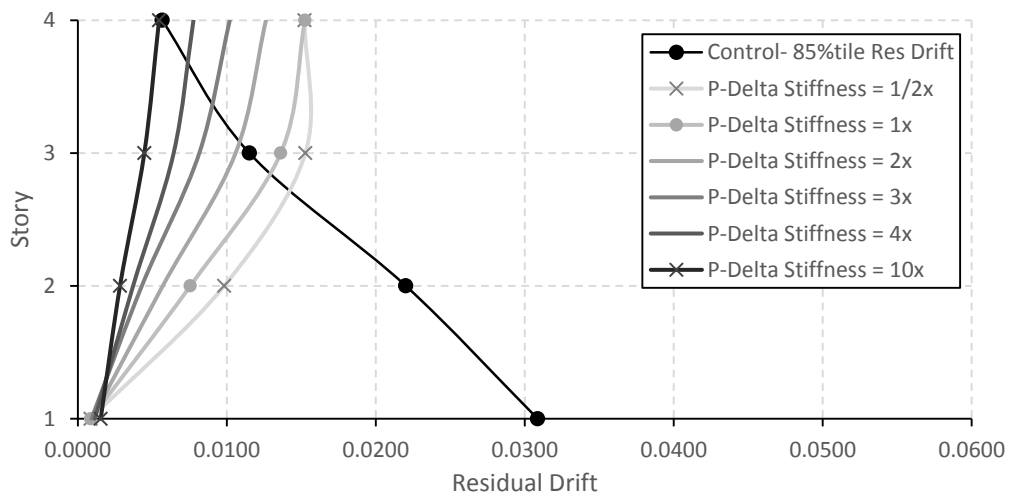
Figure 4-2. 85%tile residual drifts for 3x ES at level 1, 4S.
