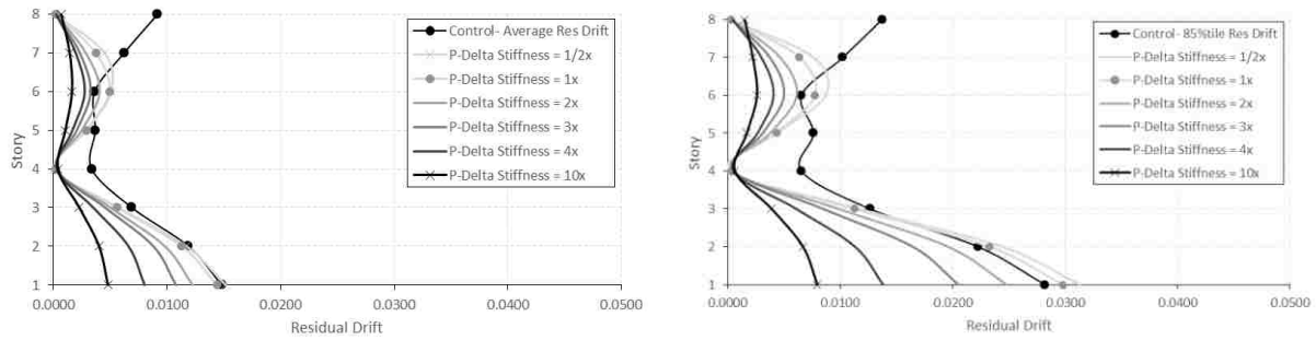
Figure E-11. Average & 85%tile residual drifts for 3× ES at level 4&8, 8S.
