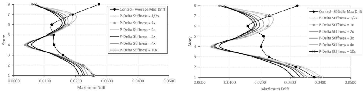
Figure E-12. Average & 85%tile maximum drifts for 3× ES at level 4&8, 8S.
