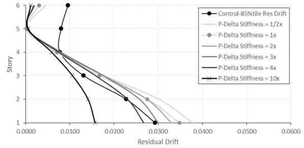
Figure D-55. Average & 85%tile residual Drifts for 10× ES at level 5, 6S.
