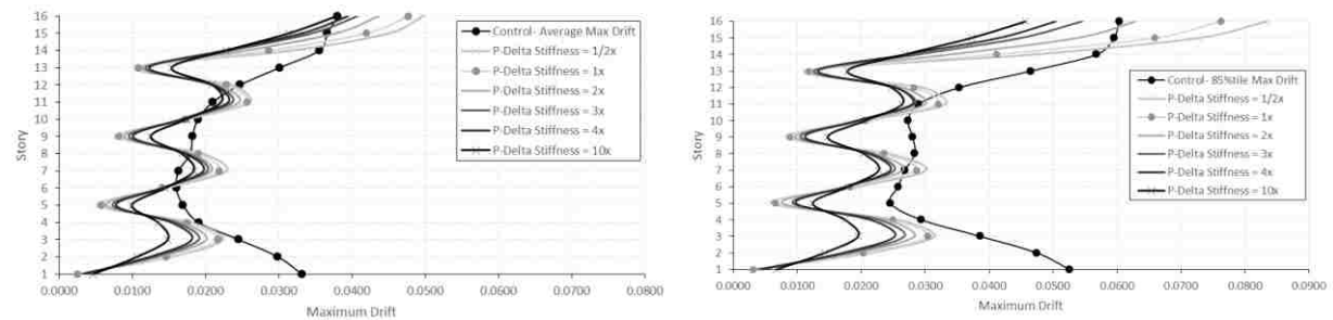
Figure G-6. Average & 85%tile maximum drifts for 4× ES at level 1, 5, 9, & 13, 16S.
