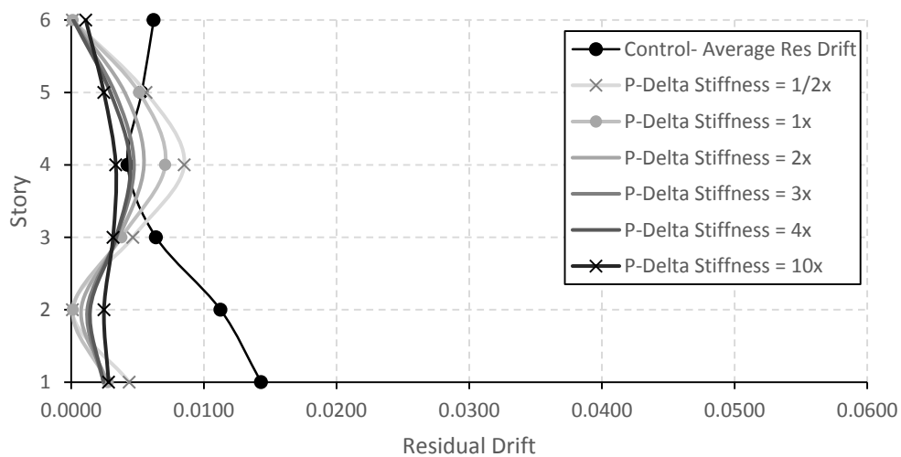
Figure 4-9. Average residual drifts for 3× ES at level 2&6, 6S.
