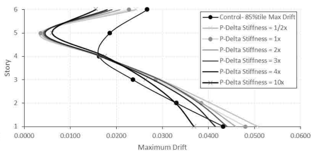
Figure D-56. Average & 85%tile maximum drifts for 10× ES at level 5, 6S.
