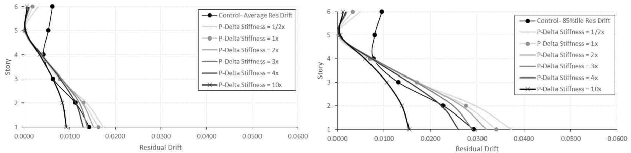
Figure D-53. Average & 85%tile residual drifts for 4× ES at level 5, 6S.
