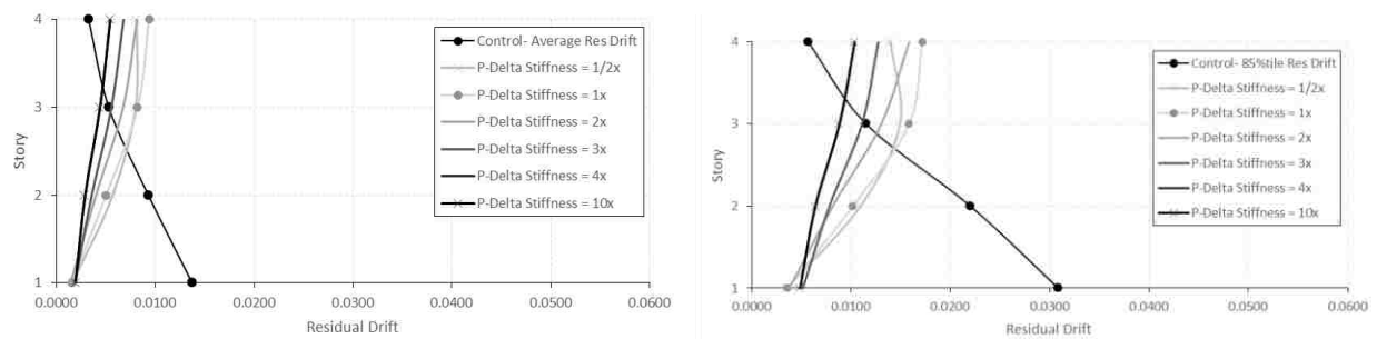
Figure C-1. Average & 85%tile residual drifts for 2× ES at level 1, 4S.
