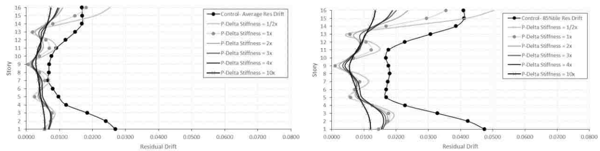
Figure G-1. Average & 85%tile residual drifts for 2× ES at level 1, 5, 9, & 13, 16S.
