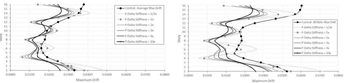
Figure G-10. Average & 85%tile maximum drifts for 2× ES at level 4, 8, 12, & 16, 16S.
