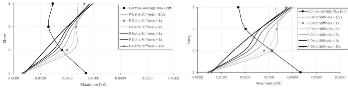
Figure C-4. Average & 85%tile maximum drifts for 3× ES at level 1, 4S.
