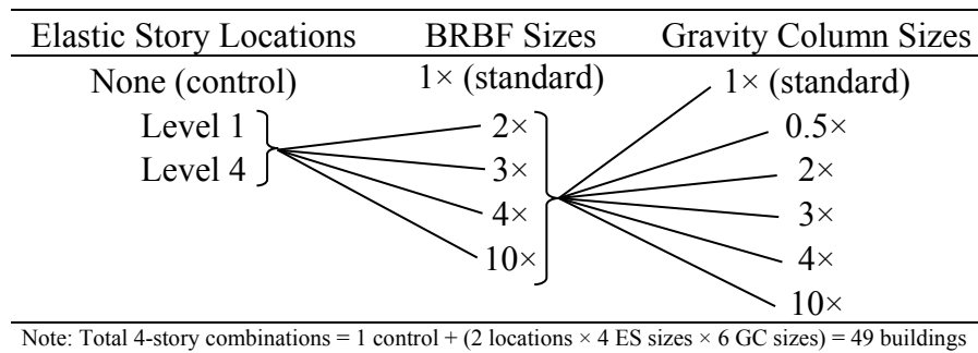
Figure 3-9. Four-story design buildings.
