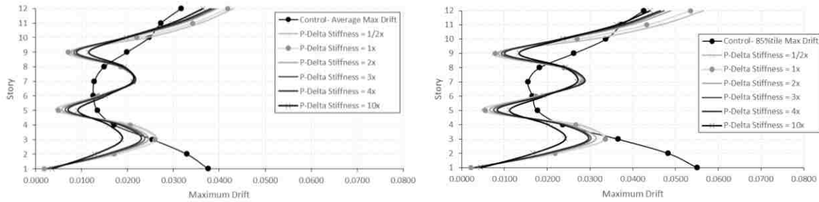
Figure F-8. Average & 85%tile maximum drifts for 10× ES at level 1, 5, & 12S.
