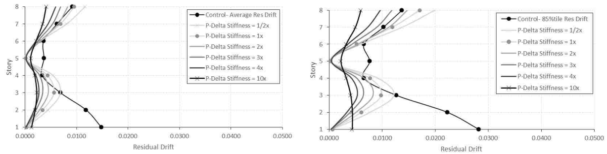
Figure E-3. Average & 85%tile residual drifts for 3× ES at level 1&5, 8S.
