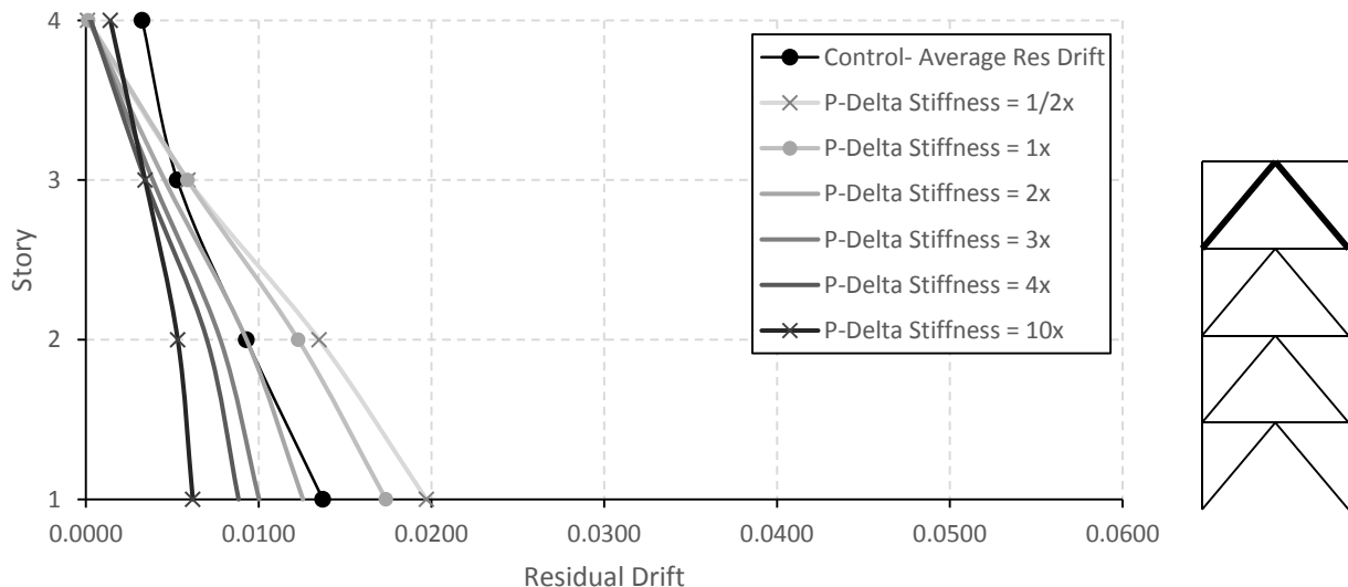
Figure 4-7. Average residual drifts for 3× ES at level 4, 4S.
