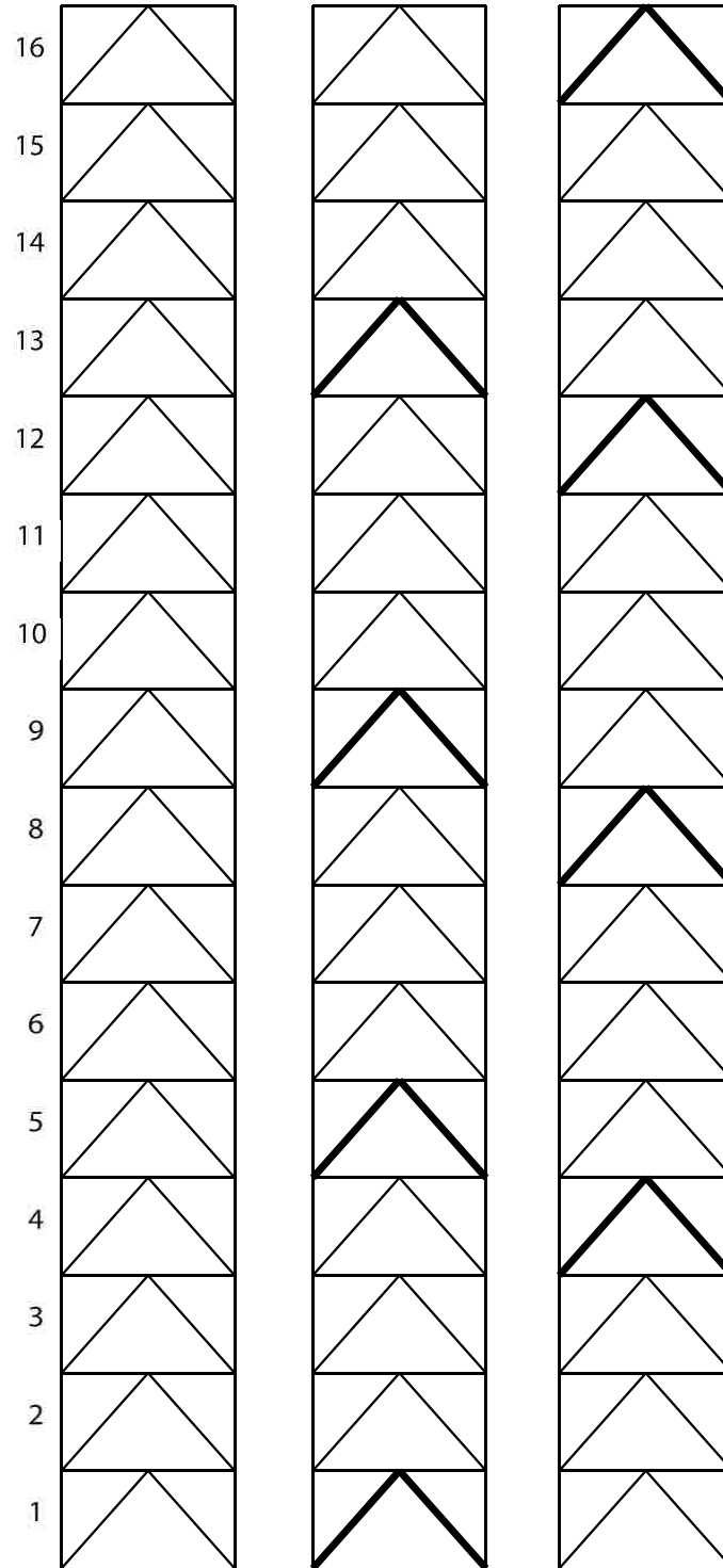
Figure 3-8. Elastic story combination locations for 16-story buildings.
