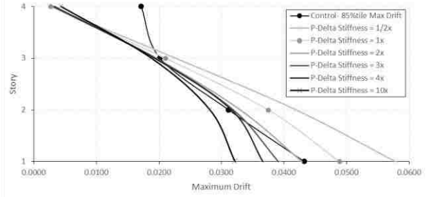
Figure C-16. Average & 85%tile maximum drifts for 10× ES at level 4, 4S.
