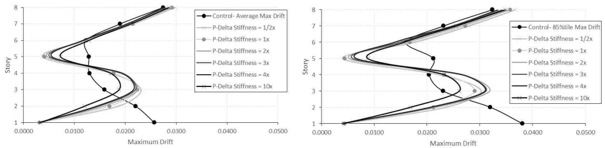
Figure E-6. Average & 85%tile maximum drifts for 4× ES at level 1&5, 8S
