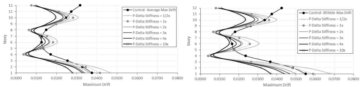
Figure F-16. Average & 85%tile maximum drifts for 10× ES at level 4, 8, & 12, 12S.
