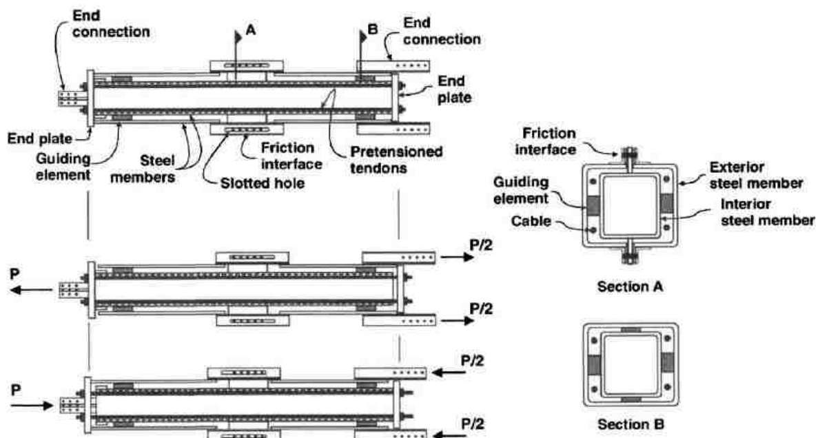
Figure 2-9. Embodiment of SCED system with steel tubes, tendons and dissipative mechanism [29].
