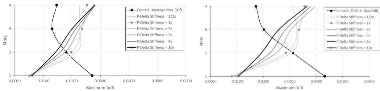
Figure C-2. Average & 85%tile maximum drifts for 2× ES at level 1, 4S.
