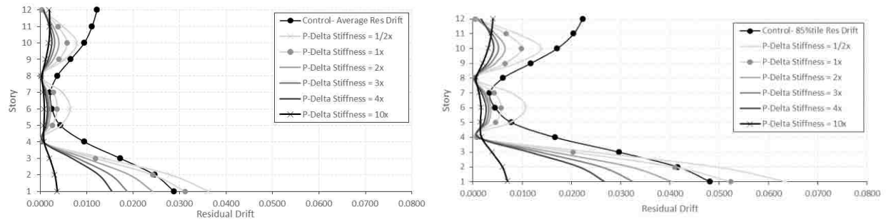
Figure F-11 Average & 85%tile residual drifts for 3× ES at level 4, 8, & 12, 12S.
