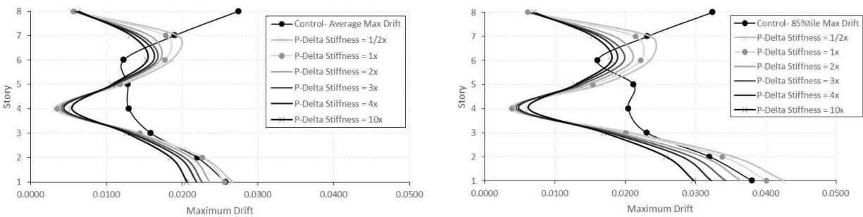
Figure E-14. Average & 85%tile maximum drifts for 4× ES at level 4&8, 8S.
