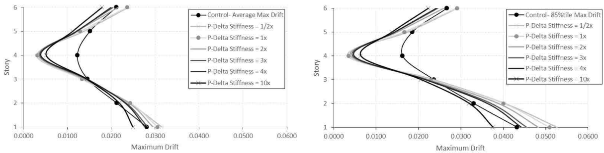
Figure D-46. Average & 85%tile maximum drifts for 4× ES at level 4, 6S.
