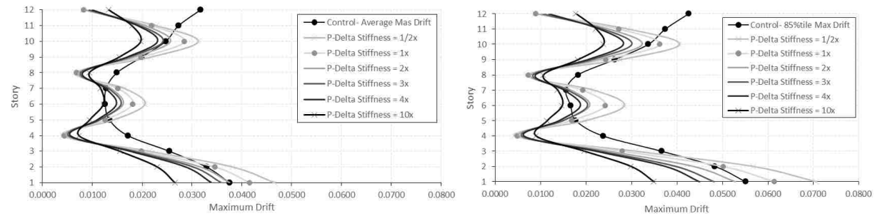
Figure F-12. Average & 85%tile maximum drifts for 3× ES at level 4, 8, & 12, 12S.
