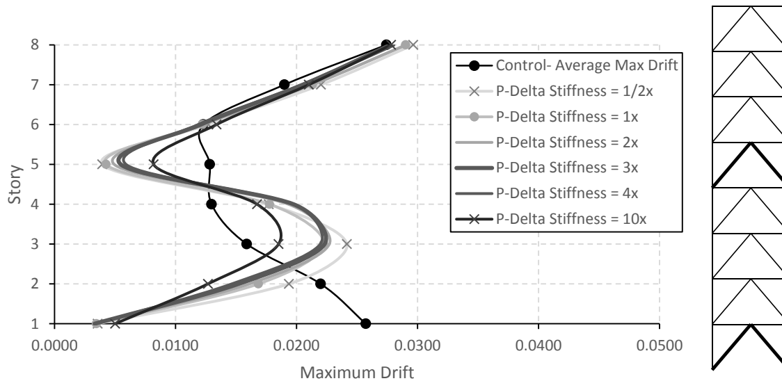
Figure 4-13. Average maximum drifts for 3x ES at level 1&5, 8S.
