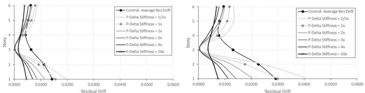
Figure D-35. Average & 85%tile residual drifts for 3× ES at level 3, 6S.
