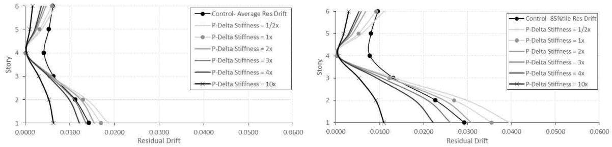
Figure D-47. Average & 85%tile residual drifts for 10× ES at level 4, 6S.
