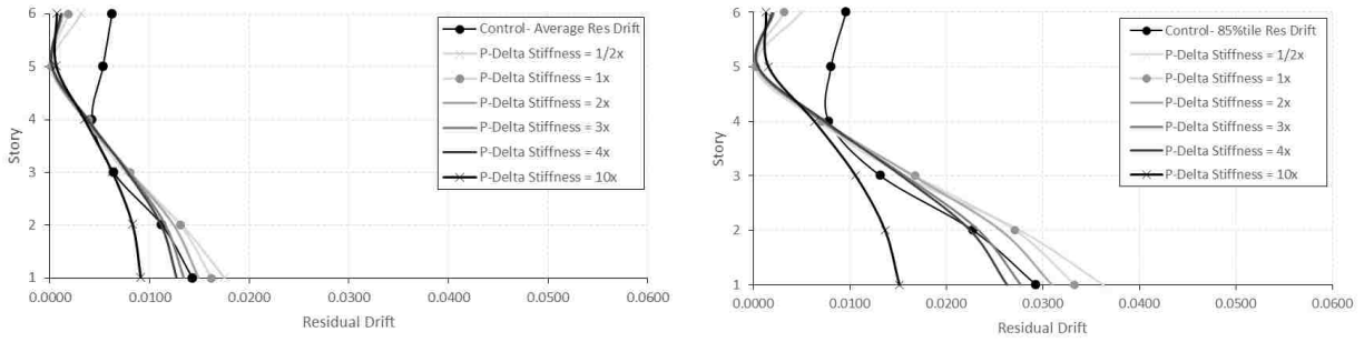
Figure D-51. Average & 85%tile residual drifts for 3× ES at level 5, 6S.
