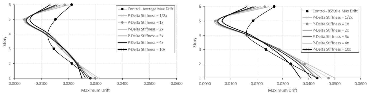
Figure D-54. Average & 85%tile maximum drifts for 4× ES at level 5, 6S.
