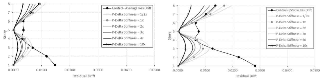
Figure E-5. Average & 85%tile residual drifts for 4× ES at level 1&5, 8S.
