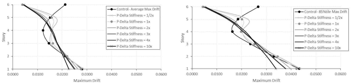
Figure D-64. Average & 85%tile maximum drifts for 10× ES at level 6, 6S.
