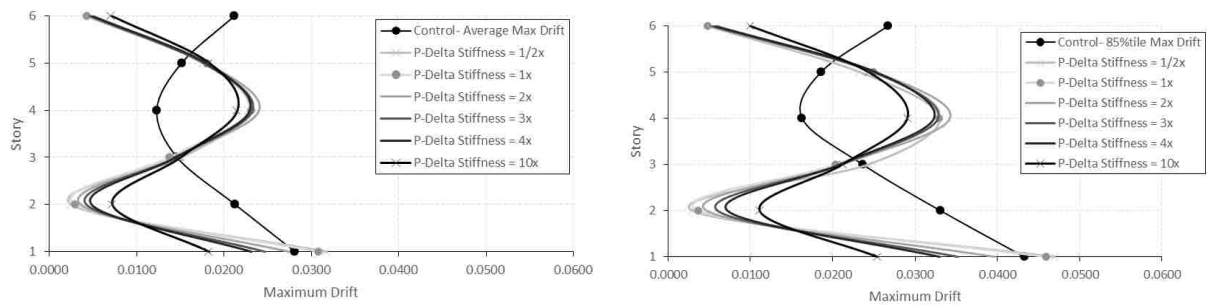
Figure D-14. Average & 85%tile maximum drifts for 4× ES at level 2&6, 6S.
