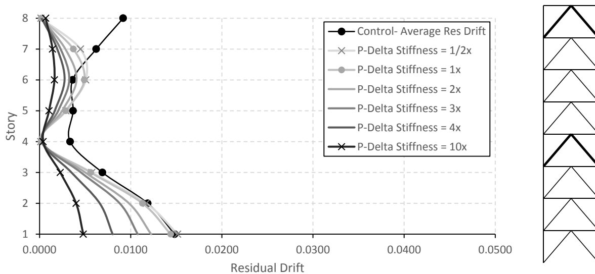
Figure 4-12. Average residual drifts for 3× ES at level 4&8, 8S.
