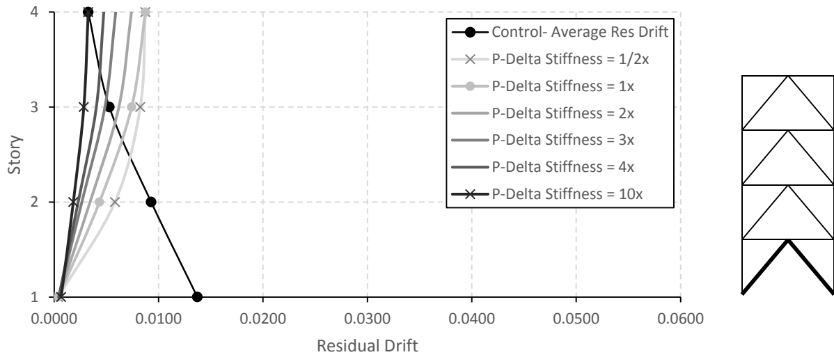
Figure 4-1. Average residual drifts for 3x ES at level 1, 4S.
