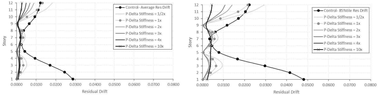
Figure F-5. Average & 85%tile residual drifts for 4× ES at level 1, 5, & 9, 12S.
