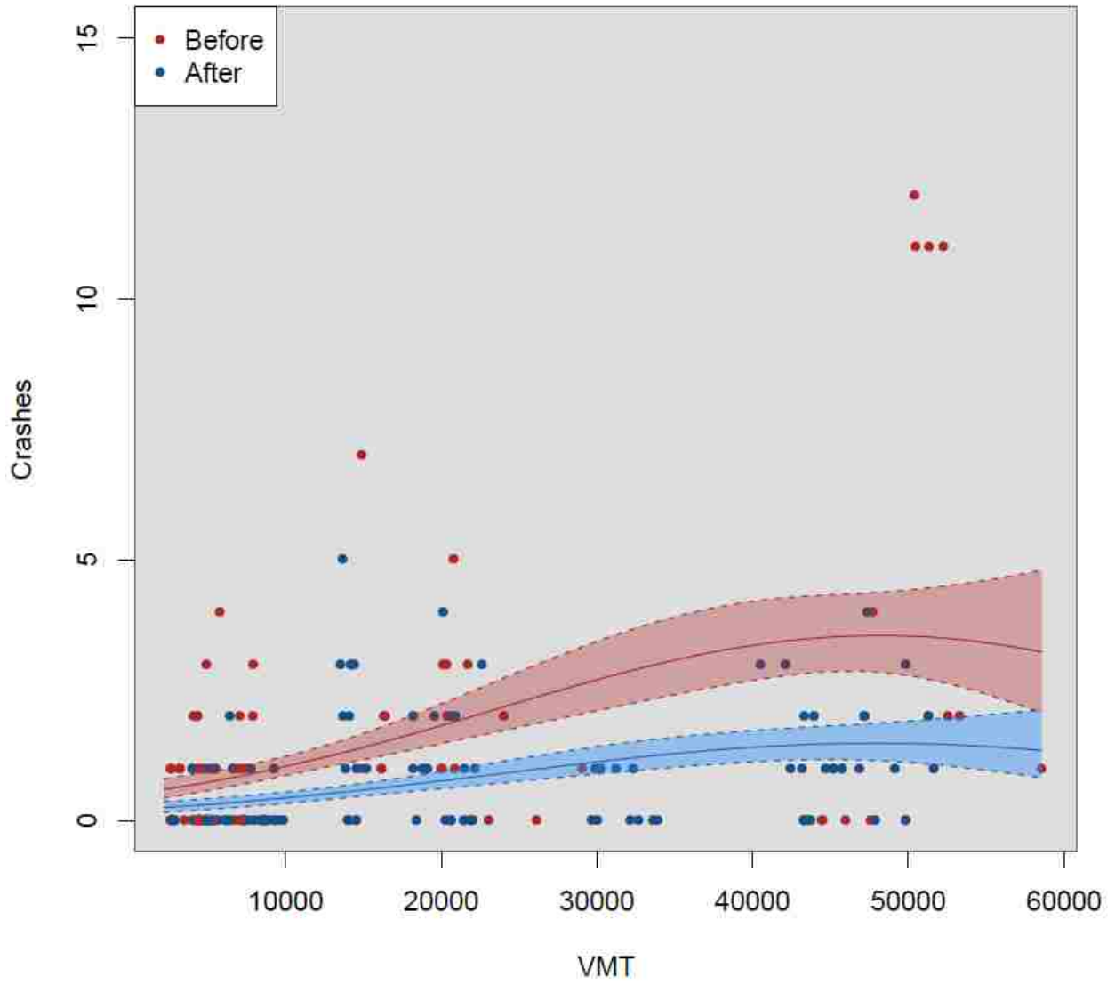
Figure C-26: Regression plot for AC 5 only including crashes with severity 4 and 5.
