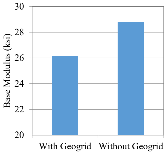
Figure A-10: Main effect of geogrid presence on base modulus measured with FWD at 10,000 lb at additional Springville site.
