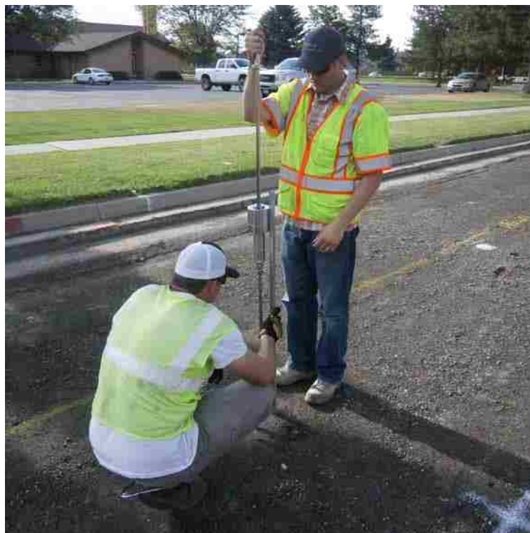
Figure 3-18: DCP testing of base layer.
