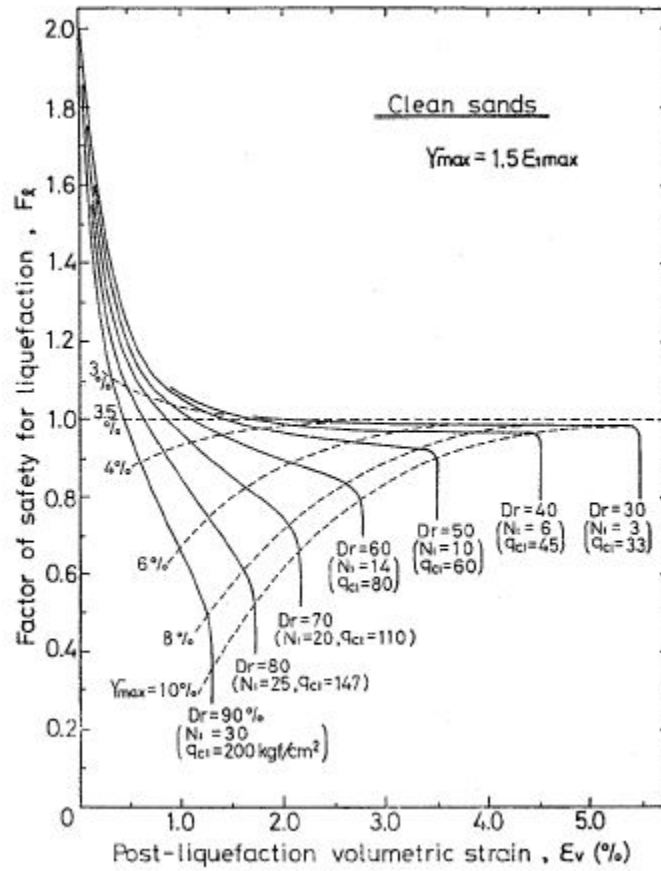
Figure 5-7: Ishihara and Yoshimine method for predicting volumetric strain (Ishihara and Yoshimine 1992)
