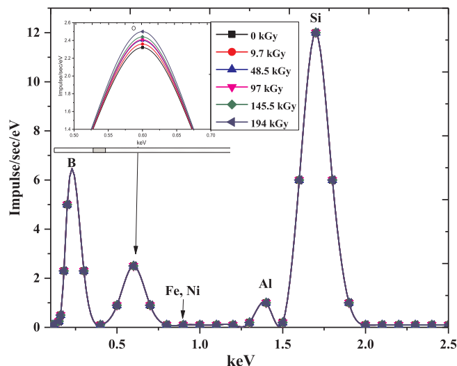
Fig. 4. Unirradiated and irradiated of sample distribution of chemical elements of silicide hexaboride.
