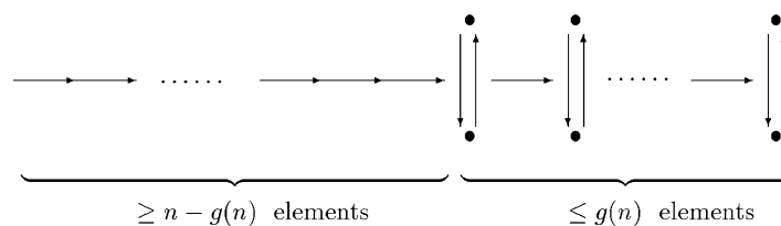
Fig. 1. A relation from \leq_{\uparrow g} .
