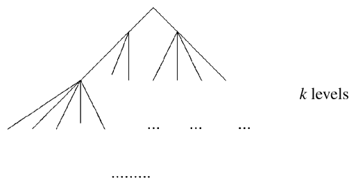
Fig. 2. Canonical k -bushy tree.
