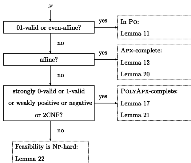
Fig. 2. The complexity of the maximum Hamming distance problem.
