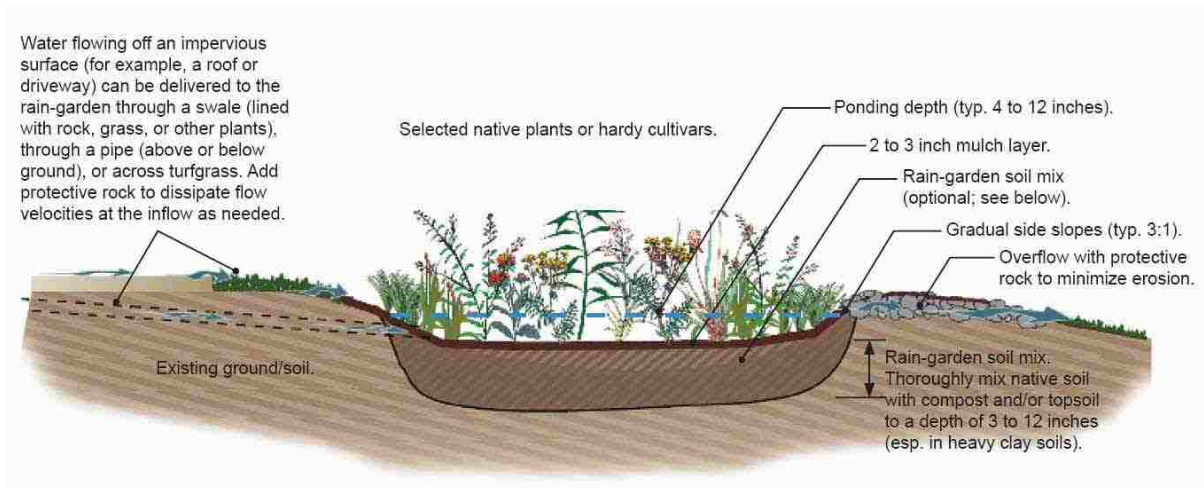
Figure 2. Cross section of rain garden (no under-drain system).
