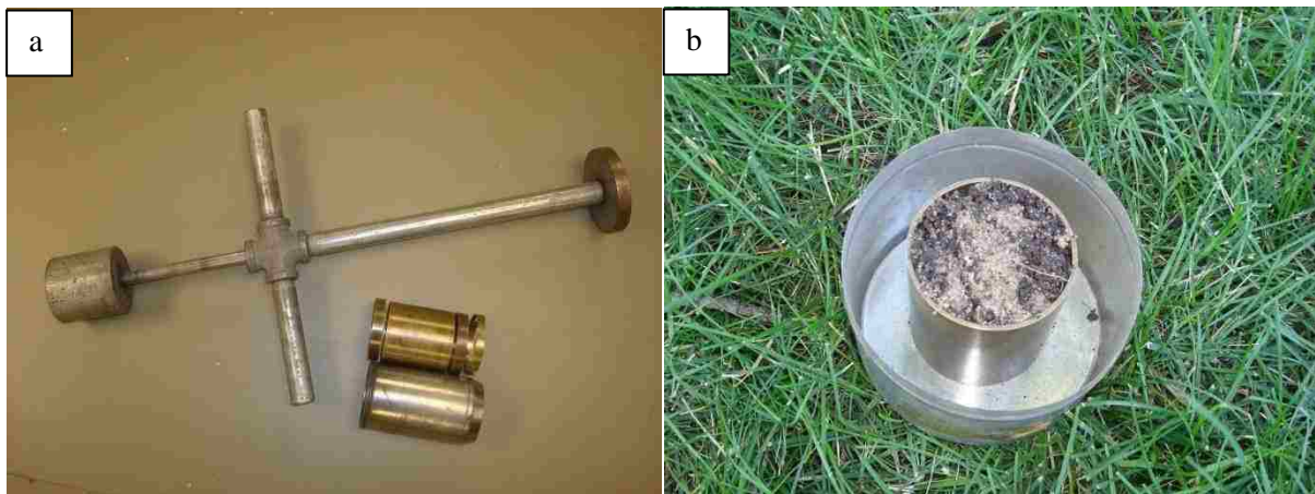
Figure 7. (a) Drop hammer and sharpened steel core with inner sampling ring for bulk density measurement. (b) Shaved soil core using collection equipment. Note the high sand content of the core indicates amendments were added.
