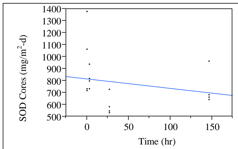
Figure 10. Regression plot of GLM analysis of SOD as measured in short cores collected from the tanks ( \text{mg}/\text{m}^2\text{-d} ) without a treatment effect (combined oxygenated and non-oxygenated data) (p-value: 0.3581, R^2 = 0.05 )
