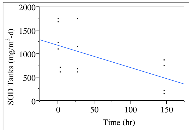
Figure 9. Regression plot of GLM analysis of SOD as measured using datasonde data in the tanks ( \text{mg}/\text{m}^2\text{-d} ) without a treatment effect (combined oxygenated and non-oxygenated data) (p-value: 0.0155, R^2 = 0.34 ).
