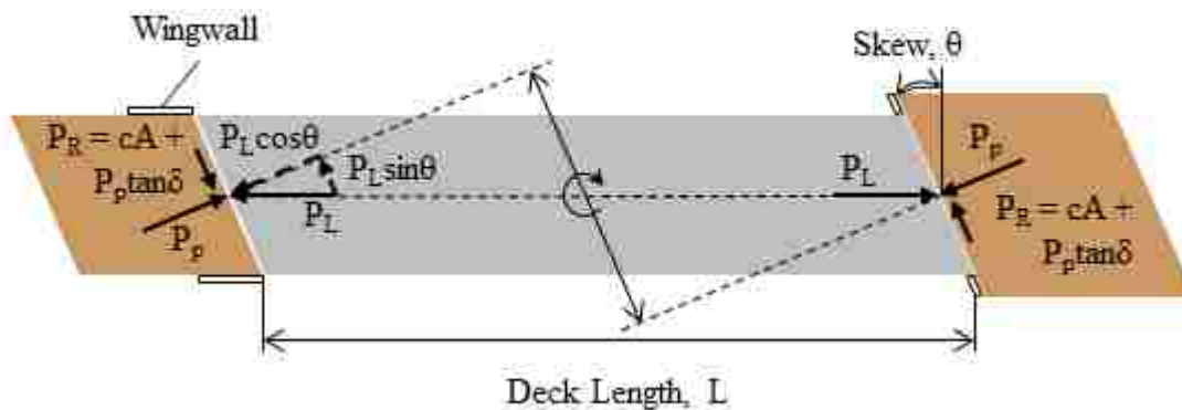
Figure 2.16: Skewed Bridge Force Diagram
