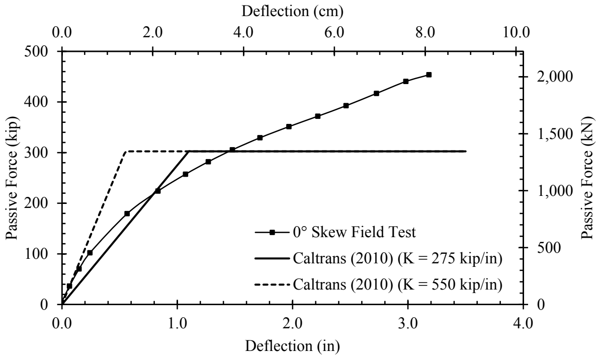
Figure 5.1: Comparison of Soil Stiffness Specified by Caltrans (2010).
