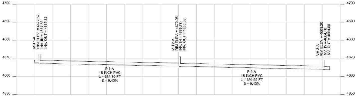
Figure 2-1: Reach 1 Dimensions
