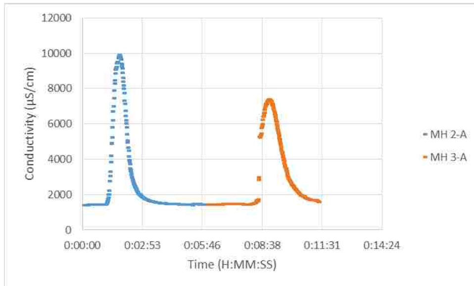
Figure 3-1: Observed Conductivity, Reach 1
