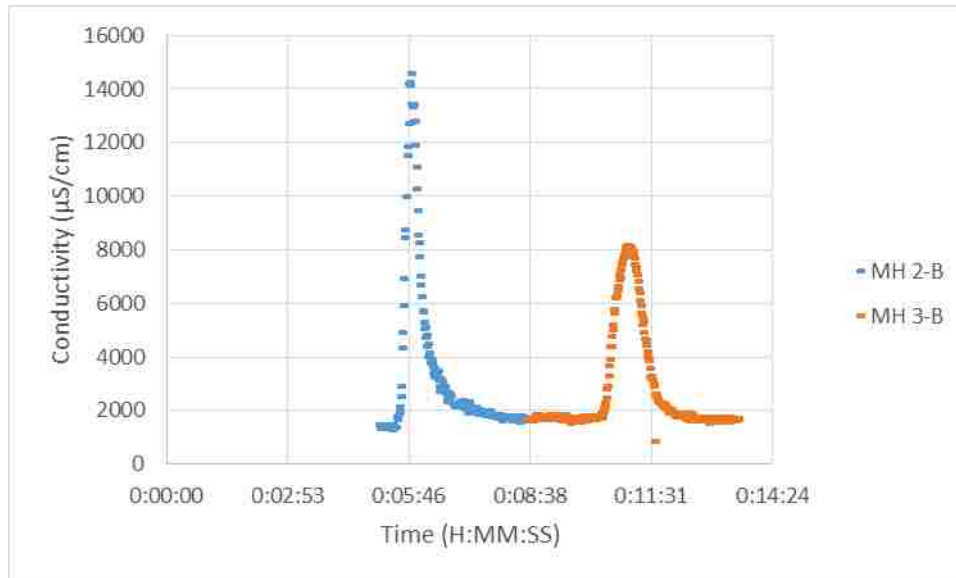
Figure 3-4: Observed Conductivity, Reach 2
