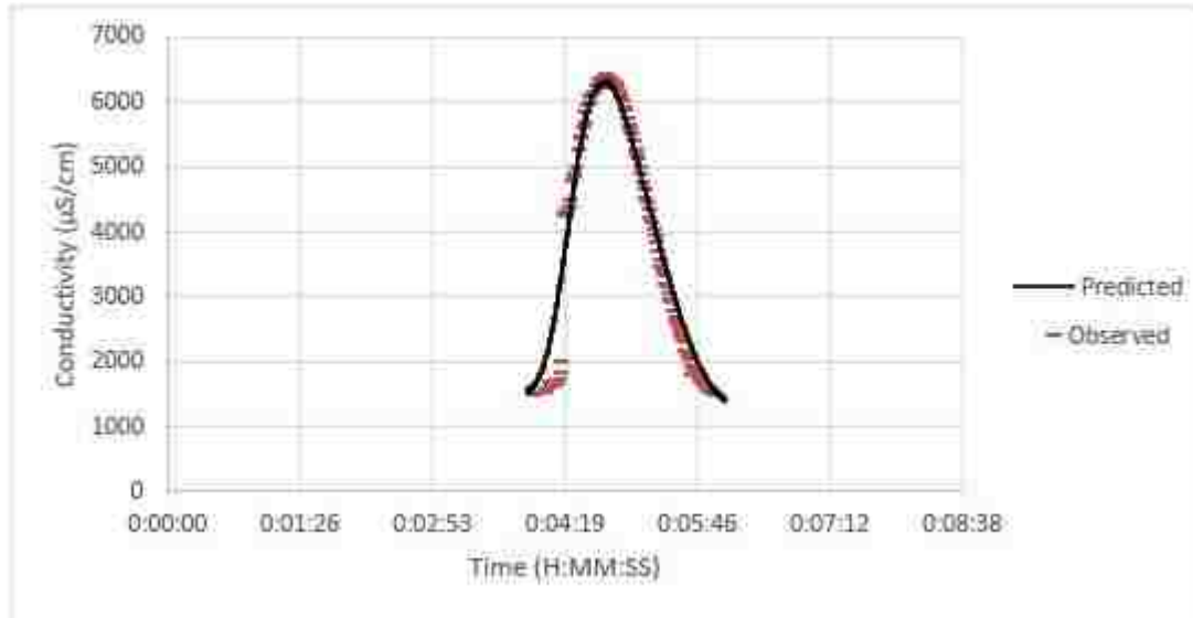
Figure 3-5: Predicted Data vs Observed
