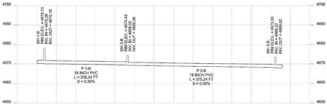
Figure 2-2: Reach 2 Dimensions
