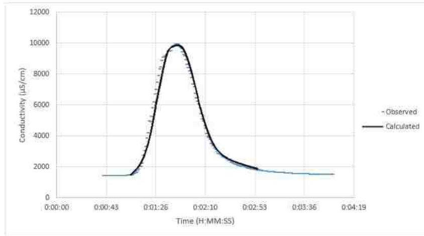
Figure 3-3: Observed vs. Calculated Conductivity
