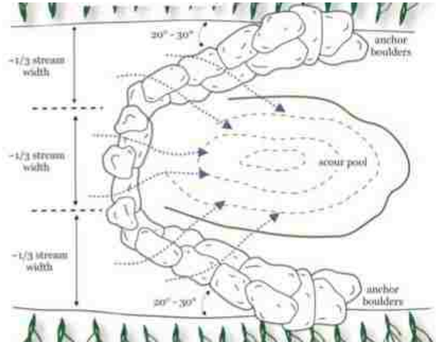
Figure 2-8: Cross-Vane (Sotiropoulos, 2013).
