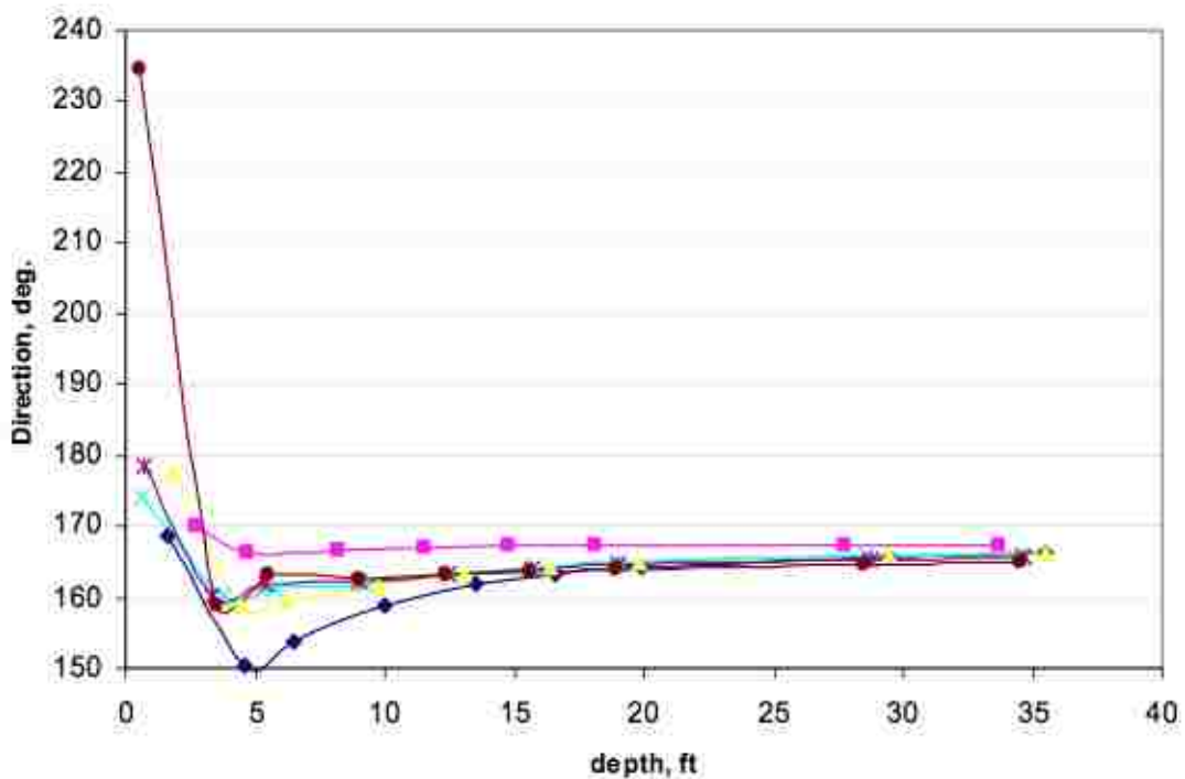
Figure 4-1: Cross-Vane Effective Depth from Change in Flow Direction (Dahle, 2008).
