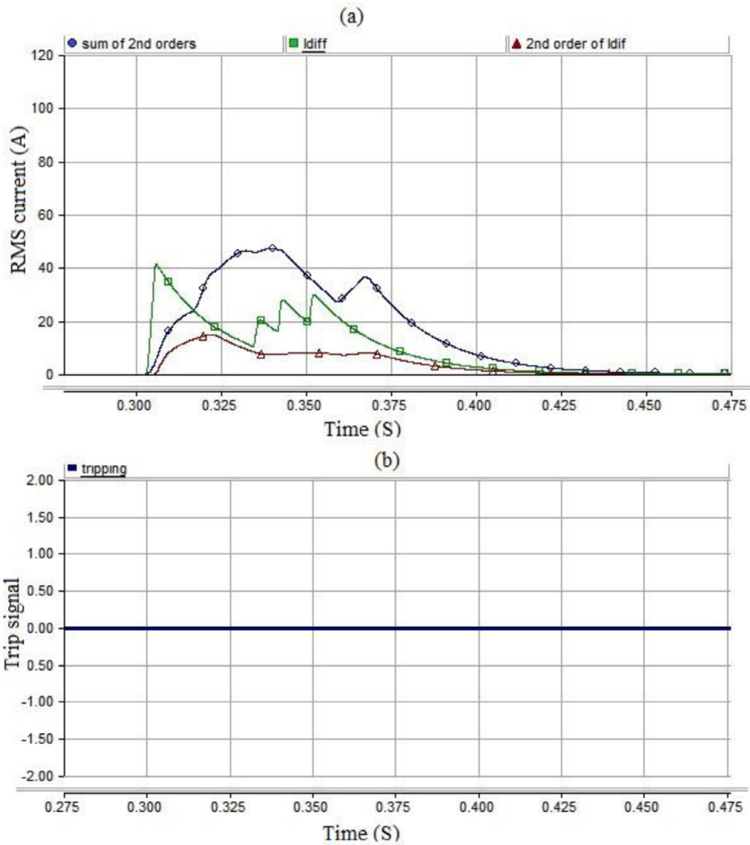
Figure 13 (a) RMS currents; (b) trip signal during external fault, with low fault resistance and saturated CTs.
