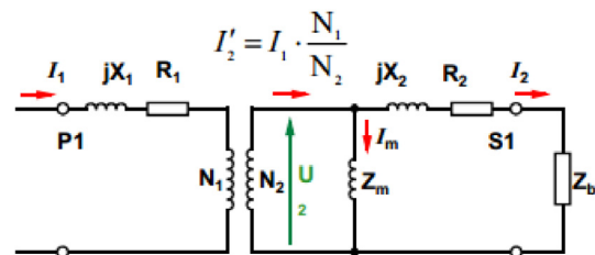
Figure 7 Equivalent circuit of current transformer.
