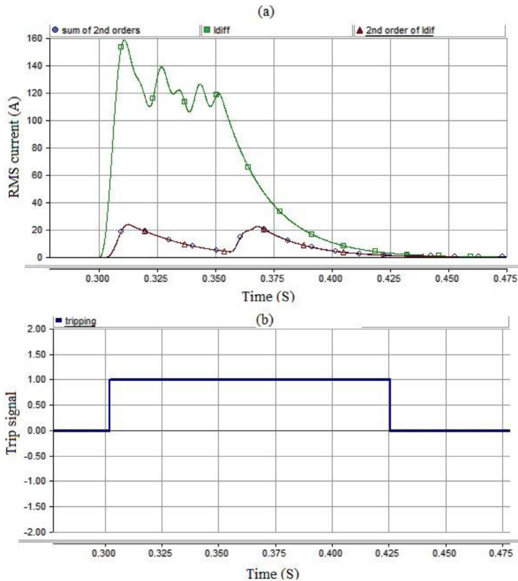
Figure 9 (a) RMS currents; (b) trip signal during internal fault with low fault resistance and unsaturated CTs.
