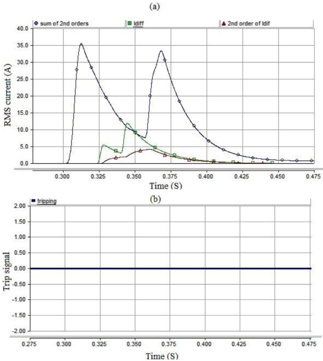
Figure 10 (a) RMS currents; (b) trip signal during external fault, with low fault resistance and unsaturated CTs.
