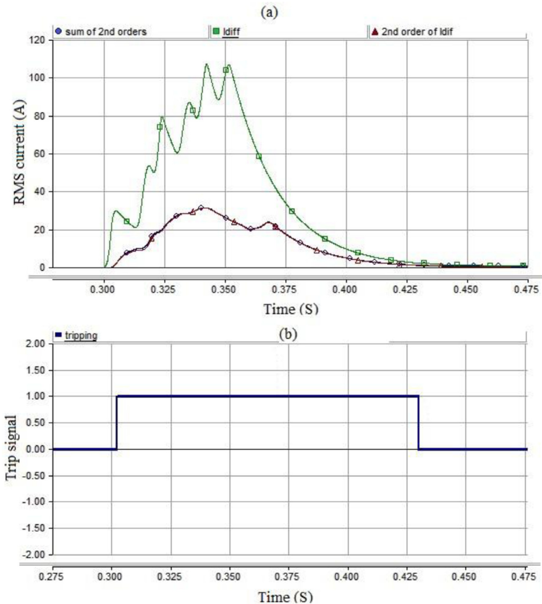
Figure 12 (a) RMS currents; (b) trip signal, during internal fault, with low fault resistance and saturated CTs.
