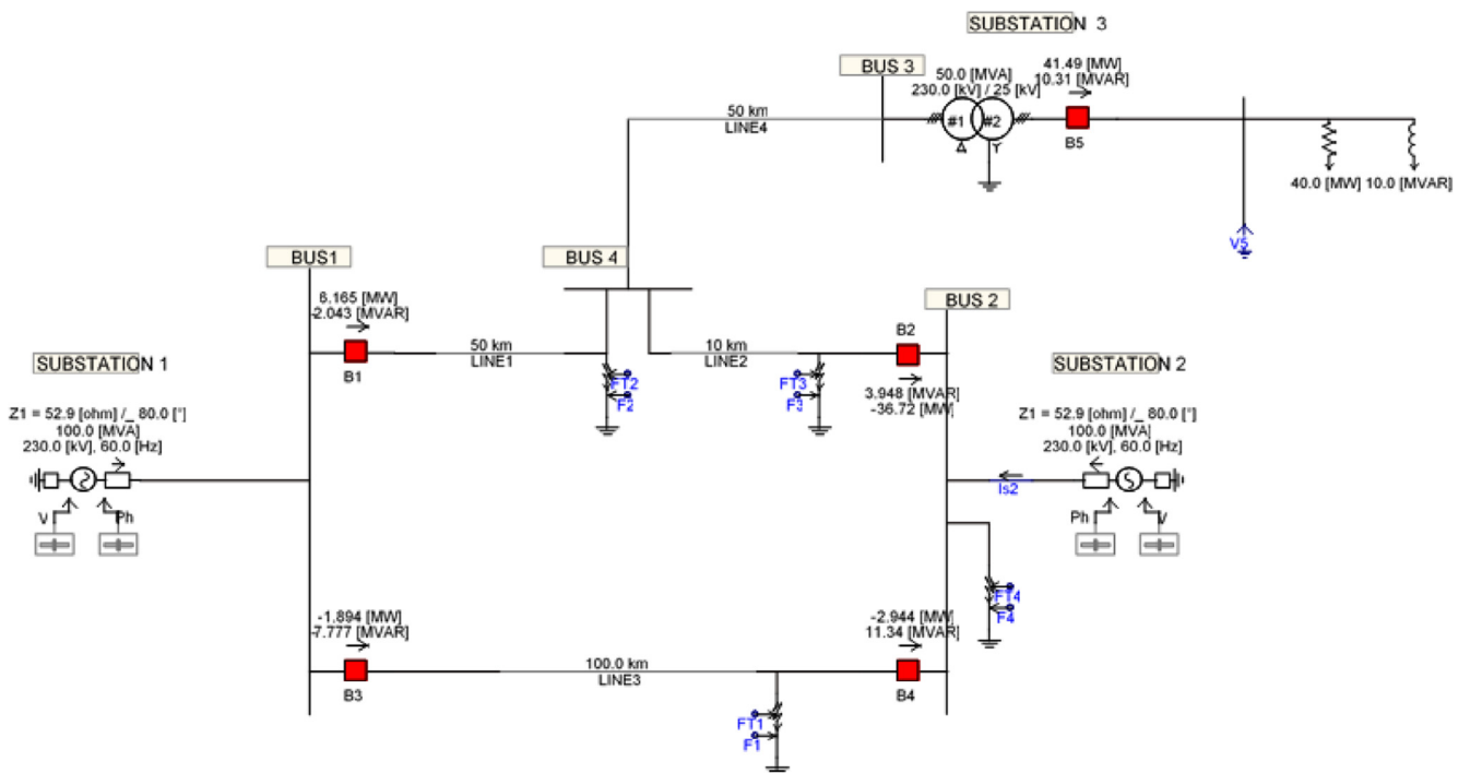
Figure 5 Single-line diagram of power system case study.
