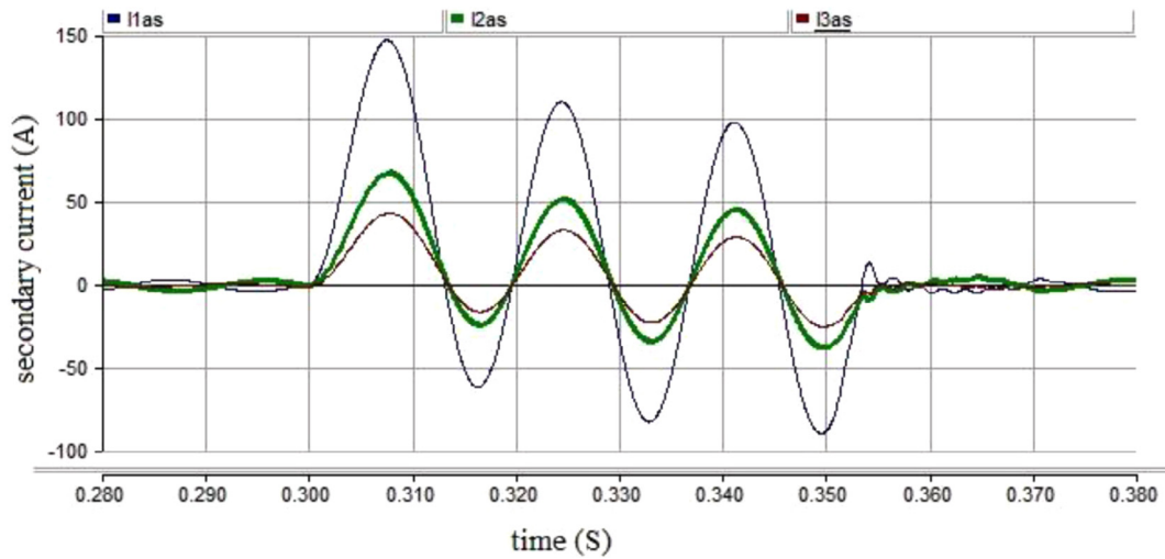
Figure 8 Secondary currents during internal fault (burden impedance 0.5 \Omega without remnant flux).
