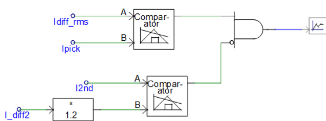
Figure 6 Simulation of proposed scheme.
