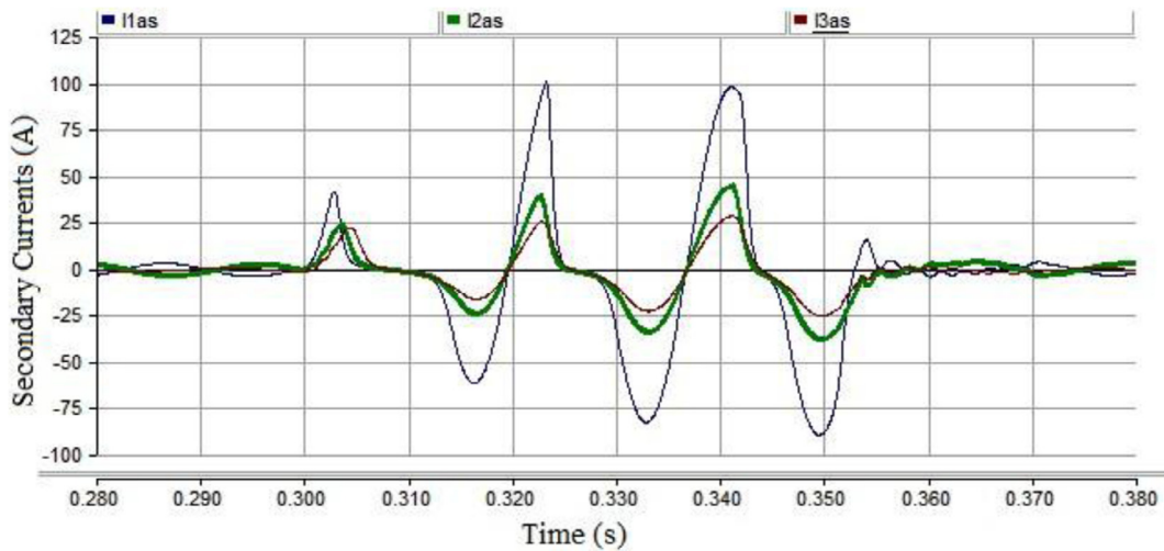
Figure 11 Saturated secondary currents during internal fault (burden impedance 5 \Omega and remnant flux 1.5 Tesla).
