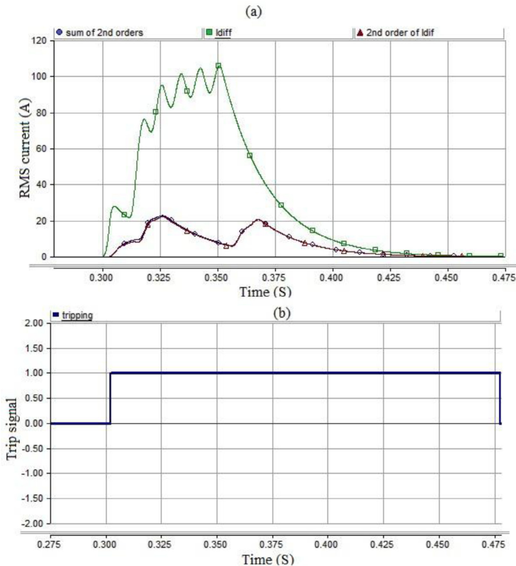
Figure 14 (a) RMS currents; (b) trip signal during internal fault, with high fault resistance and saturated CTs.
