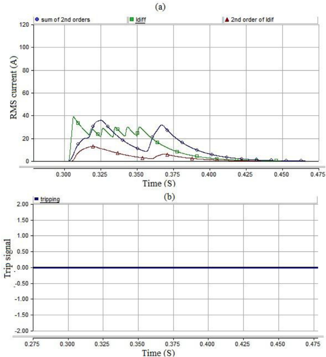
Figure 15 (a) RMS currents; (b) trip signal during external fault, with high fault resistance and saturated CTs.
