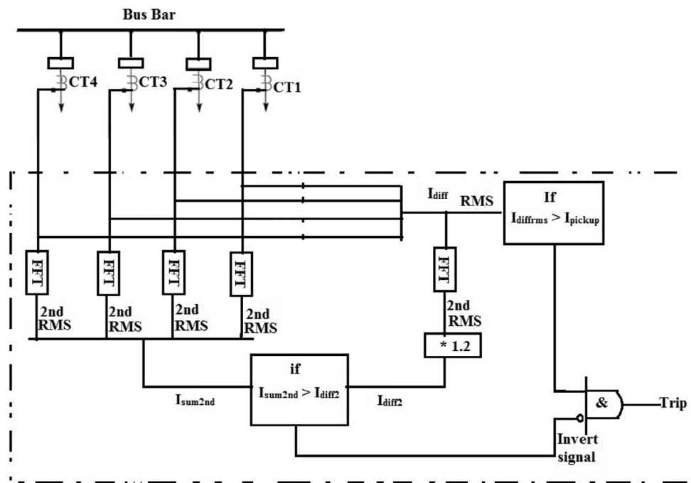
Figure 4 Block diagram of proposed algorithm.
