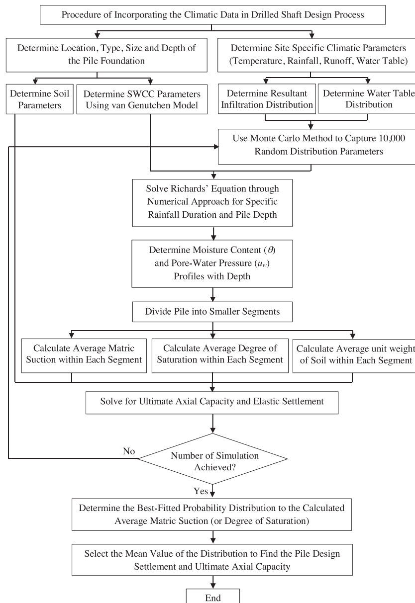
Fig. 4. Flowchart of proposed procedure for incorporating the hydrological data in geotechnical design of drilled shaft.
