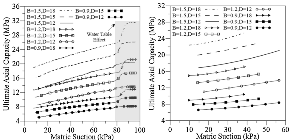
Fig. 12. Predicted variation of ultimate axial capacity with matric suction after 3-day continuous rainfall (Left: Riverside, CA and Right: Salt Lake City, UT).
