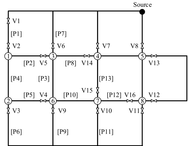
Fig. 4. A small WDN.
