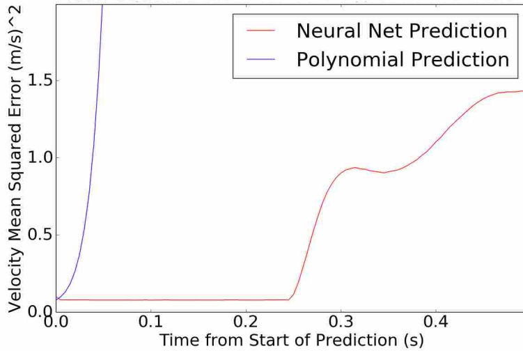
Figure 3.15: Mean squared error of the neural network prediction and the polynomial prediction for 0.5 seconds using data with added noise similar to the noise from the encoders on our robot. While both predictions are degraded, the polynomial prediction becomes useless. An 8th order polynomial does not extrapolate well when there is noise. Notice that the scale of this graph is different than the other MSE graphs. The polynomial prediction MSE reaches 1,000,000 (m/s) 2 by 0.5 seconds.
