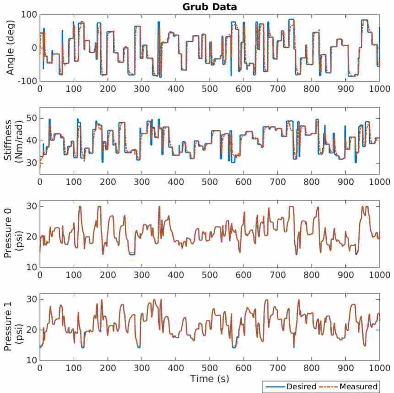
Figure 4.4: Data collected from the grub used to train the neural net.
