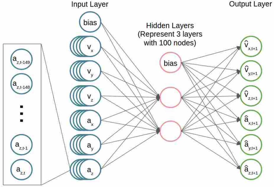
Figure 3.1: Symbolic representation of the neural network. a represents acceleration and v represents velocity. The subscripts, x , y , and z , represent the orthogonal axes. t + 1 represents one time step into the future.
