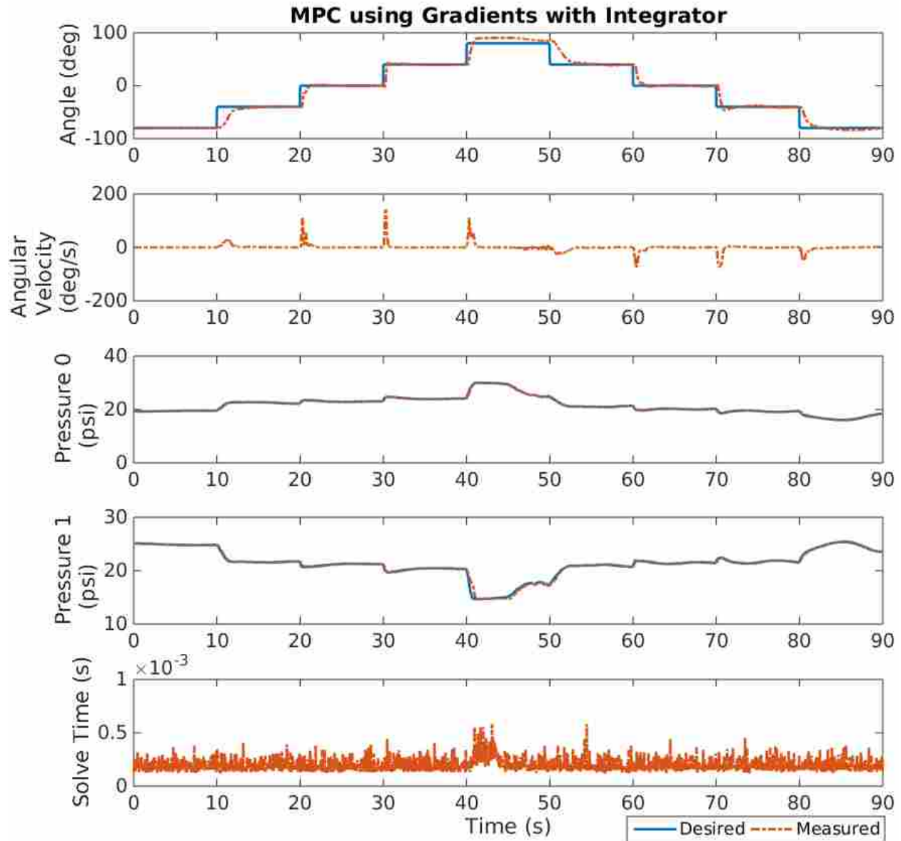
Figure 4.6: MPC with the gradients from the neural net at 30 Hz using an integrator
