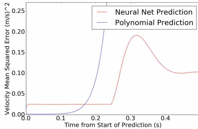
Figure 3.13: Mean squared error of the neural network prediction and the polynomial prediction for 0.5 seconds using the training data set. The neural net is specifically trained for the first 0.25 seconds which are flat, after which the performance of the neural network significantly degrades. The polynomial prediction MSE reaches 1500 \text{ (m/s)}^2 by 0.5 seconds. Interestingly, the neural net prediction increases and then decreases after the first 50 steps. It is difficult to know why neural nets behave in certain ways and this warrants further investigation.
