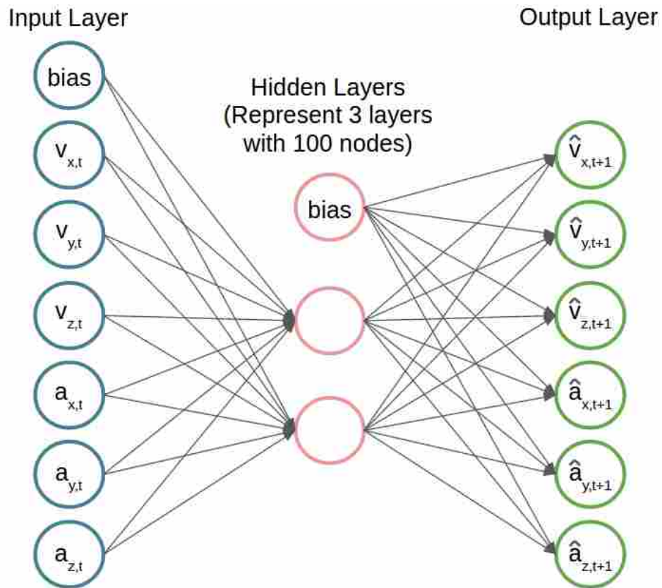
Figure 1.2: Symbolic representation of a neural network. The hat represents a prediction, and t + 1 indicates that it is one time step into the future.
