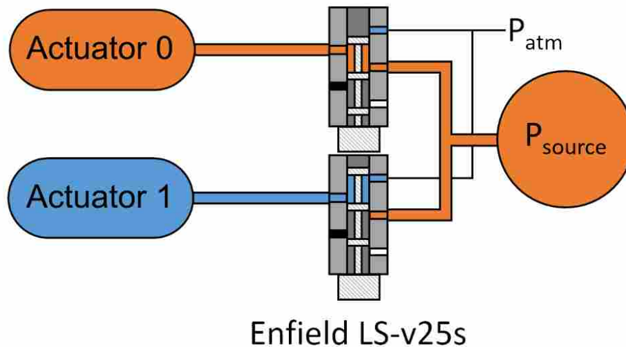
Figure 4.2: Representative figure of valve and actuator bladder configuration.
