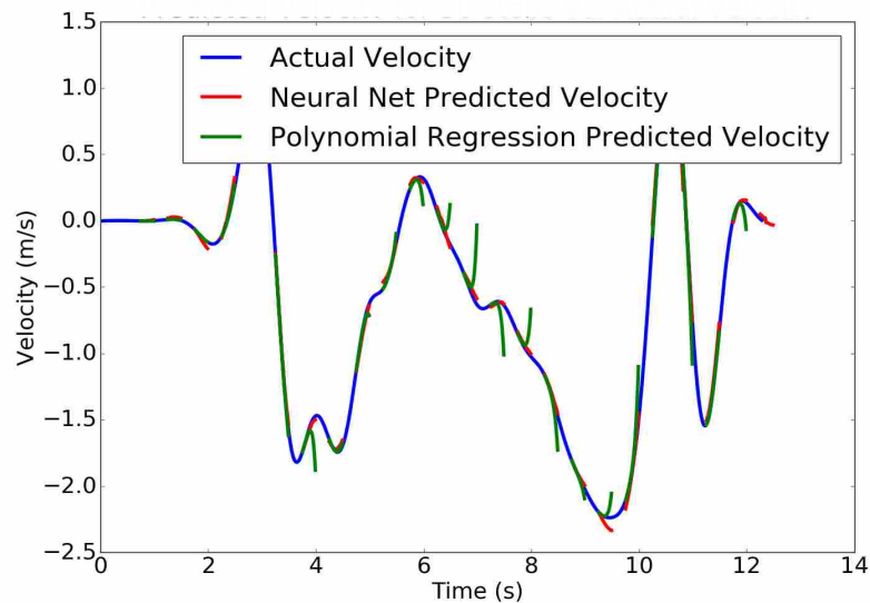
Figure 3.10: Predictions using the neural net and a polynomial estimator for velocity in one task. While both are accurate in most cases, in several cases the polynomial prediction is far from the actual data.
