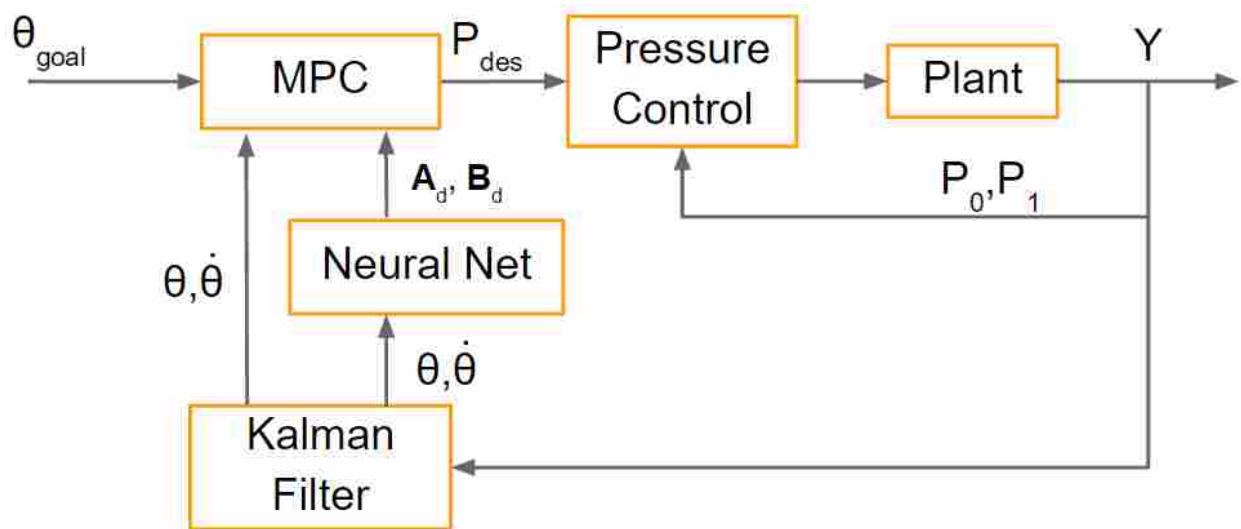
Figure 4.3: MPC flow chart showing the neural net linearization and the low level PID pressure controller
