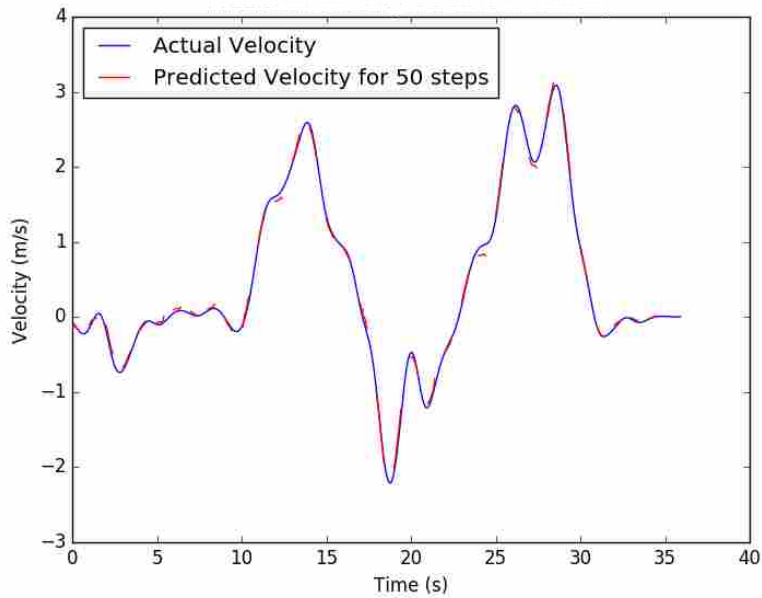
Figure 3.4: Comparison of the velocity prediction to actual future data in the longitudinal direction while a human dyad moves the table. The directions are body-fixed to the table frame. Each red line is a separate 50 step prediction using the 150 steps before it.
