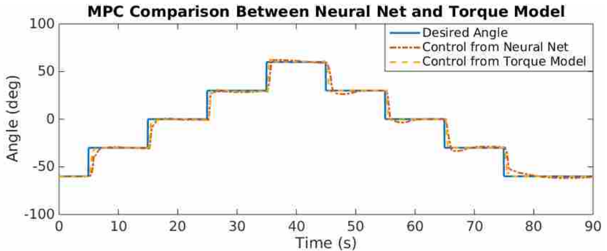
Figure 4.8: This shows how MPC using the neural net gradients compares to MPC using first principles models in past work.
