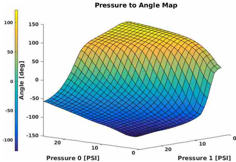
Figure 4.7: The angle of the soft robot joint based on the pressures in the bladders.
