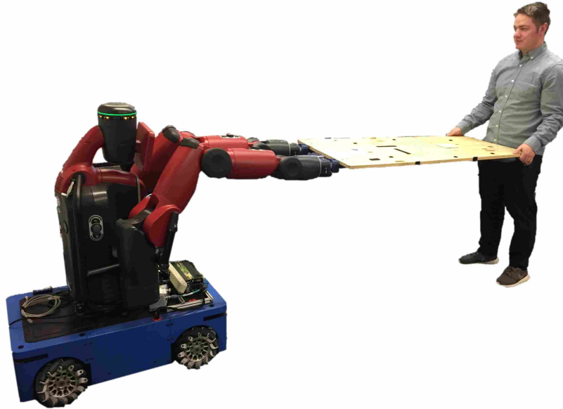
Figure 3.3: Rethink Robotics Baxter robot mounted on HStar Technologies AMP-1 holonomic base carrying the table with a person.
