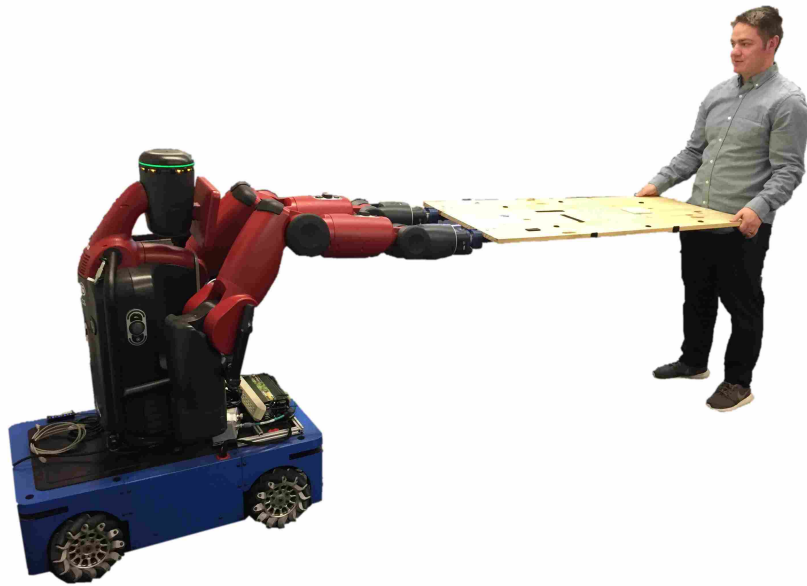
Figure 1.4: Rethink Robotics Baxter robot mounted on HStar Technologies AMP-1 holonomic base carrying the table with a person.
