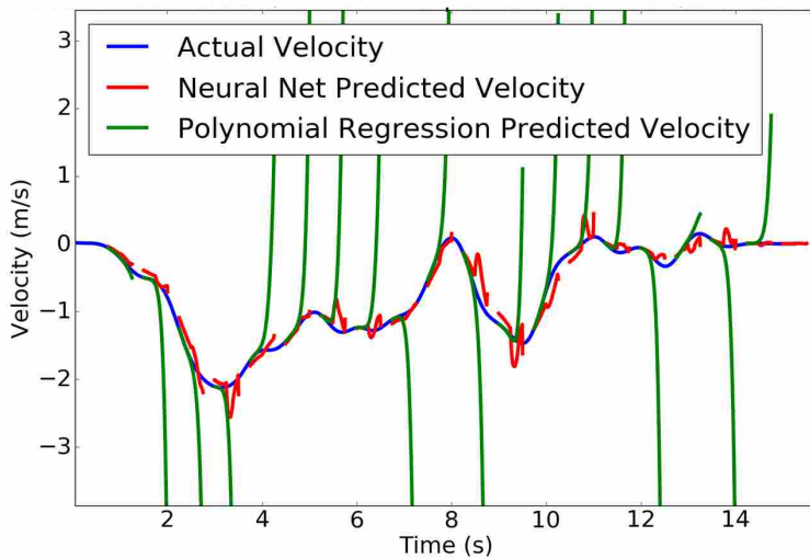
Figure 3.12: Comparison of the velocity prediction to actual future data in the x direction while a human dyad moves the table. Each red line is a separate 100 step prediction using the 150 steps before it. The green line is the polynomial prediction. This shows how the quality of the neural net prediction decreases significantly after 50 steps as expected.
