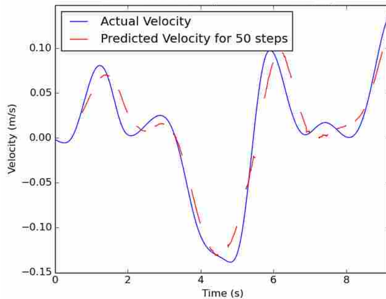
Figure 3.20: Horizontal direction comparison.
