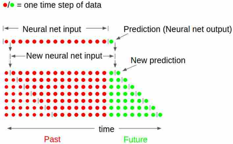
Figure 3.2: Iterated prediction allows us to predict more than one step into the future.
