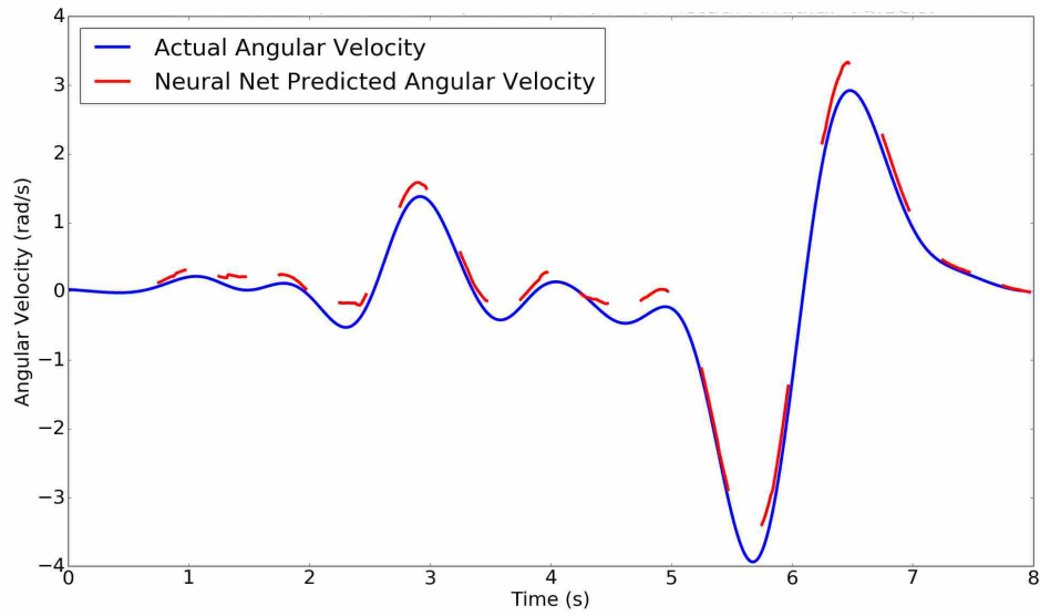
Figure 3.8: Pitch angular velocity prediction versus actual angular velocity.
