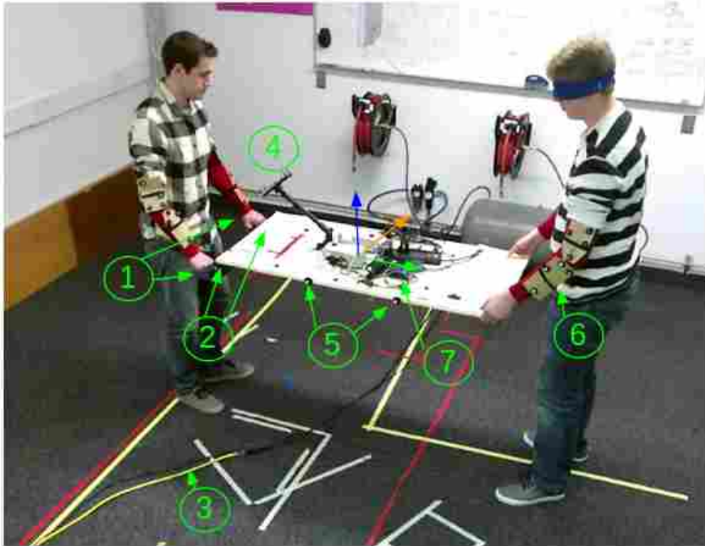
Figure 2.1: A dyad performing a task along with a description of the setup. The leader is on the left holding the handles. The follower is on the right with a blindfold which they wore for half of the tasks. The numbers describe the following: 1. Handles 2. Force/torque sensors 3. Power and ethernet cables 4. iPad with instructions 5. Motion capture IR reflective markers 6. Motion capture sleeves 7. Router, force sensor boxes, and power strip. Green is the longitudinal axis, blue is the vertical axis, and orange is the horizontal axis.
