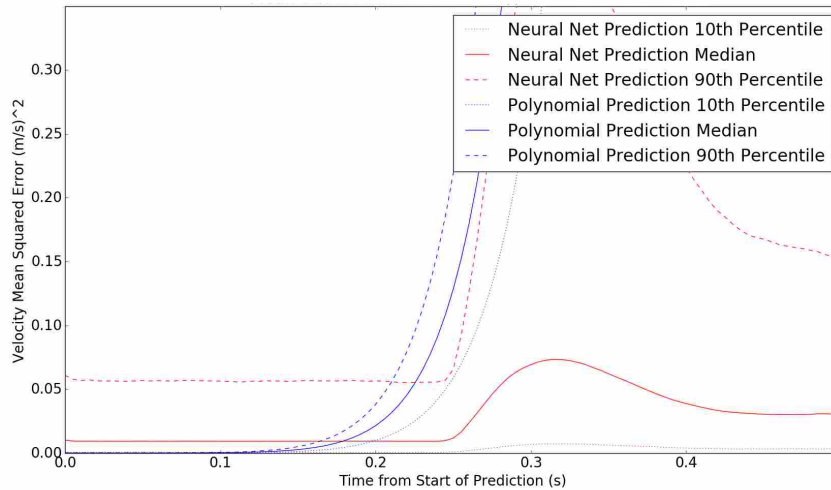
Figure 3.16: 10th percentile, median, and 90th percentile squared error plots for the neural net prediction in red and the polynomial prediction in blue.
