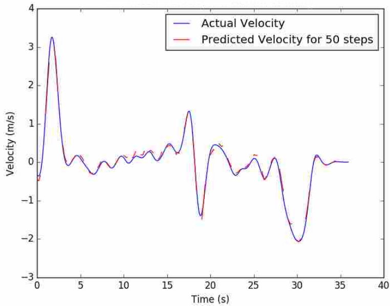
Figure 3.6: Vertical direction prediction versus actual velocity.
