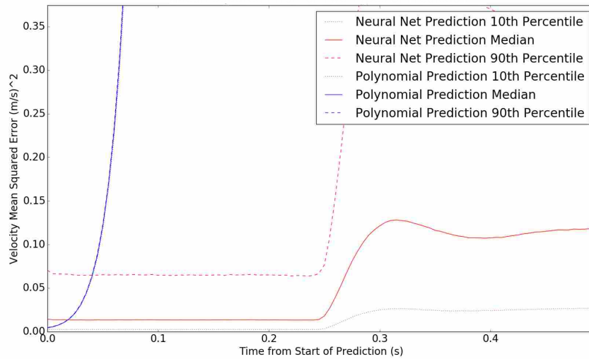
Figure 3.18: 10th percentile, median, and 90th percentile squared error plots for the neural net prediction in red and the polynomial prediction in blue when noise is added to the data. The polynomial prediction lines all overlap. Notice that the values for the neural net prediction are comparable to the ones in Figure 3.16.
