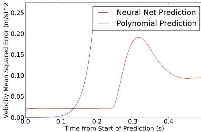
Figure 3.14: Mean squared error of the neural network prediction and the polynomial prediction for 0.5 seconds using the validation data set. There is very little difference between the prediction on the validation and training data sets. The polynomial prediction MSE reaches 1500 \text{ (m/s)}^2 by 0.5 seconds.
