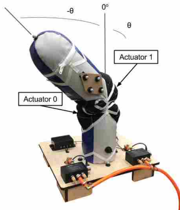
Figure 4.1: This is a single degree of freedom soft robot platform that we call a grub.
