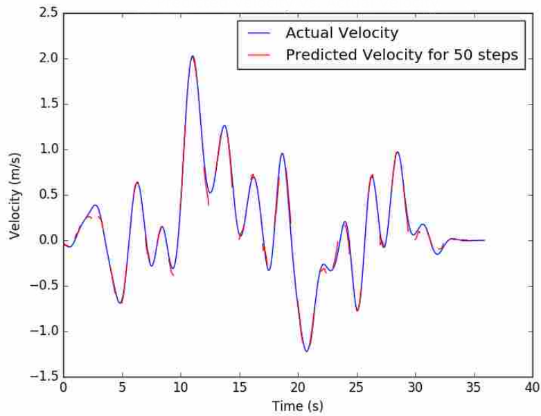
Figure 3.5: Horizontal direction prediction versus actual velocity.
