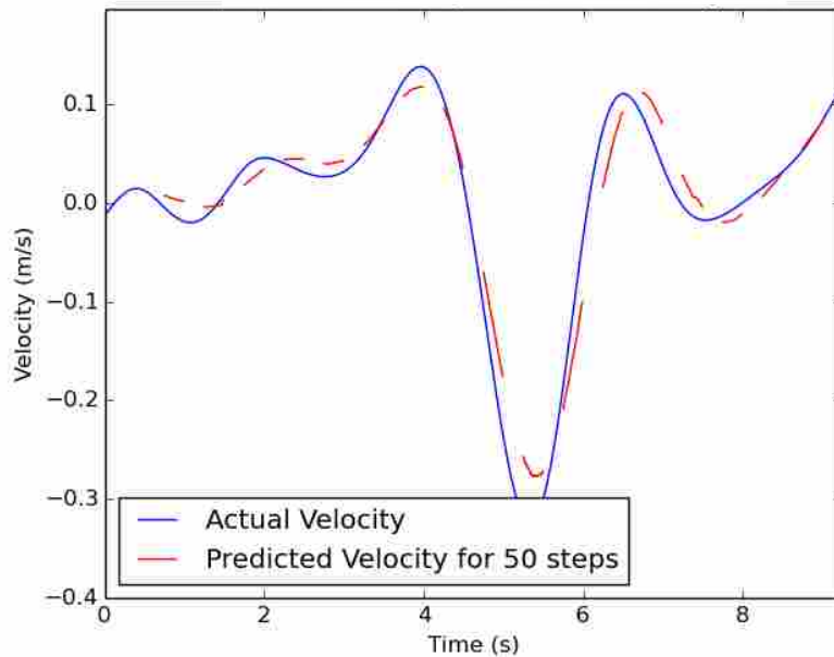
Figure 3.19: Comparison of velocity prediction to actual future data in the longitudinal direction while a human-robot dyad moves the table. Each red line is a separate 50 step prediction using the 150 steps of real data before it.
