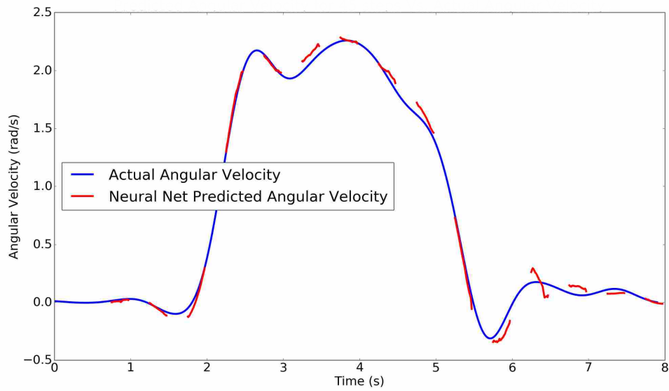
Figure 3.9: Yaw angular velocity prediction versus actual angular velocity.
