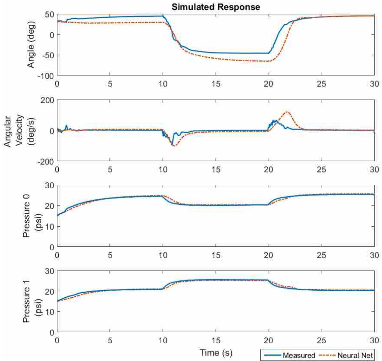
Figure 4.5: Neural net predictions compared to actual data.
