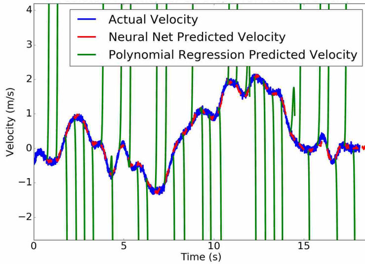
Figure 3.11: Predictions using the neural net and a polynomial estimator for velocity in one task where white noise has been added. The noise causes the polynomial prediction to go completely unstable while the neural network prediction is fairly robust.
