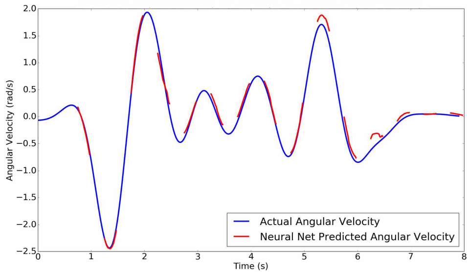
Figure 3.7: Comparison of roll angular velocity prediction to actual future data while a human dyad moves the table. These are in the table frame. Each red line is a separate 50 step prediction using the 150 steps before it.
