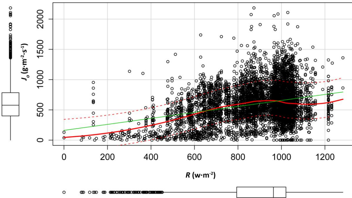
Figure 5. Sap-flux density ( J_o ) as a function of incoming shortwave radiation( R ). Based on average daily for all trees at all sites. Green: line of best fit. Red: fitted parabolic line. Dotted red: average range of data.
