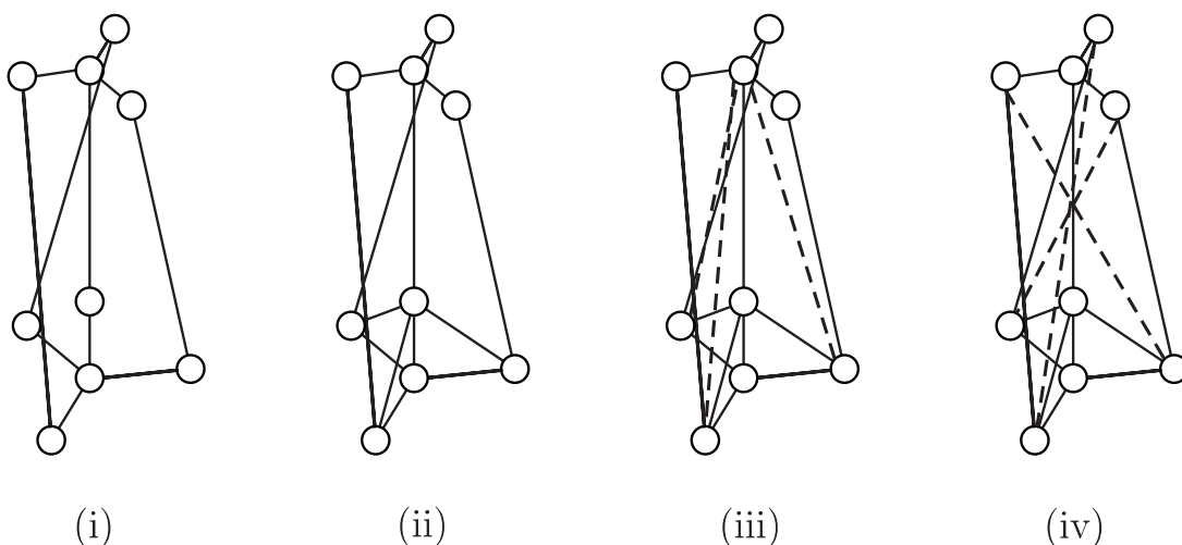
Figure 5.7: Bracing options for the IBGS: (i) no bracing, (ii) inclined bracing, (iii) additional bracing option A and (iv) additional bracing option B.
