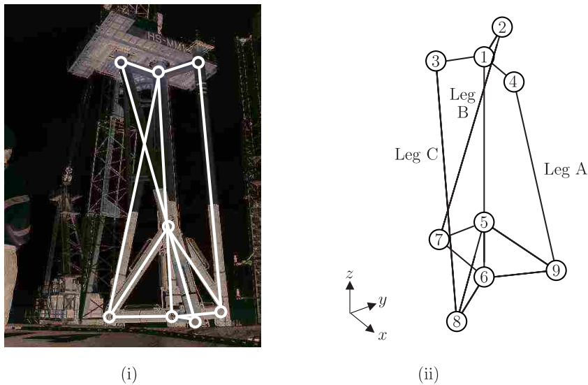
Figure 5.2: (i) Discretisation of the IBGS using linear beam elements [16] and (ii) the node numbering system used.
