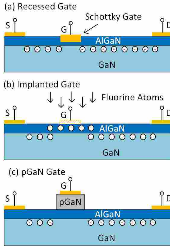
Figure 1.4: Enhancement-mode structures for AlGaIn/GaN devices showing (a) recessed gate, (b) implanted gate, and (c) pGaIn gate technologies.
