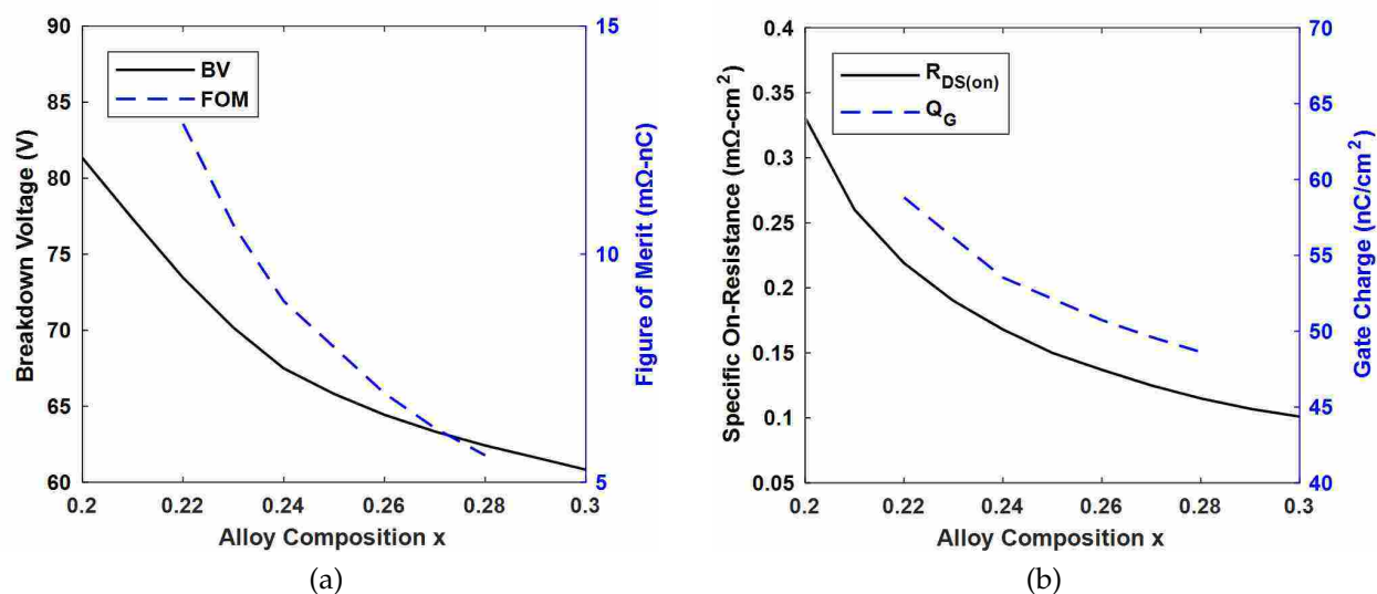
Figure 4.8: Simulation results for x_{AlGaIn} presenting (a) breakdown voltage and FOM trends as well as (b) on-state resistance and gate charge trends.
