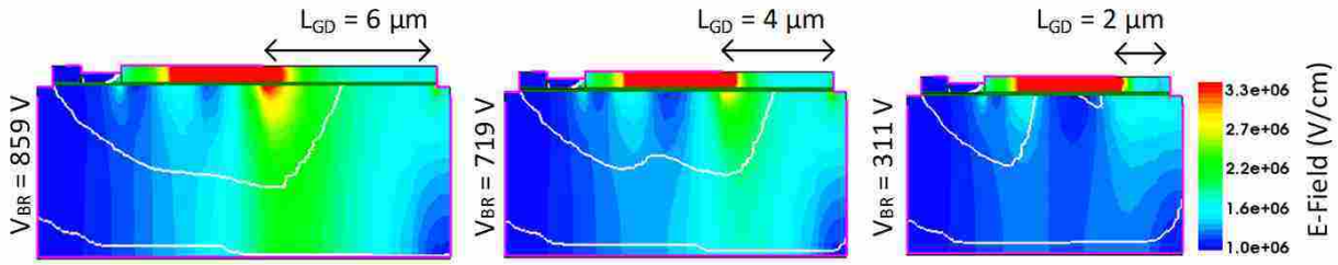
Figure 2.4: Electric field profiles as L_{GD} is reduced.
