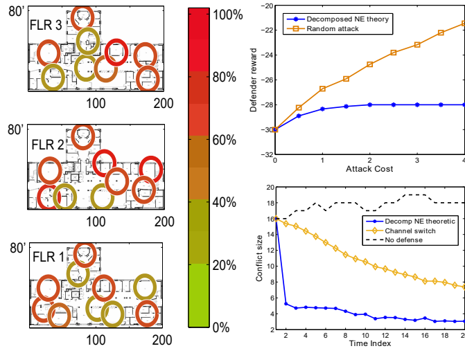
Figure 3.7: (Left) Mixed strategy for power assignment of 28 nodes in 3-floor building, (Right) The top plot shows the defender reward vs the attack cost, and the bottom plot displays the time evolution of the conflicts with and without defense.
