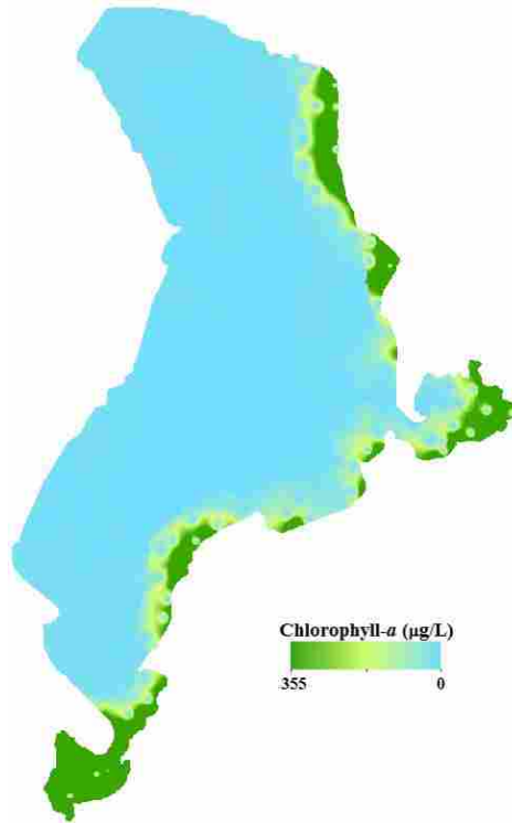
Figure 4-2: Chlorophyll- a mapping over Utah Lake for spring 2005
