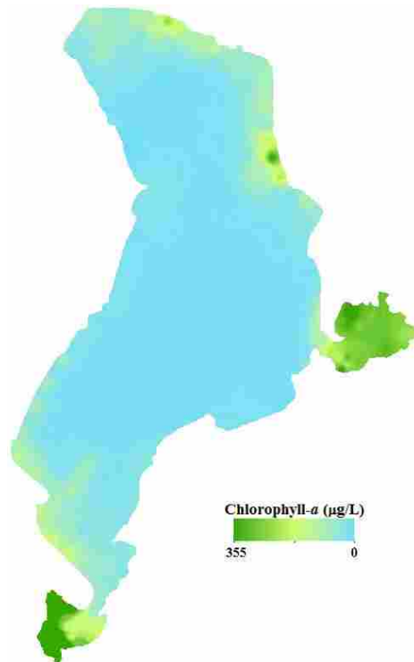
Figure 4-13: Chlorophyll- a mapping over Utah Lake for summer 2008
