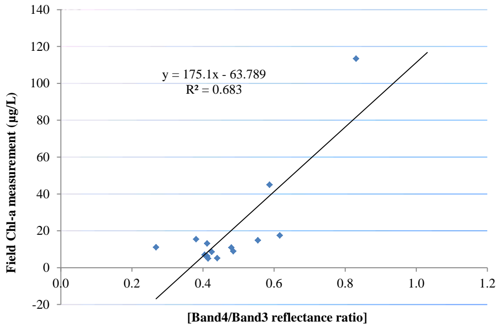
Figure A-5: Field measured chlorophyll- a vs. Band 4/Band 3 (linear trendline)
