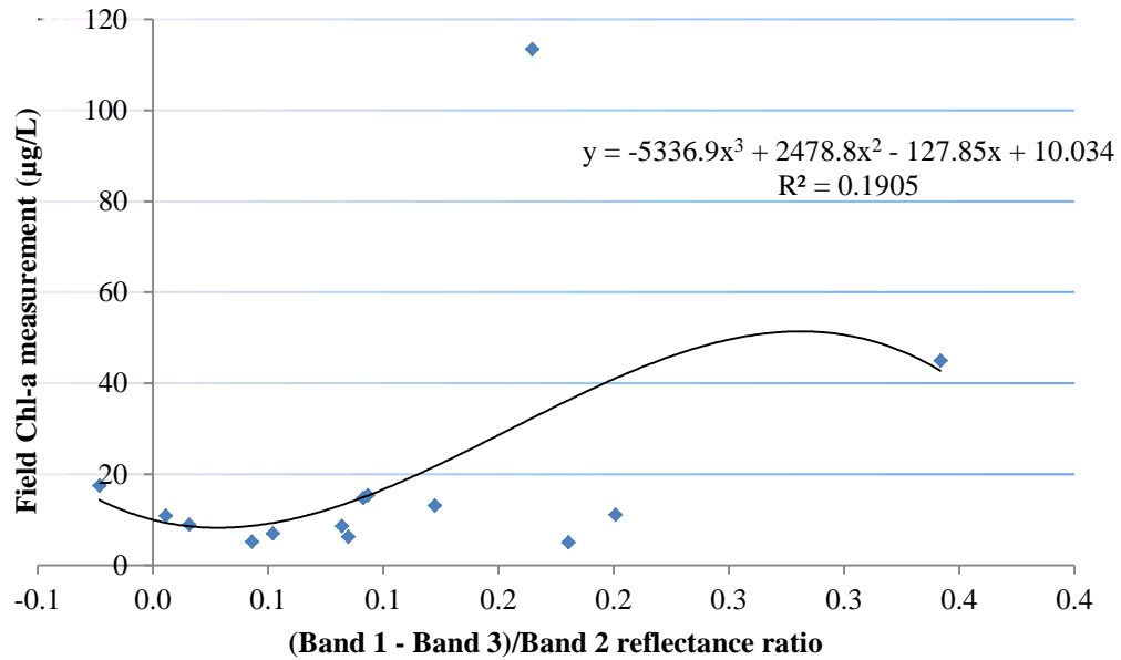
Figure A-8: Field measured chlorophyll- a vs. (Band 1 – Band 3)/Band 2 (polynomial trendline)
