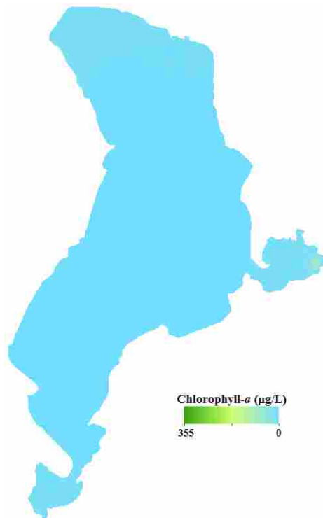
Figure 4-3: Chlorophyll- a mapping over Utah Lake for spring 2006
