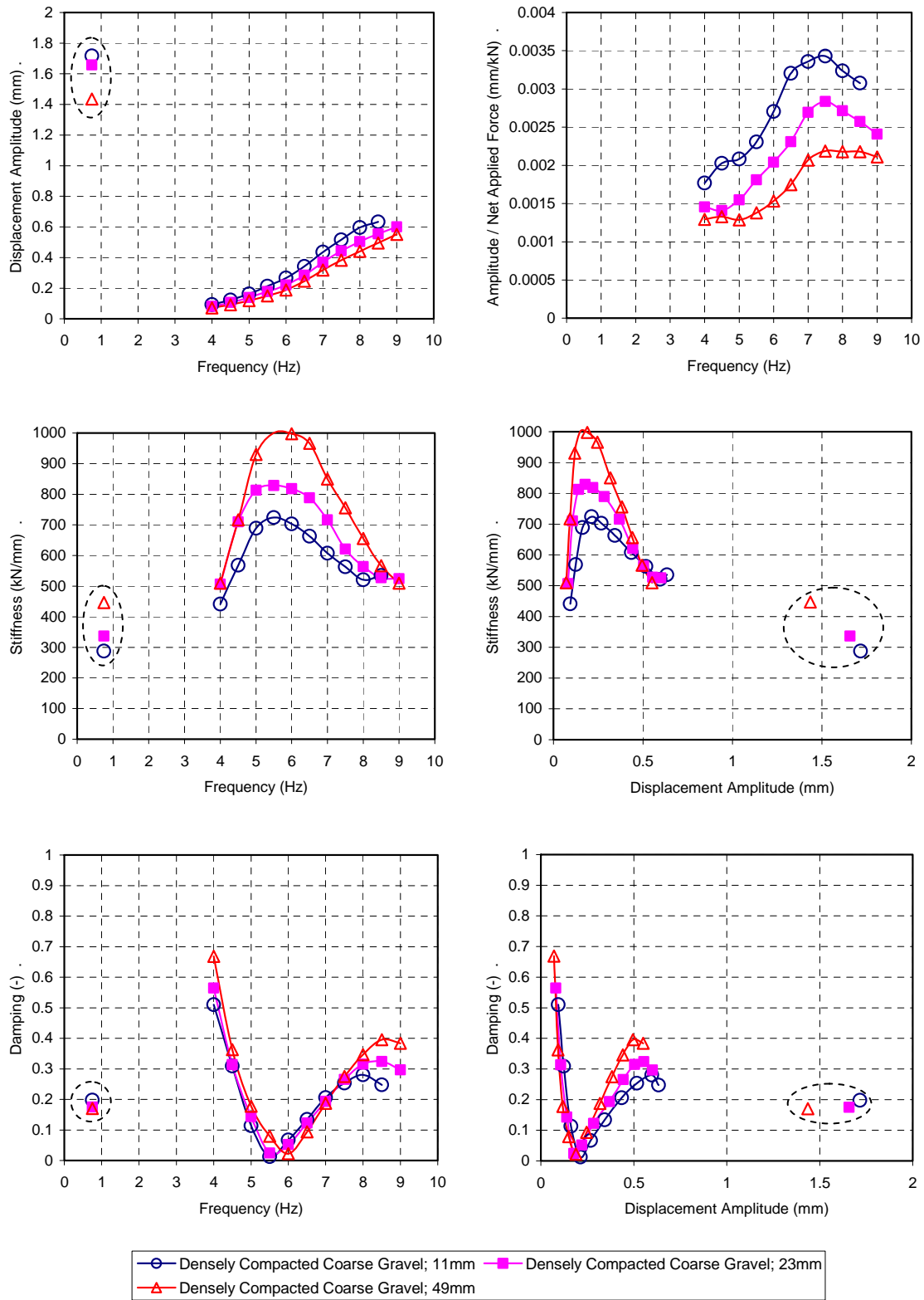
Figure 8-7 Summary of response to dynamic shaker loadings for pile cap with densely compacted coarse gravel backfill
