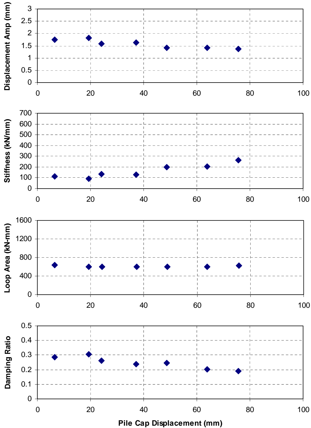
Figure 7-6 Summary of response to cyclic actuator loadings for pile cap with loosely compacted fine gravel backfill
