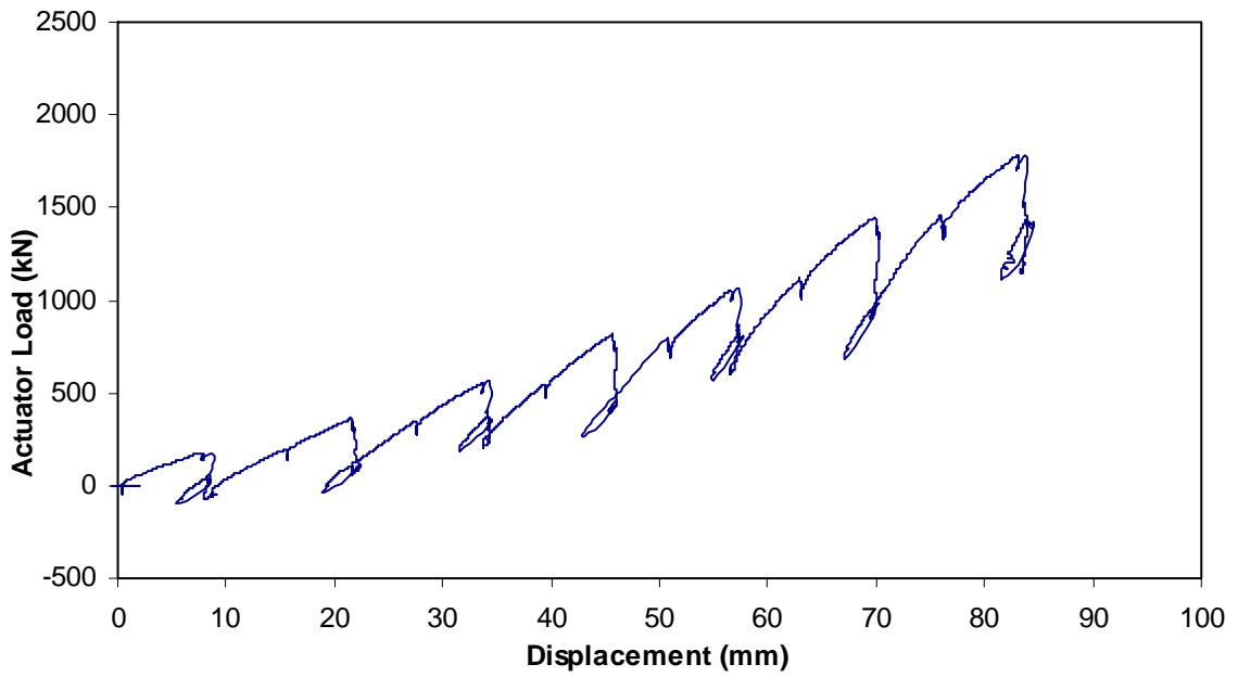
Figure 4-1 Load versus displacement relationship for pile cap with no backfill materials present (baseline test)
