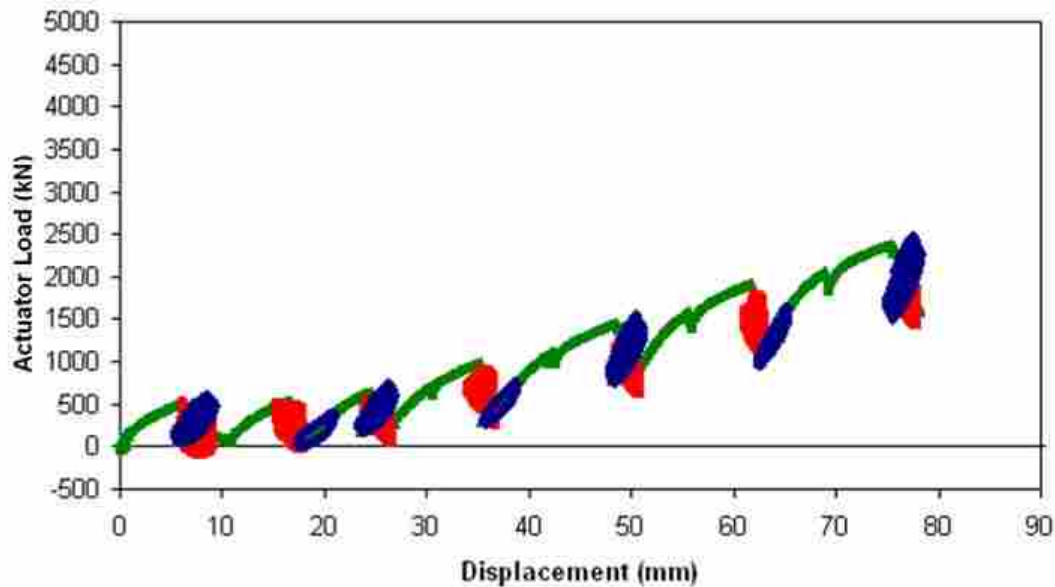
Figure 7-1 Actuator load versus pile cap displacement with loosely compacted fine gravel backfill (Test 7; June 6, 2007)
