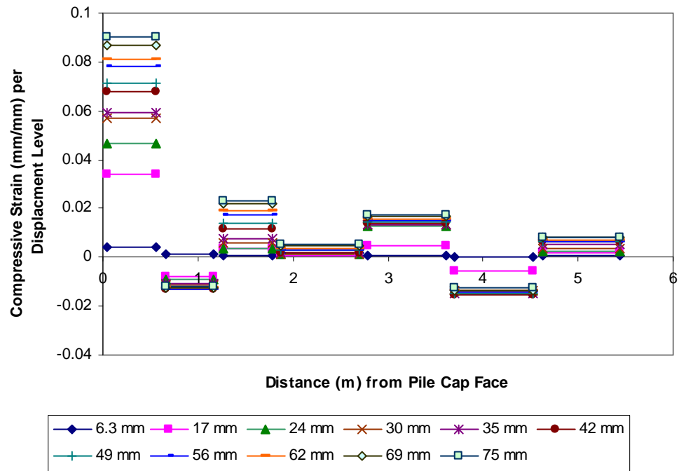
Figure 7-13 Strain per displacement level for loosely compacted fine gravel backfill
