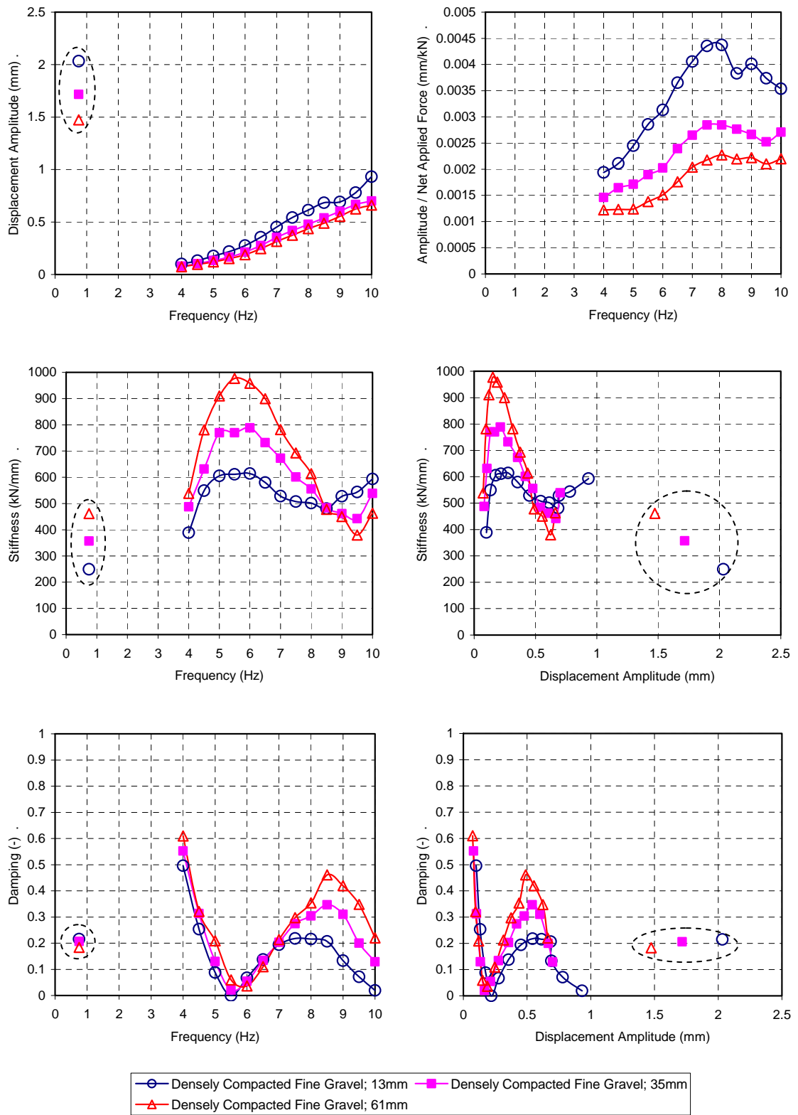
Figure 6-7 Summary of response to dynamic shaker loadings for pile cap with densely compacted fine gravel backfill
