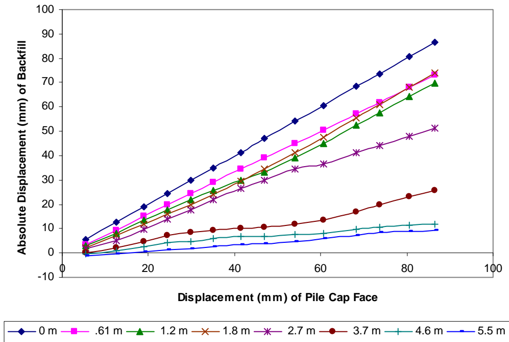
Figure 6-12 Displacement of monitoring points in densely compacted fine gravel backfill
