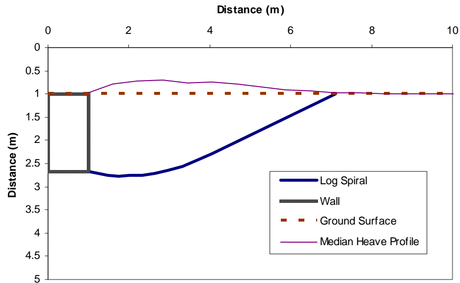
Figure 6-11 Heave profile with best-fit log-spiral failure surface from PYCAP for densely compacted fine gravel backfill
