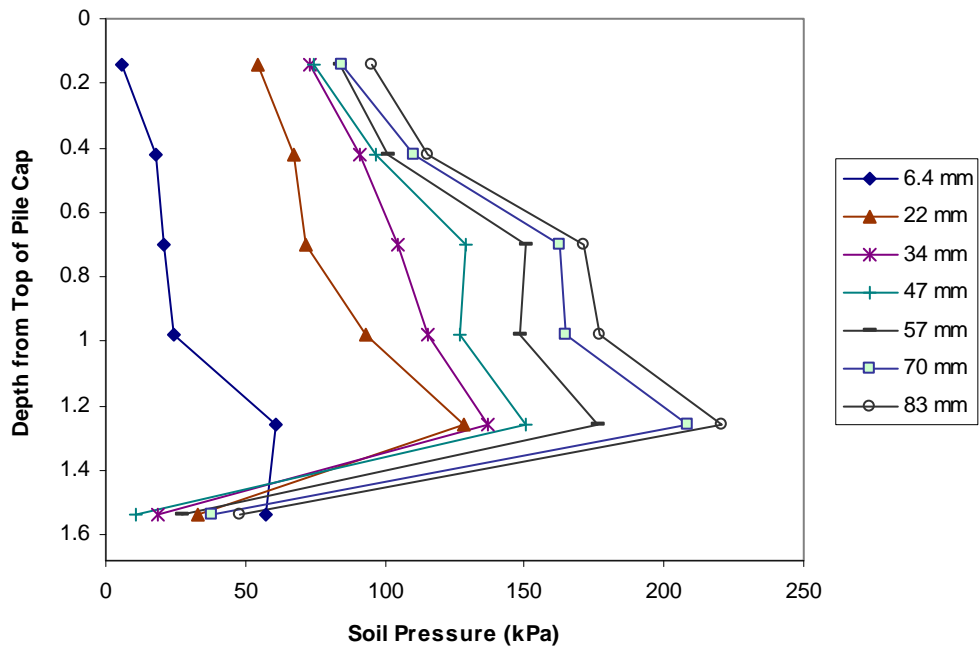
Figure 9-8 Earth pressure distribution as a function of pile cap displacement with loosely compacted coarse gravel
