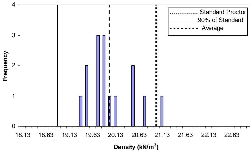
Figure 3-12 Density distribution of loosely compacted coarse gravel backfill
