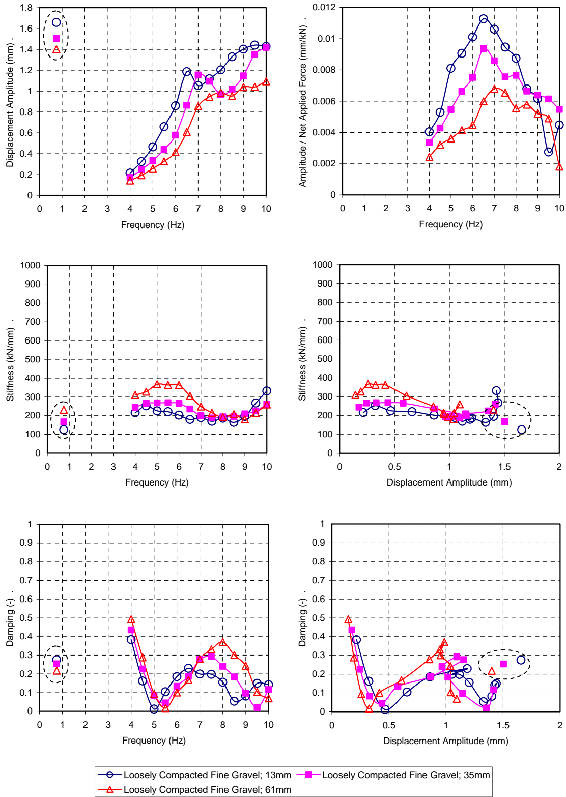
Figure 7-7 Summary of response to dynamic shaker loadings for pile cap with loosely compacted fine gravel backfill
