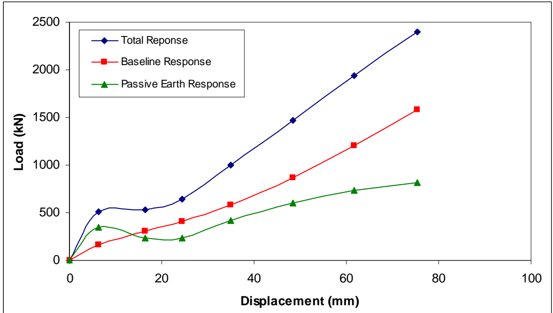
Figure 7-2 Total, baseline and passive earth responses for the pile cap with loosely compacted fine gravel backfill
