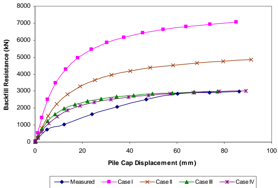
Figure 6-4 Comparison of measured and LSH-based calculated passive resistance for densely compacted fine gravel backfill
