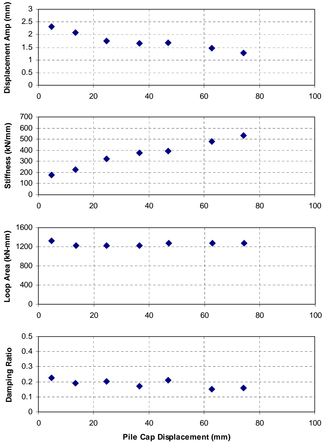
Figure 6-6 Summary of response to cyclic actuator loadings for pile cap with densely compacted fine gravel backfill
