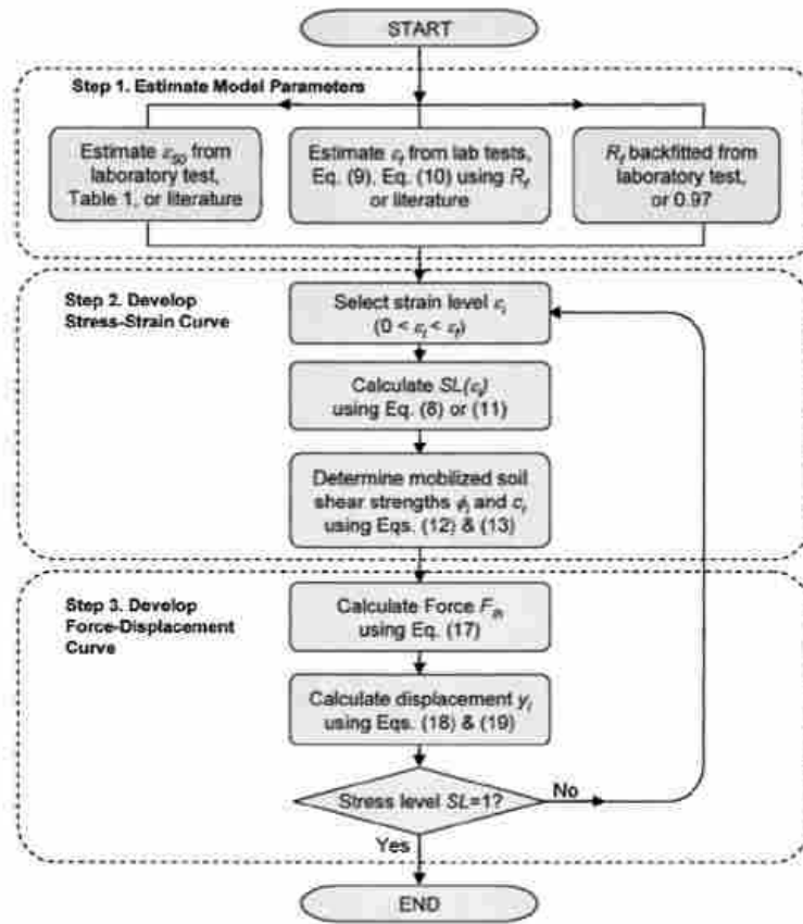
Figure 2-5 Flowchart for the LSH (Shamsabadi et al., 2007) method of predicting lateral passive resistance of an abutment backfill soil
