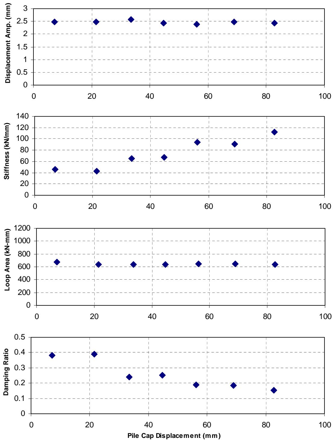
Figure 5-3 Summary of response to cyclic actuator loadings for pile cap without backfill (baseline test)
