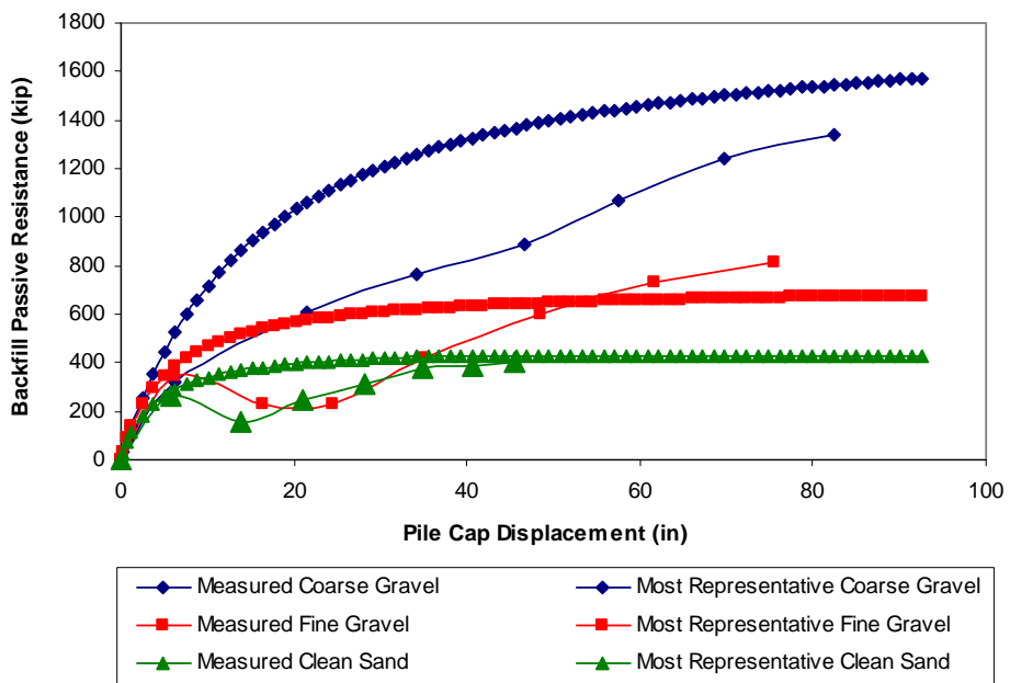
Figure 10-6 Summary of measured versus calculated load-displacement curves for loosely compacted backfill materials using “most-representative” parameters
