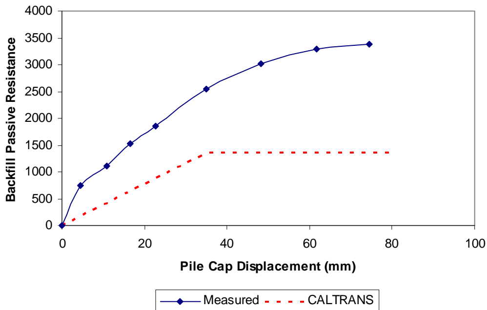
Figure 8-5 Comparison of measured and CALTRANS-based passive resistance for densely compacted coarse gravel backfill
