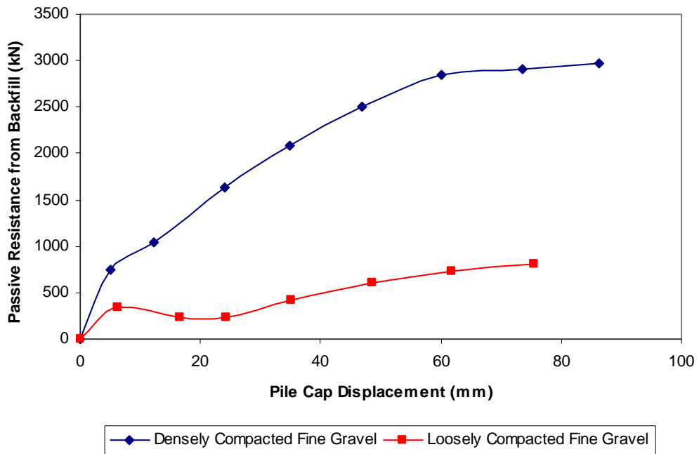
Figure 10-1 Comparison of measured passive earth force-displacement curves for densely and loosely compacted fine gravel backfill
