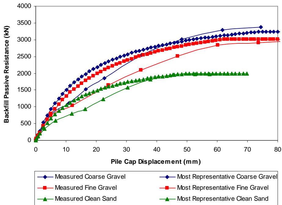
Figure 10-5 Summary of measured versus calculated load-displacement curves for densely compacted backfill materials using “most-representative” parameters
