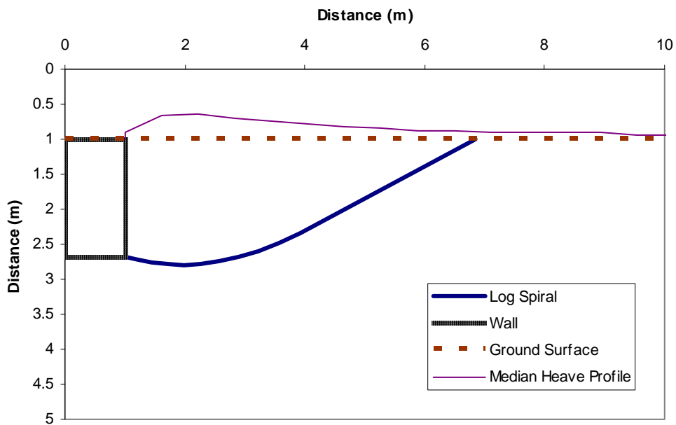
Figure 8-11 Heave profile for densely compacted coarse gravel compared with log-spiral failure surface from PYCAP
