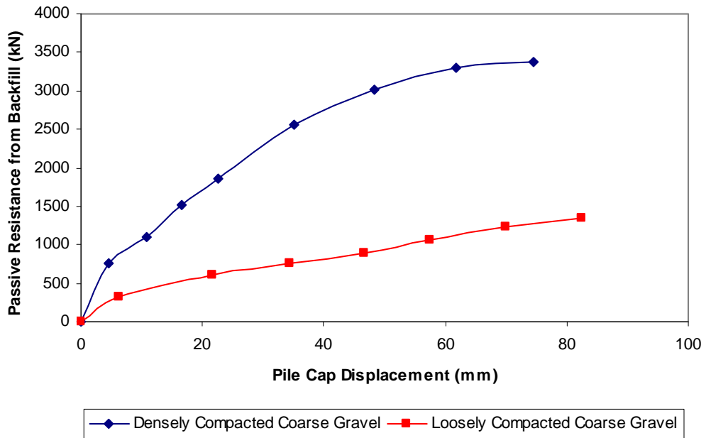
Figure 10-2 Comparison of measured passive earth force-displacement curves for densely and loosely compacted coarse gravel backfill
