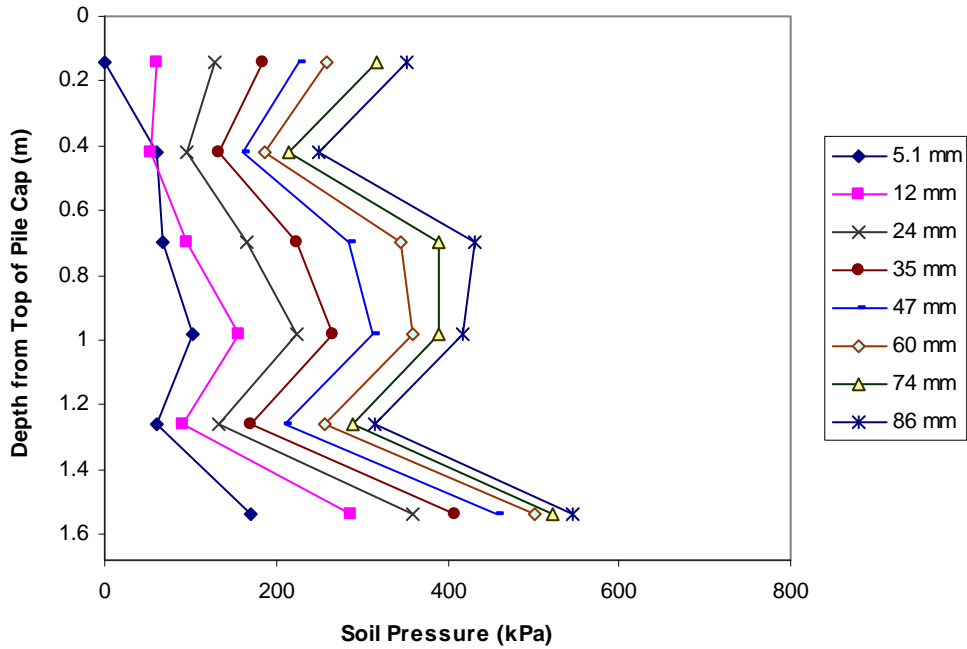
Figure 6-8 Earth pressure distribution as a function of pile cap displacement with densely compacted fine gravel backfill
