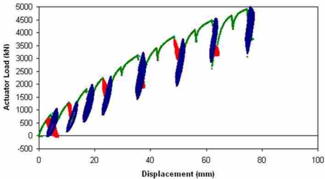
Figure 8-1 Actuator load versus pile cap displacement with densely compacted coarse gravel backfill (Test 12; June 26, 2007)
