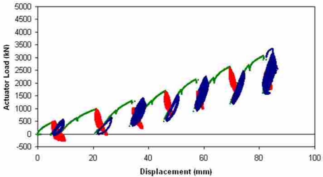
Figure 9-1 Actuator load versus pile cap displacement with loosely compacted coarse gravel backfill (Test 10; June 21, 2007)
