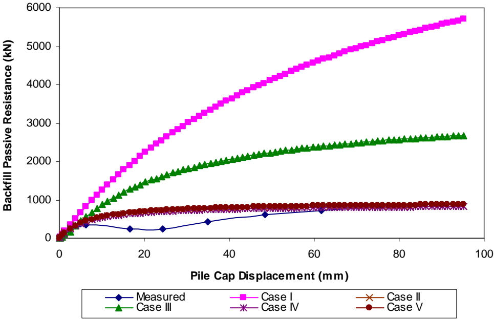
Figure 7-3 Comparison of measured and PYCAP-based calculated passive resistance for loosely compacted fine gravel backfill
