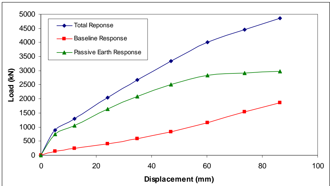
Figure 6-2 Total, baseline, and passive earth responses for pile cap with densely compacted fine gravel backfill
