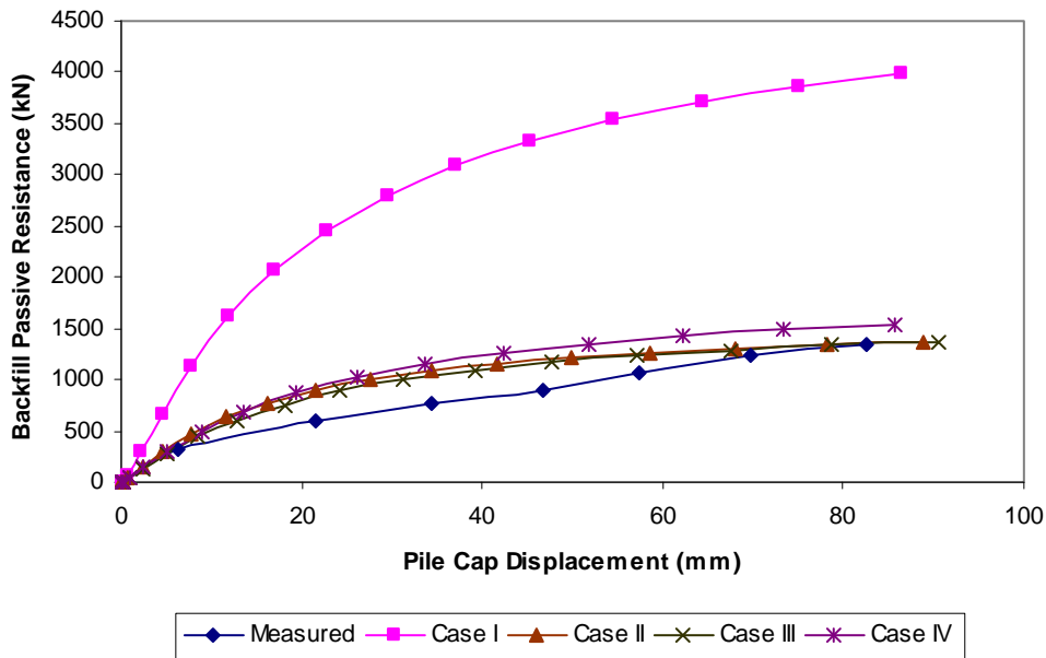
Figure 9-4 ABUTMENT case comparison for loosely compacted coarse gravel backfill
