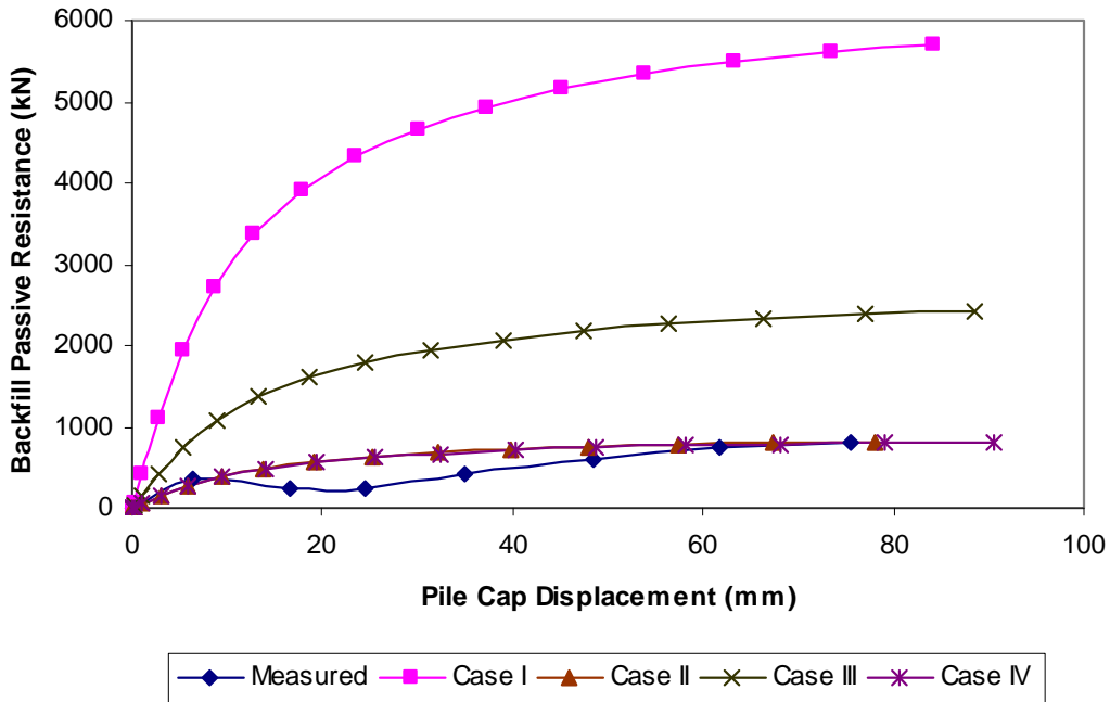
Figure 7-4 Comparison of measured and LSH-based calculated resistance for loosely compacted fine gravel backfill
