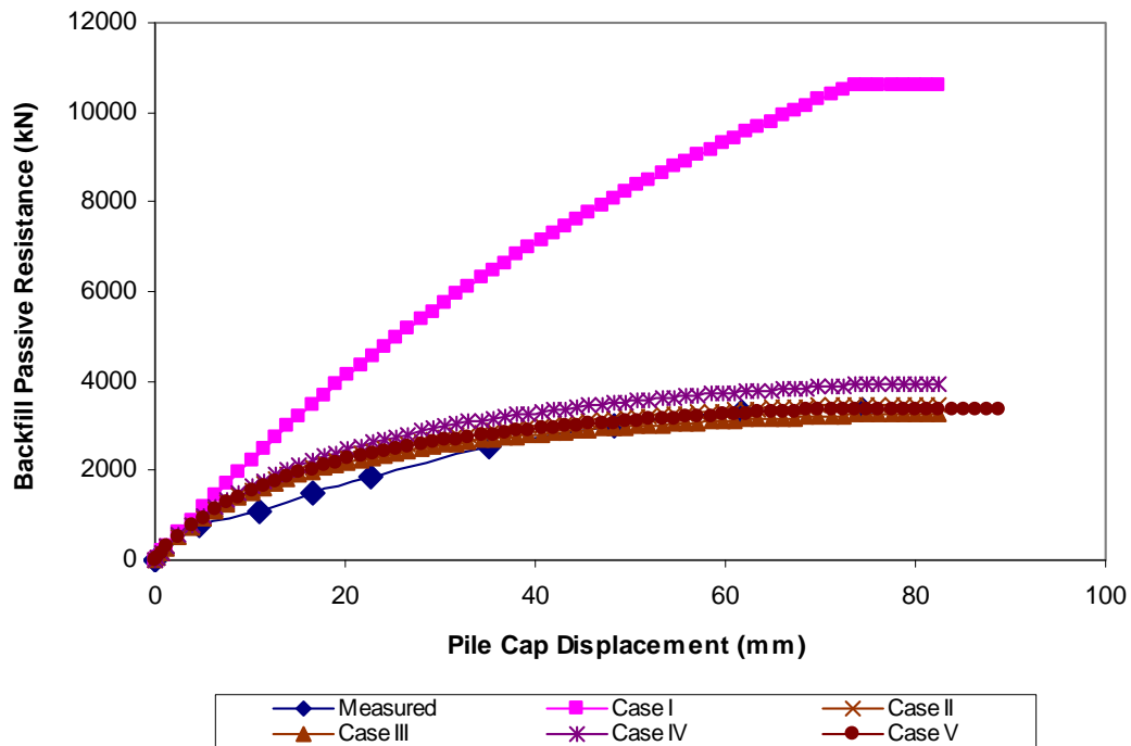
Figure 8-3 PYCAP case comparison for densely compacted coarse gravel
