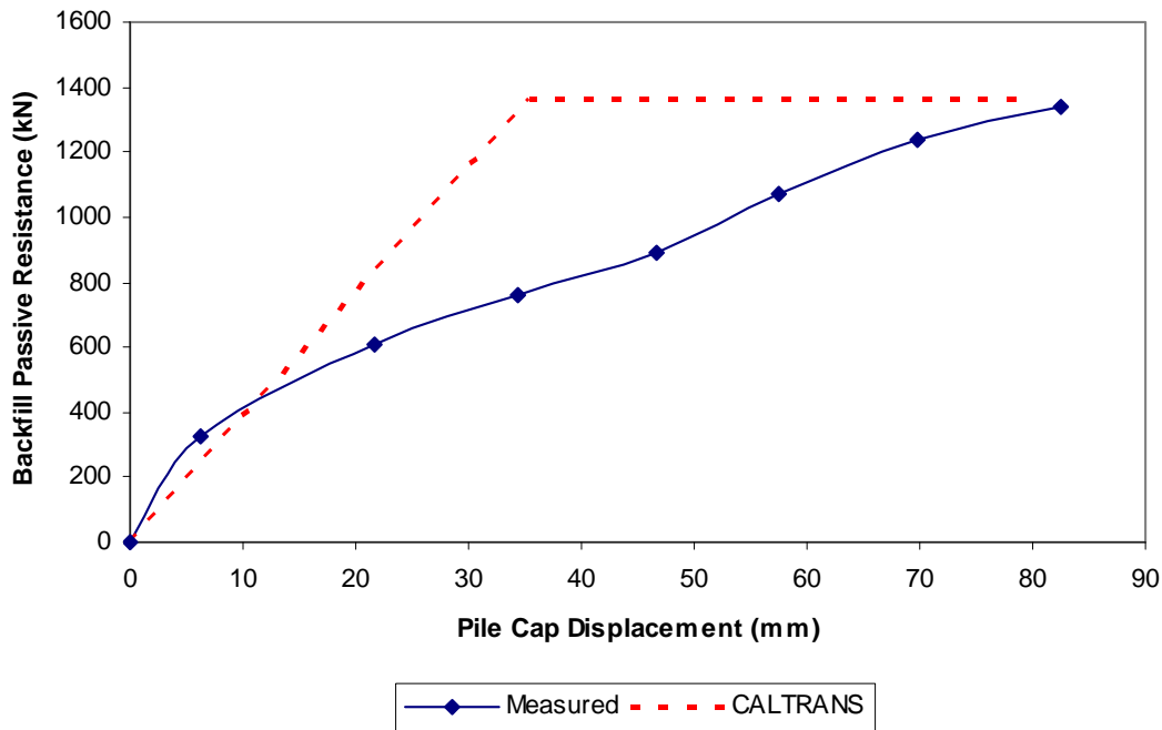
Figure 9-5 Comparison of measured and CALTRANS-based passive resistance for loosely compacted coarse gravel backfill
