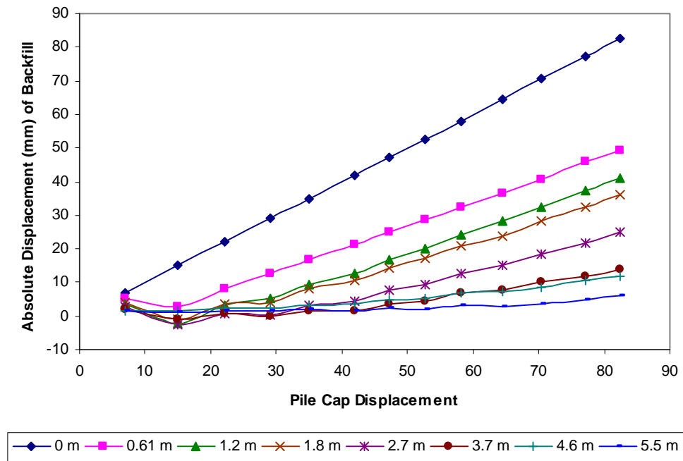
Figure 9-12 Displacement of monitoring points in loosely compacted coarse gravel backfill
