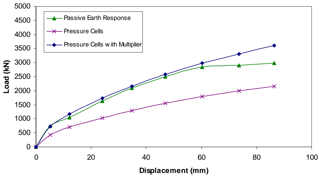
Figure 6-9 Comparison of earth forces based on actuators and pressure cells for densely compacted fine gravel backfill
