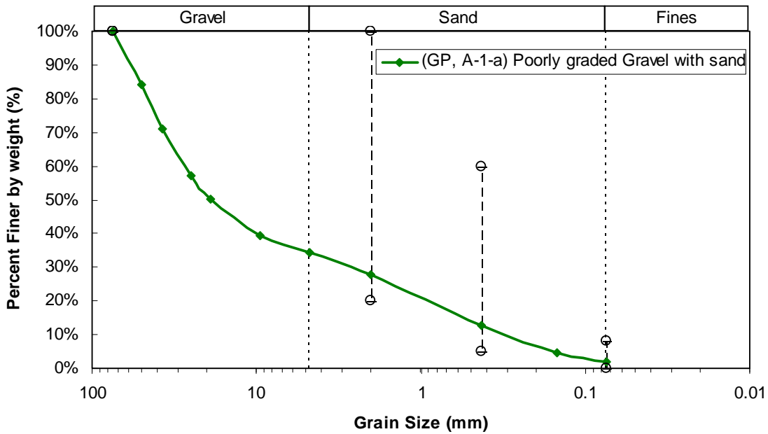
Figure 3-10 Particle distribution and P-154 qualifying limits for coarse gravel backfill
