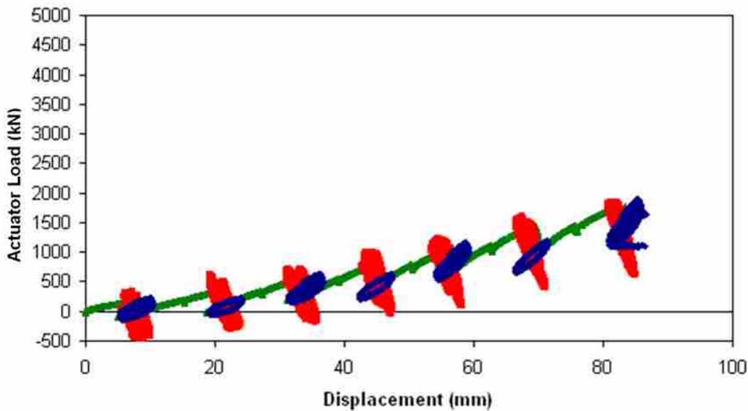
Figure 5-1 Actuator load versus pile cap displacement with no backfill (Test 11; June 21, 2007)
