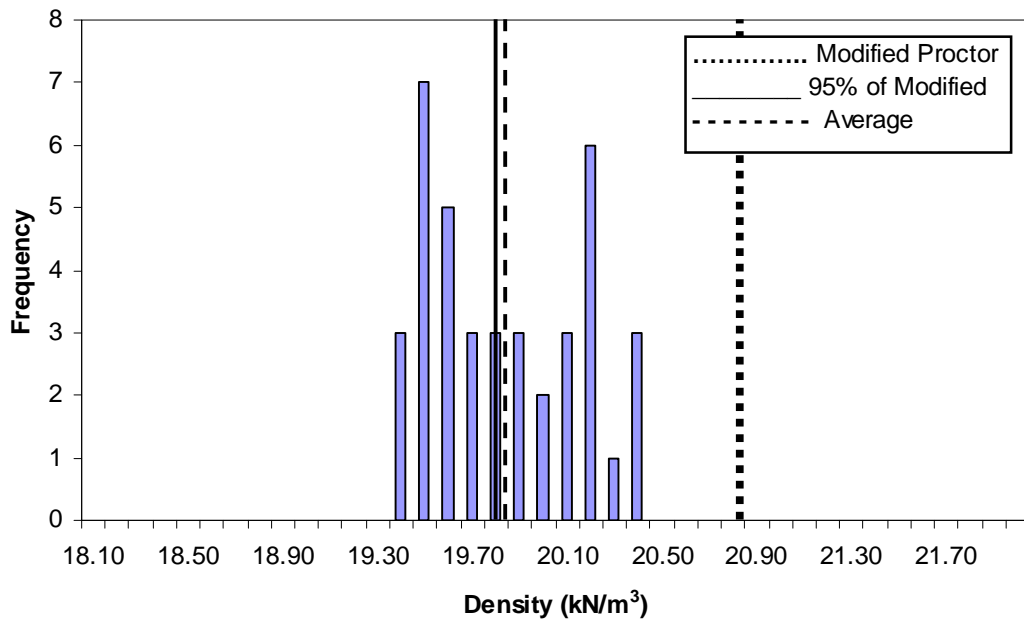
Figure 3-7 Density distribution of densely compacted fine gravel backfill
