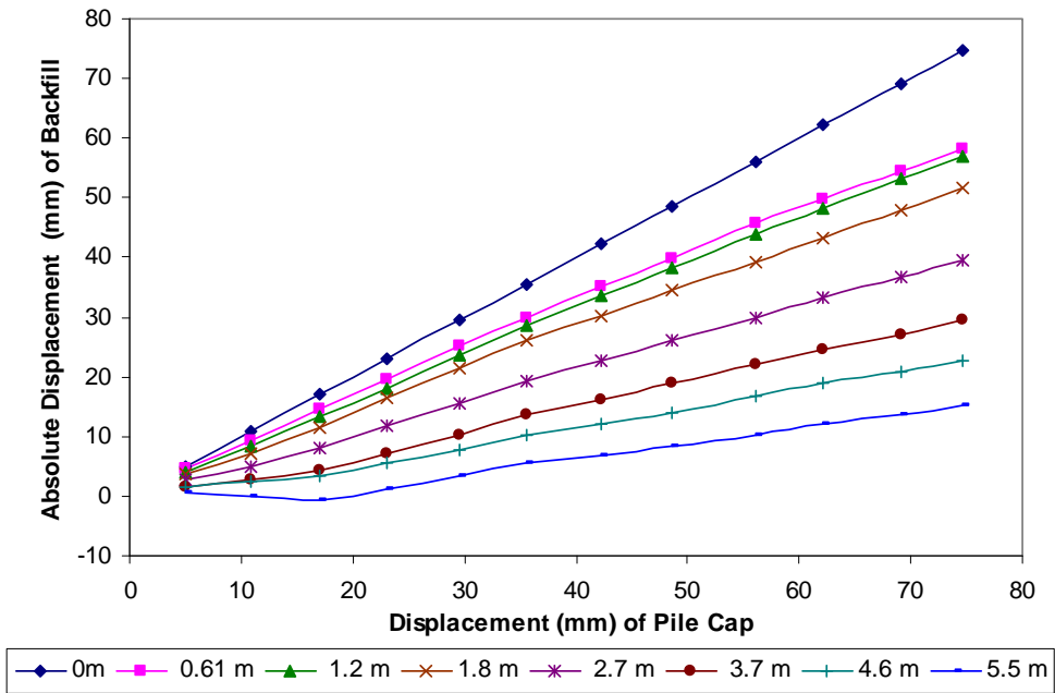
Figure 8-12 Displacement of monitoring points in densely compacted coarse gravel backfill
