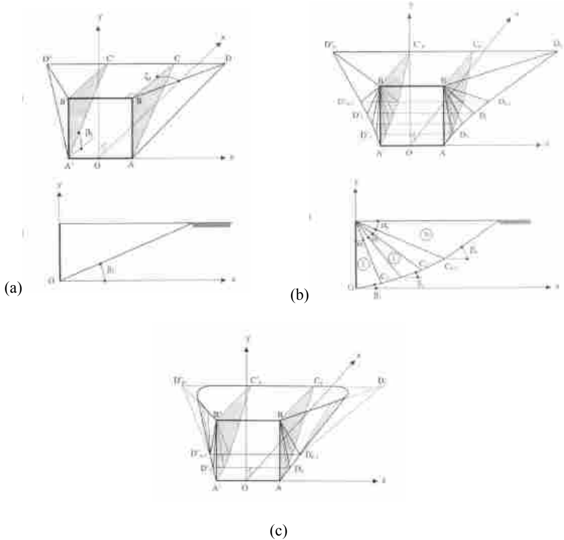
Figure 2-6 Diagrams of different failure mechanisms in Soubra and Regenass (2000)
