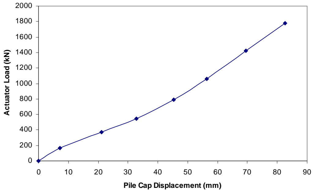
Figure 5-2 Total (and in this case, baseline) static response for pile cap with no backfill
