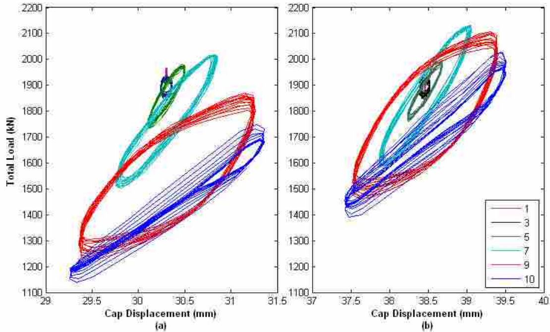
Figure 4-5 Typical load-displacement loops when shaker cycles are applied (a) second and (b) first
