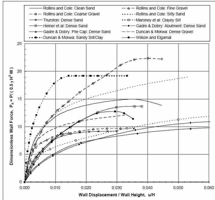
Figure 2-3 Experimental passive force-displacement curves for translation of wall structures from various authors (Wood, 2009)
