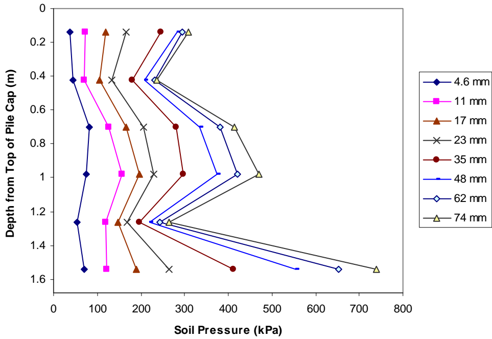
Figure 8-8 Earth pressure distribution as a function of pile cap displacement with densely compacted coarse gravel
