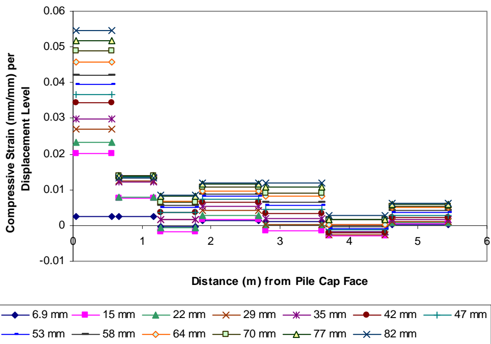
Figure 9-13 Strain per displacement level for loosely compacted coarse gravel backfill
