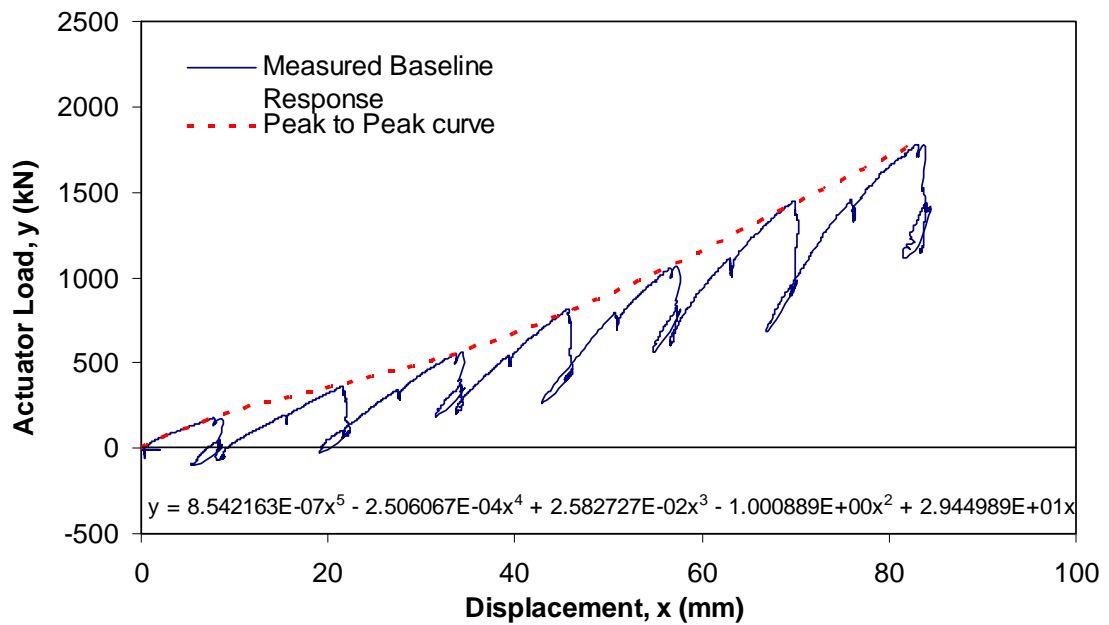
Figure 4-2 Measured baseline response with modeled baseline response
