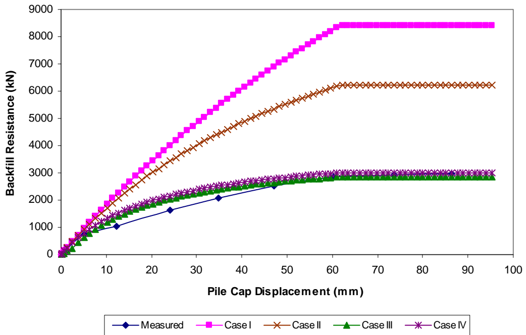
Figure 6-3 PYCAP case comparison for densely compacted fine gravel backfill
