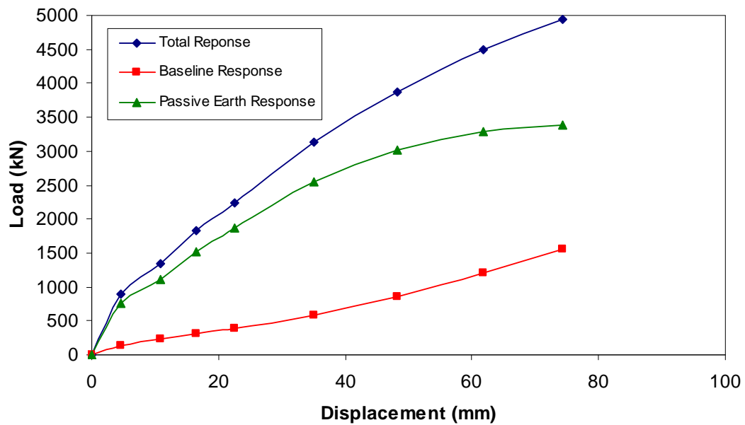
Figure 8-2 Total, baseline, and passive earth responses for pile cap with densely compacted coarse gravel backfill
