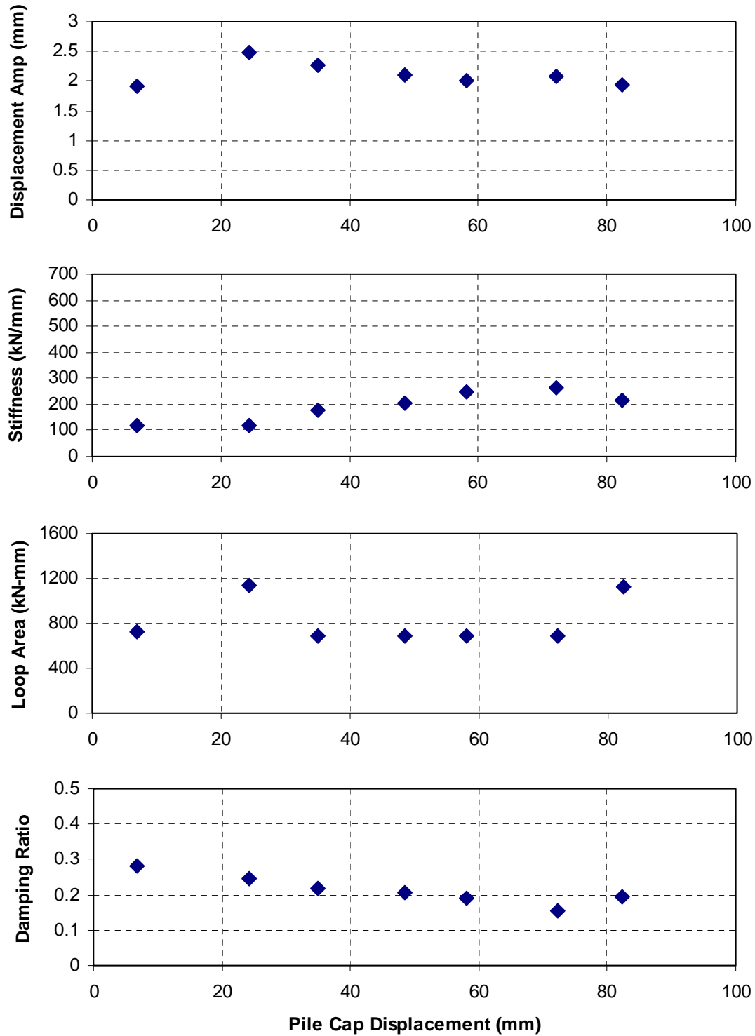
Figure 9-6 Summary of response to cyclic actuator loadings for pile cap with loosely compacted coarse gravel backfill
