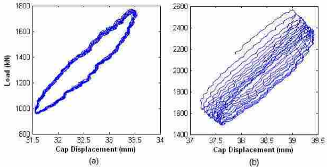
Figure 4-4 Typical actuator loops when actuator cycles are applied (a) second and (b) first
