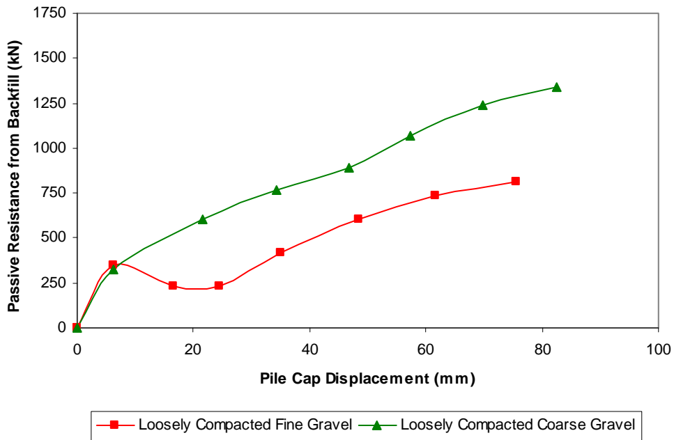
Figure 10-4 Comparison of measured earth force-displacement curves for loosely compacted backfills
