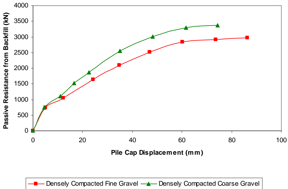
Figure 10-3 Comparison of measured earth force-displacement curves for densely compacted backfills
