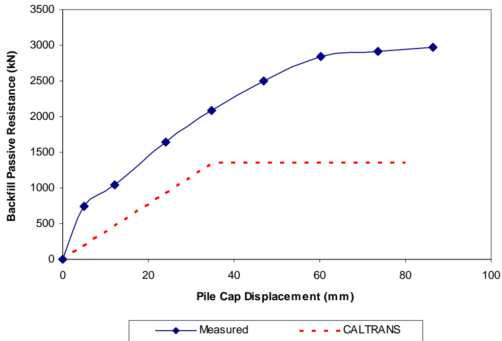
Figure 6-5 Comparison of measured and CALTRANS-based passive resistance for densely compacted fine gravel backfill
