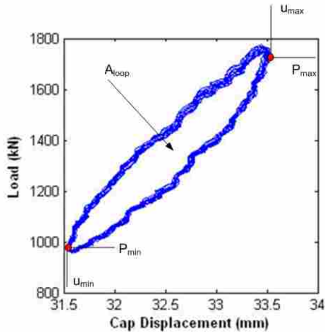
Figure 4-3 Example of actuator-based load-displacement loops
