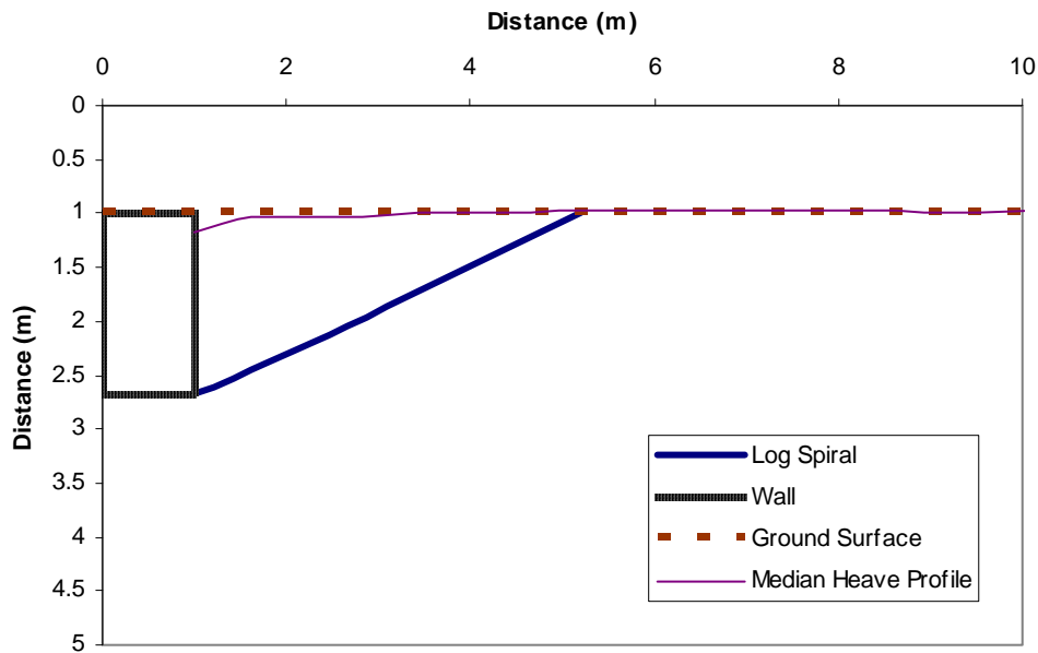
Figure 7-11 Heave profile with best-fit log-spiral failure surface from PYCAP for loosely compacted fine gravel backfill
