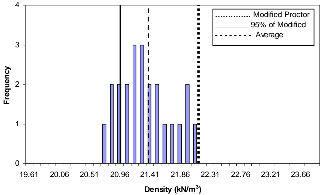
Figure 3-11 Density distribution of densely compacted coarse gravel backfill
