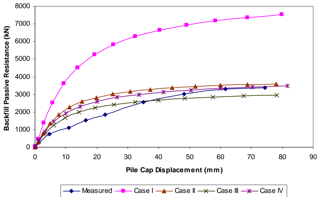
Figure 8-4 ABUTMENT case comparison for densely compacted coarse gravel backfill
