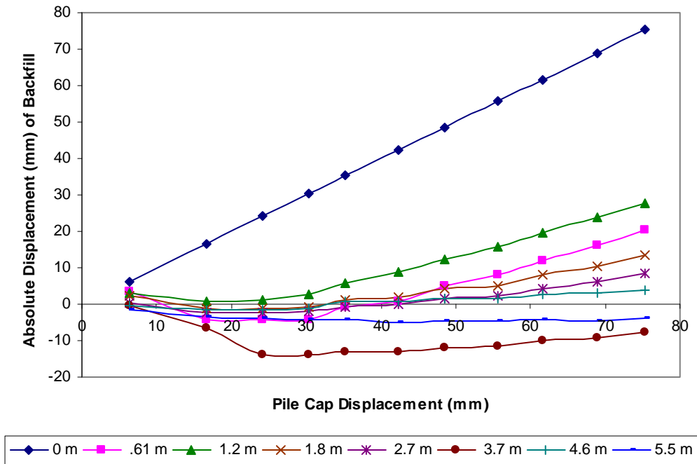
Figure 7-12 Displacement of monitoring points in loosely compacted fine gravel backfill
