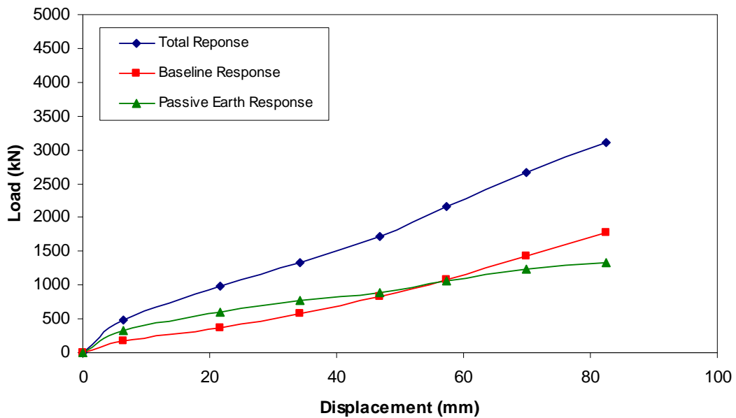
Figure 9-2 Total, baseline, and passive earth responses for pile cap with loosely compacted coarse gravel backfill
