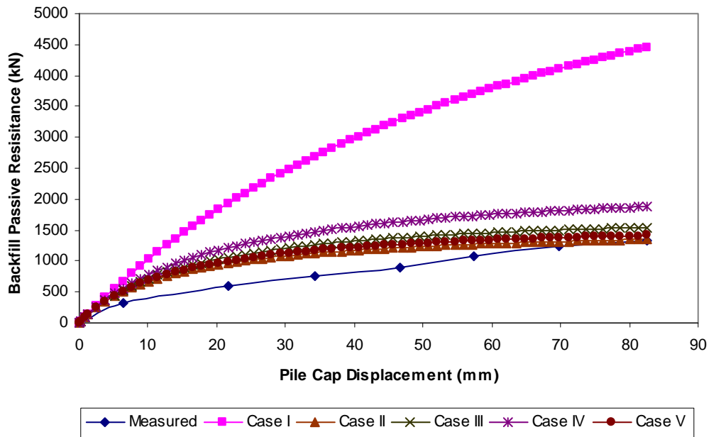
Figure 9-3 PYCAP case comparison for loosely compacted coarse gravel backfill
