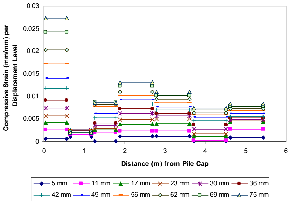
Figure 8-13 Strain per displacement level for densely compacted coarse gravel backfill
