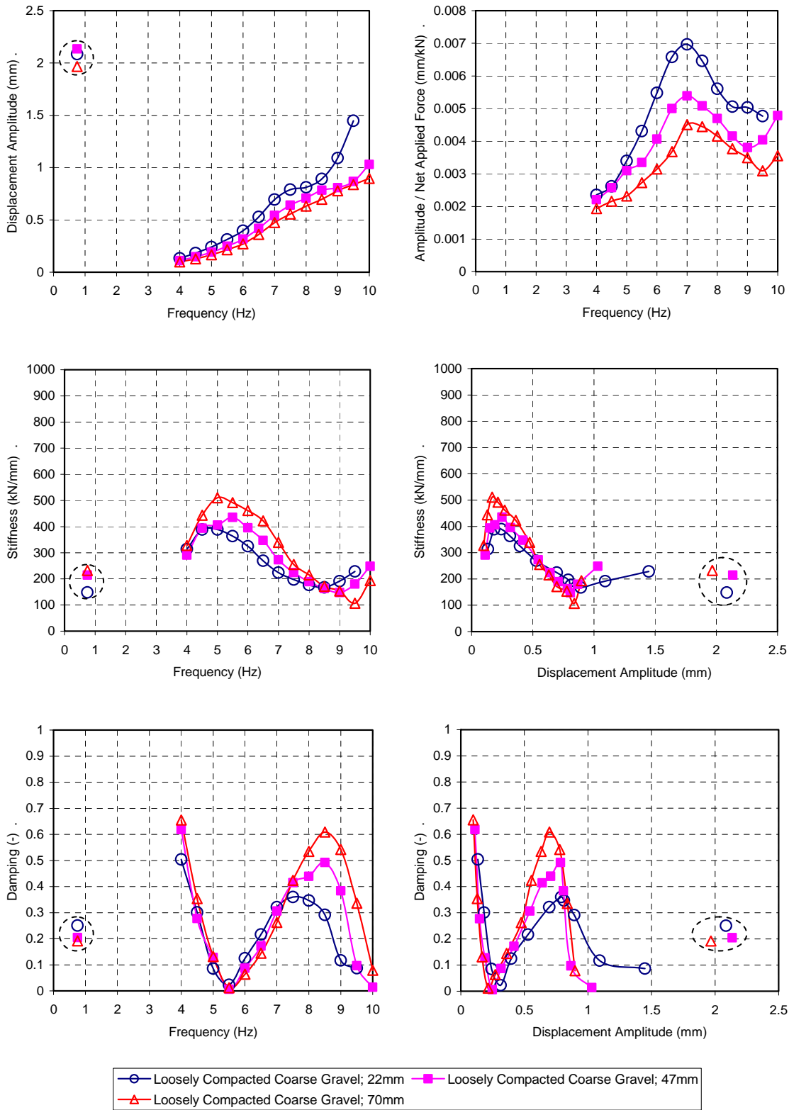
Figure 9-7 Summary of response to dynamic shaker loadings for pile cap with loosely compacted coarse gravel backfill
