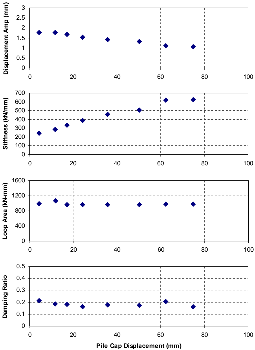
Figure 8-6 Summary of response to cyclic actuator loadings for pile cap with densely compacted coarse gravel backfill
