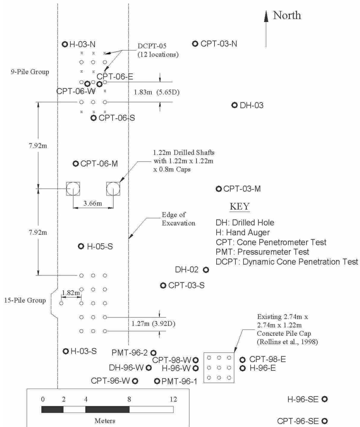
Figure 3-2 Entire test site with locations of subsurface tests (Christensen, 2006)
