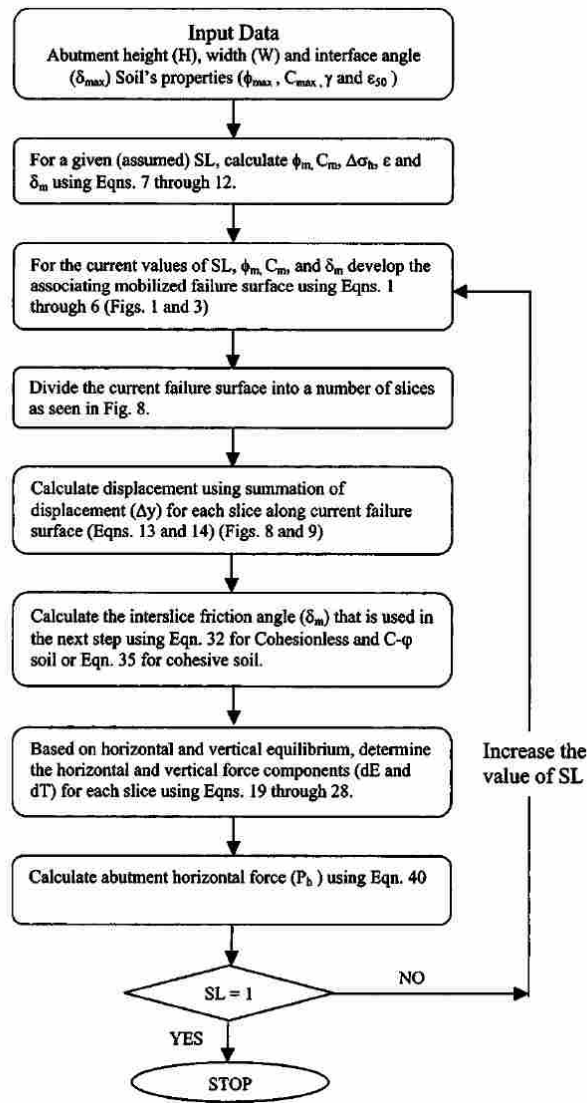
Figure 2-4 Method developed in Shamsabadi et al. (2005) to compute the passive resistance of a backfill soil
