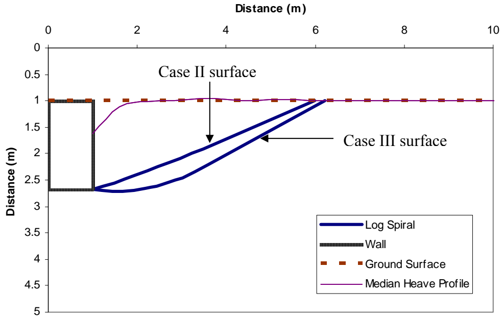
Figure 9-11 Heave profile with “best-fit” (Case II) and “most-representative” (Case III) log-spiral failure surfaces from PYCAP for loosely compacted coarse gravel
