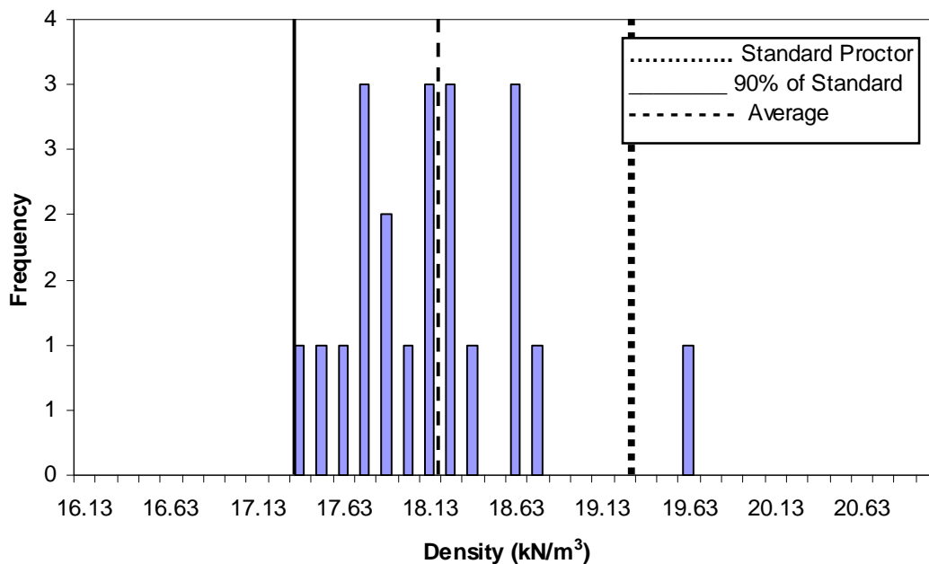
Figure 3-8 Density distribution of loosely compacted fine gravel backfill
