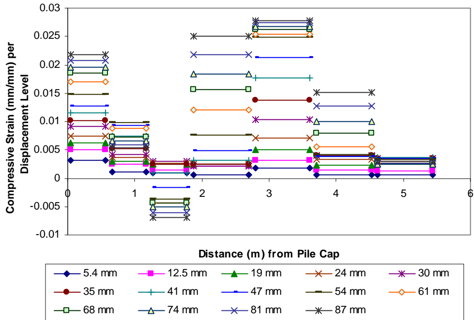
Figure 6-13 Strain per displacement level for densely compacted fine gravel backfill
