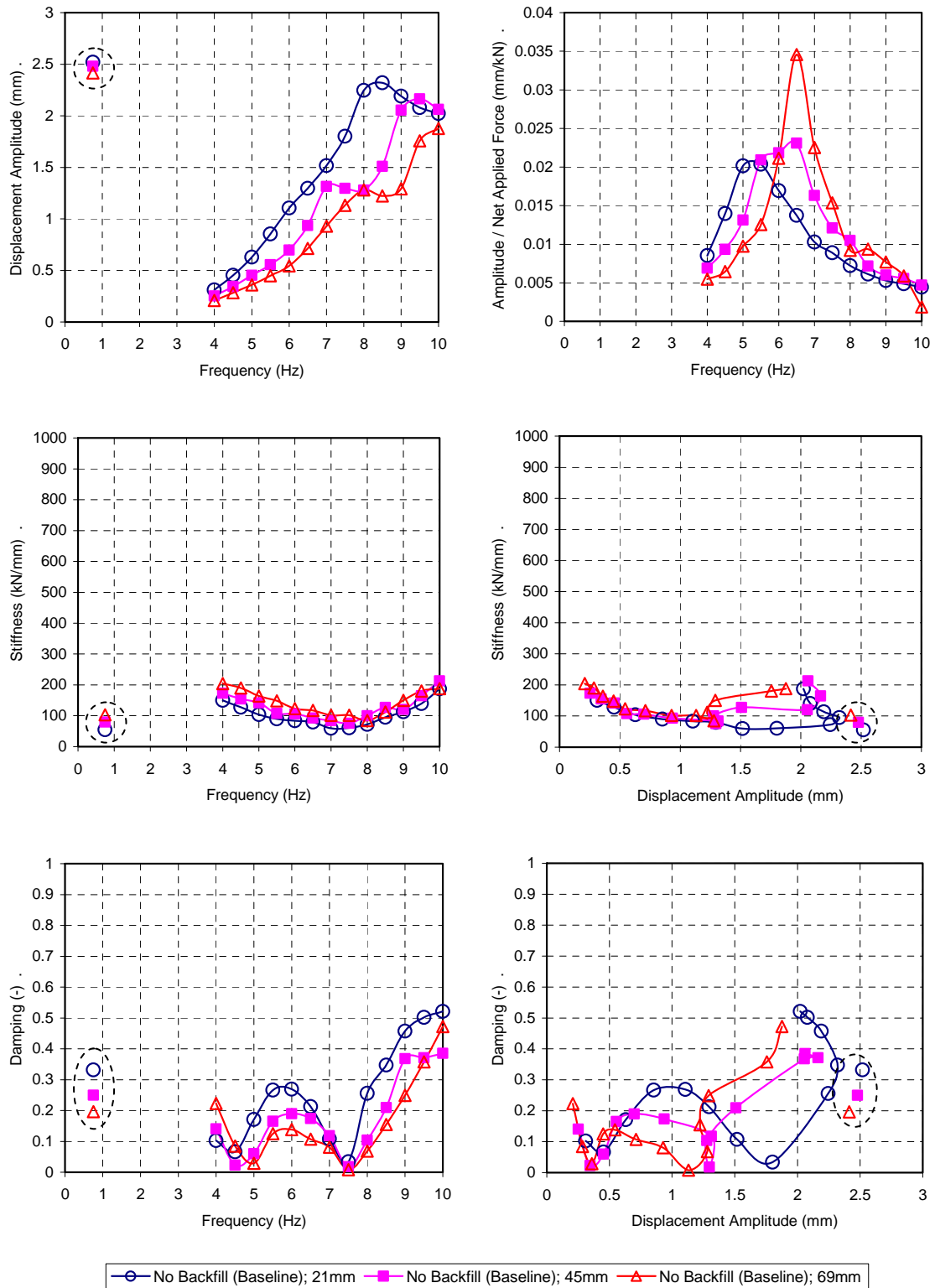
Figure 5-4 Summary of response to dynamic shaker loadings for pile cap without backfill (baseline condition)
