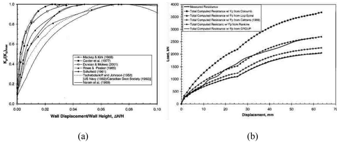
Figure 2-2 (a) Comparison of normalized load-displacement curves from various authors; (b) comparison of various passive resistance estimation procedures with measured resistance
