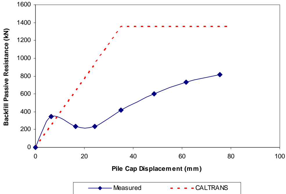
Figure 7-5 Comparison of measured and CALTRANS-based passive resistance for loosely compacted fine gravel backfill
