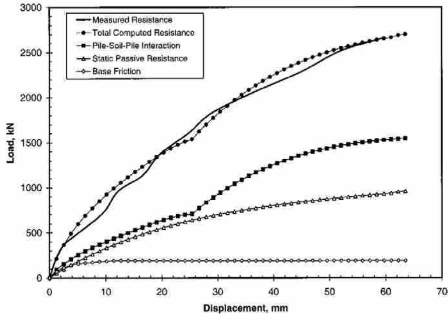
Figure 2-1 Contribution of various components to the total lateral resistance of a pile cap with sandy gravel backfill
