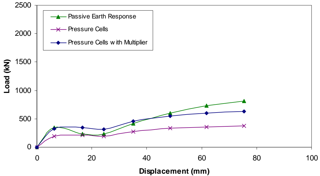
Figure 7-9 Comparison of earth forces based on actuators and pressure cells for loosely compacted fine gravel backfill
