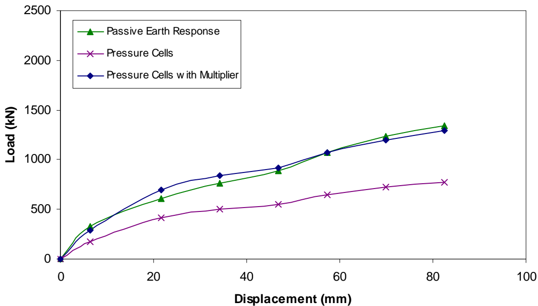
Figure 9-9 Comparison of earth forces based on actuators and pressure cells for loosely compacted coarse gravel backfill
