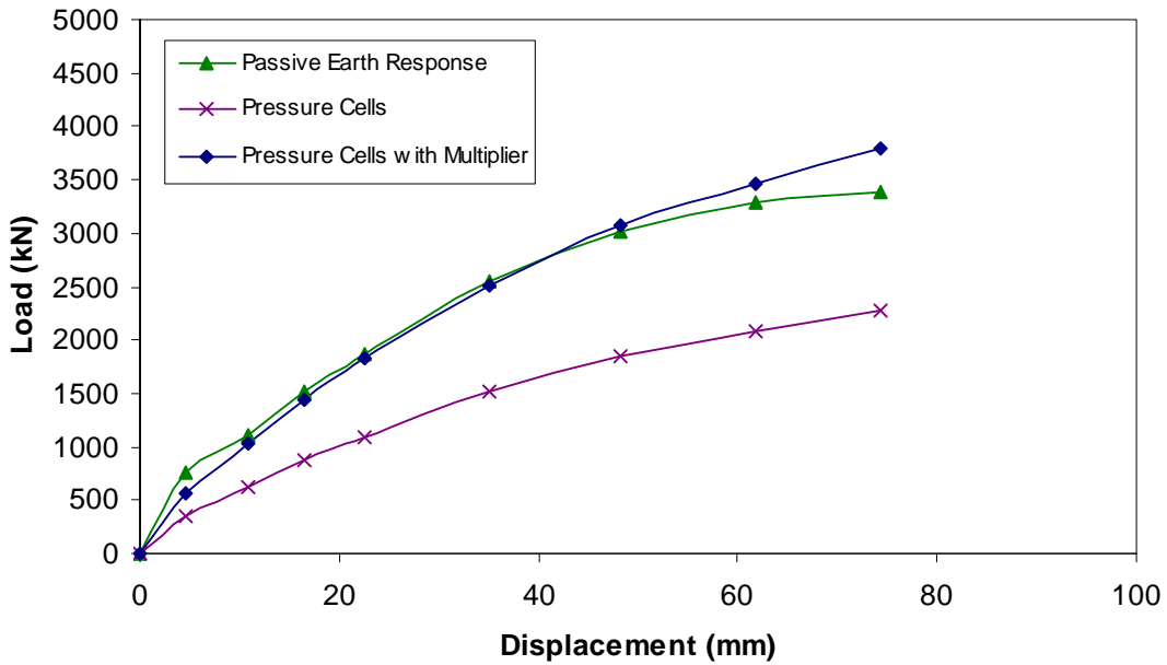
Figure 8-9 Comparison of earth forces based on actuators and pressure cells for densely compacted coarse gravel backfill
