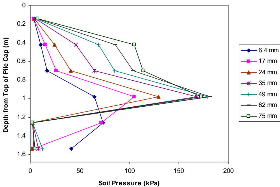
Figure 7-8 Earth pressure distribution as a function of pile cap displacement with loosely compacted fine gravel
