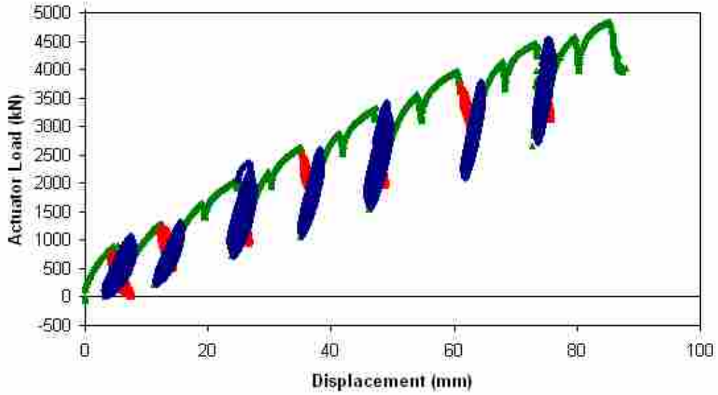
Figure 6-1 Actuator load versus pile cap displacement with densely compacted fine gravel backfill (Test 8; June 11, 2007)
