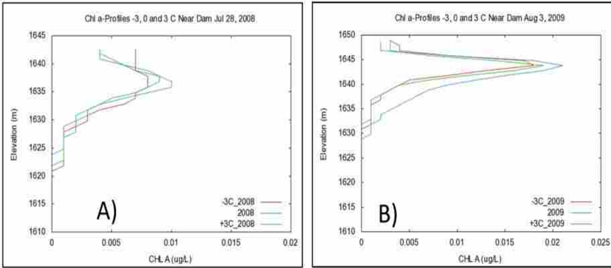
Figure 4.1: Chlorophyll-a profiles at the Near Dam sampling point by adjusting air temperature: A) Summer 2008 and B) Summer 2009
