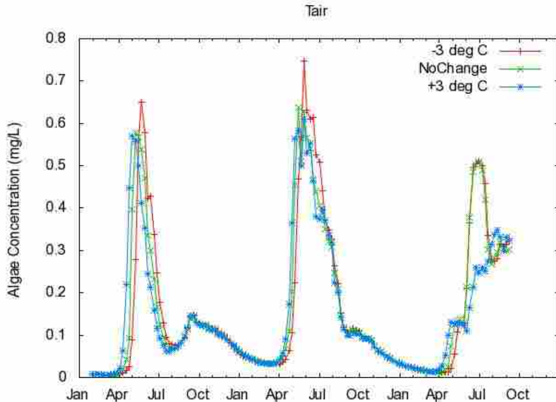
Figure 4.8: Total algae concentrations by simulating air temperature scenarios in Deer Creek, -3°C, no change, +3°C
