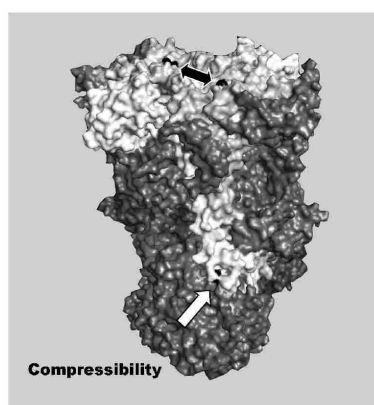
Figure 8 Amino acids undergoing radical biochemical shifts in compressibility. Three-dimensional representations of ISP and cyt- c_1 are shaded as in Figure 5. Arrows indicate the locations of amino acid sites discussed in the text
