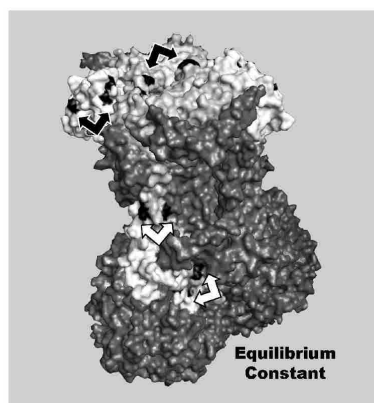
Figure 7 Amino acids undergoing radical biochemical shifts in pK' . Three-dimensional representations of ISP and cyt- c_1 are shaded as in Figure 5. Arrows indicate the locations of amino acid sites discussed in the text
