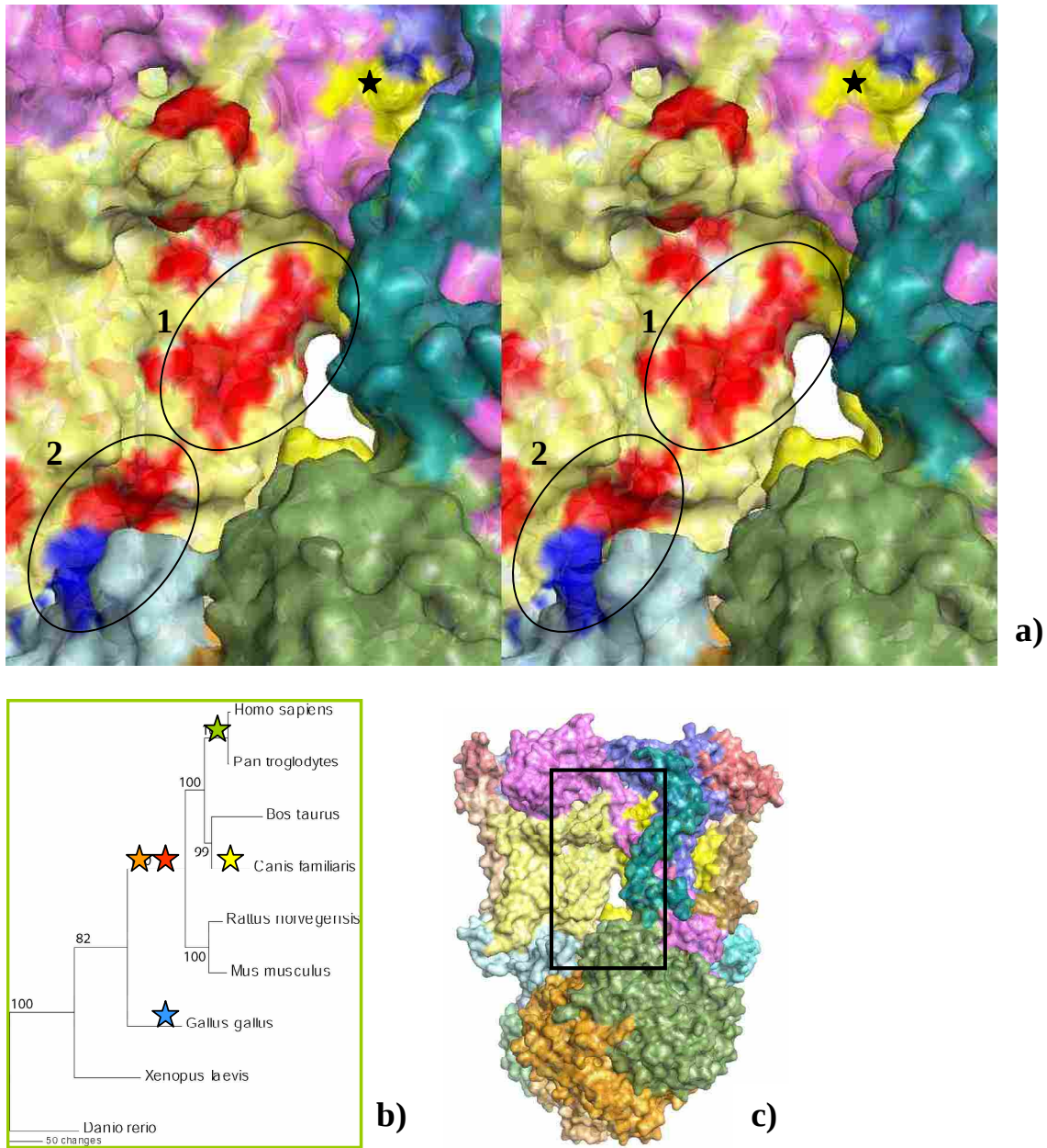
Figure 16: (a) Close up view of the transmembrane region, specifically the region of cyt b that is between heme b_H and heme b_L . Selection on cyt b is shown in red on one dimer and indigo on the other dimer. Selection on subunit 6 is shown in bright blue. In circle 1, which is directly between the two hemes of cyt b , there are 2 examples of coevolution and one of coadaptation. The changes: L184I and I192L (cyt b ) increase and decrease equilibrium constant respectively on the branch leading to mammals (red star). The changes: V117I and I118V (cyt b ) increase and decrease equilibrium constant respectively on the terminal branch of Canis familiaris (yellow star). The changes: I188L and I115T (cyt b ) decrease SARR on the terminal branch leading to Gallus gallus (blue star). In circle 2, which is directly behind heme b_L , there is one example of coevolution and one example of coadaptation between cyt b and subunit 6. Sites L108I, K110I (cyt b ) decrease equilibrium constant, Y109F (cyt b ) decreases mean r.m.s. fluctuation displacement & D40N (sub 6) decreases power to be at the C-terminus on the branch leading to all mammals (orange star). Later in the phylogeny, on the branch leading to primates (green star) there are reversals of the sites above, except I110L instead of K. The star shows the one site under selection near the location of the second proton exit. The indigo site indicates R71F (cyt b ) and is only under selection on the terminal branch to Xenopus laevis . (b) Phylogeny showing location of changes discussed in the paper. Red, yellow and blue stars are in circle 1 and orange and green are in circle 2. (c) Entire complex shown, with box indicating the close-up region in (a).
