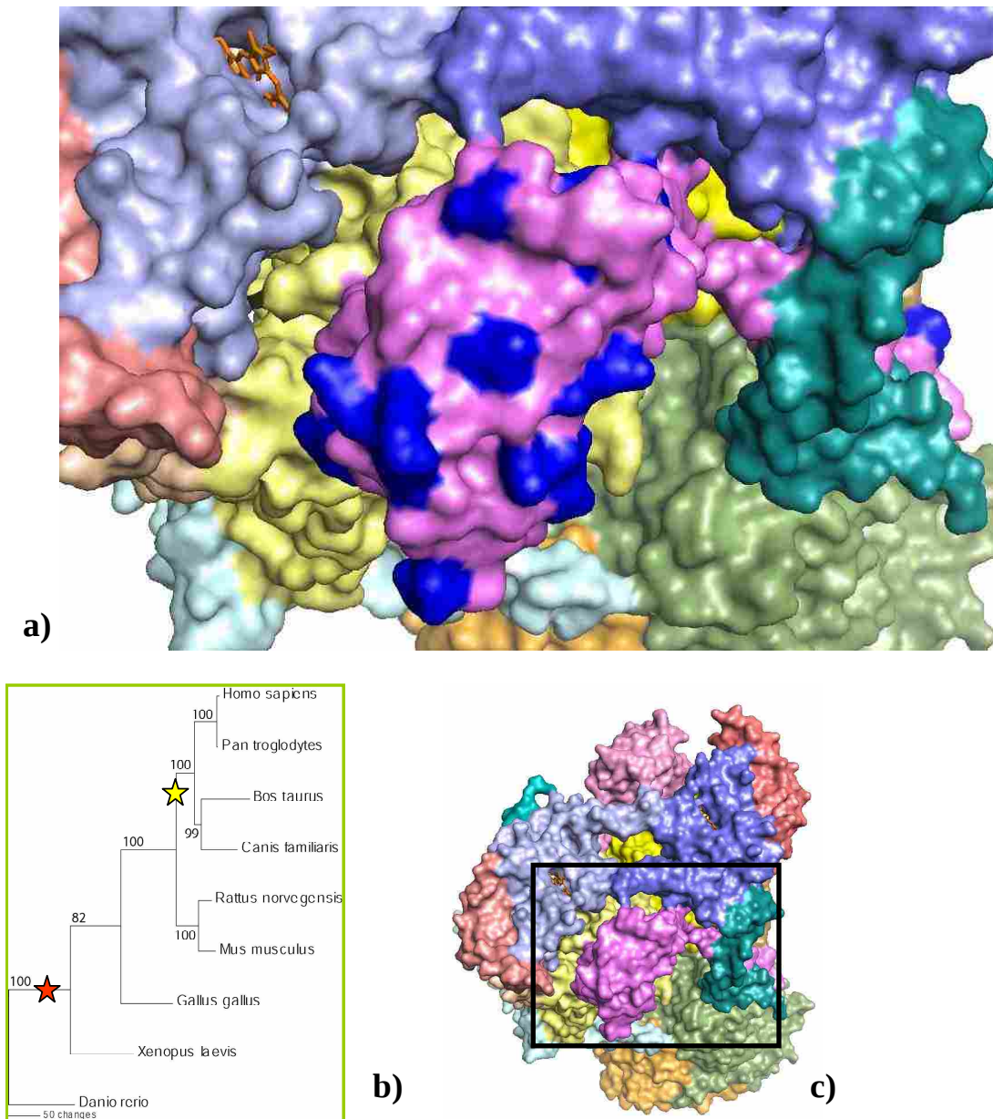
Figure 17: (a) Selection on the ISP head region is shown in bright blue. The ISP head region shows many sites experiencing physicochemical shifts. There is one example of coadaptation on the head region of ISP: E128K & S170R both increase isoelectric point and one example of coevolution: D131E & E107D reciprocal increase and decrease in turn tendency on the phylogenetic branch separating Danio rerio as the outgroup (red star). There is also one example of coevolution on the branch grouping humans, chimps, cow, and dog: I192M & V194I show reciprocal increase and decrease in the equilibrium constant (yellow star). The other changes, that do not show coevolution or coadaptation include: T88A (alpha helical tendency), S72A (alpha helical tendency), S79A (alpha helical tendency), E103A (compressibility), K104A (hydropathy, short and med range non-bonded energy), D107N (power to be at the C-terminus), N113D (power to be at the C-terminus), E116K (isoelectric point), I124K (buriedness, equilibrium constant, long-range non-bonded energy, SARR, surrounding hydrophobicity, total non-bonded energy), D125E (turn tendency), D131S power to be at the C-terminal), A150S (turn tendency), E152D (turn tendency), and S170R (short and medium range non-bonded energy, partial specific volume, helical contact area). (b) Phylogenetic tree and locations of the evolutionary changes discussed above. (c) Square shows the region of the bc 1 complex that is enlarged in (a).
