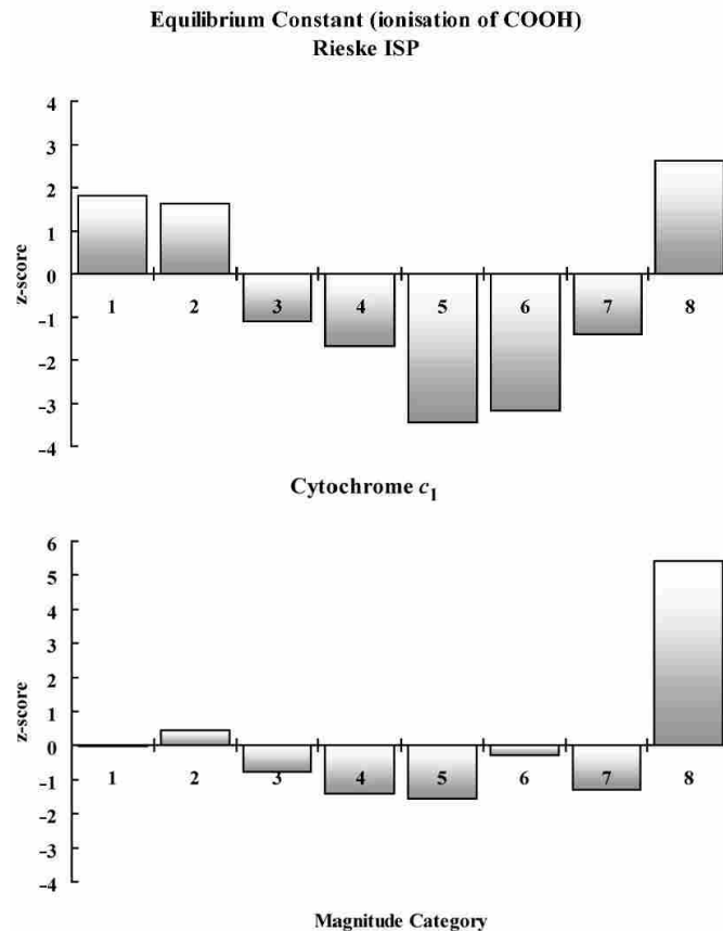
Figure 6 Extremely radical changes (category 8) in pK' in ISP ( p < 0.01 ) and cyt- c_1 ( p < 0.001 ) are affected by positive-destabilising selection. Positive-stabilising selection also is at work in ISP (category 1), promoting only the most conservative changes ( p < 0.05 )
