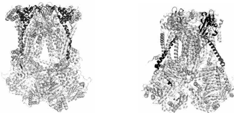
FIGURE 1: Location of cytochrome c_1 (black, left) and Rieske ISP (black, right) dimers in cytochrome bc_1 complex (gray).
