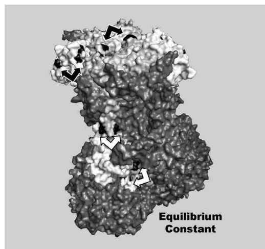
Figure 9: Amino acids undergoing radical biochemical shifts in pK' . Three-dimensional representations of ISP and cyt- c_1 are shaded as in Fig 5. Arrows indicate the locations of amino acid sites discussed in the text.
