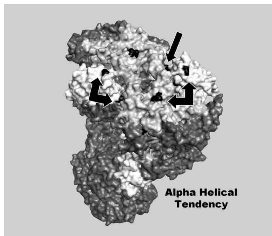
FIGURE 5: Three-dimensional representation of specific amino acids undergoing destabilizing structural shifts in \alpha -helical tendency. ISP is white, cyt- c 1 is shaded light gray, and adaptive sites are black. All other subunits of the bc 1 complex are shaded dark gray. Arrows indicate positively selected amino acid sites buried in the tertiary structures.
