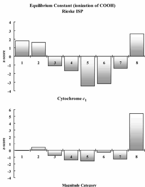
Figure 8: Extremely radical changes (category 8) in pK' in ISP ( p < 0.01 ) and cyt- c_1 ( p \ll 0.001 ) are affected by positive-destabilizing selection. Positive-stabilizing selection also is at work in ISP (category 1), promoting only the most conservative changes ( p < 0.05 ).
