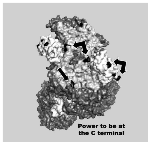
Figure 11: Amino acids undergoing radical biochemical shifts in power to be at the C-terminal. Three-dimensional representations of ISP and cyt- c_1 are shaded as in Fig 5. Arrows indicate the locations of amino acid sites discussed in the text.
