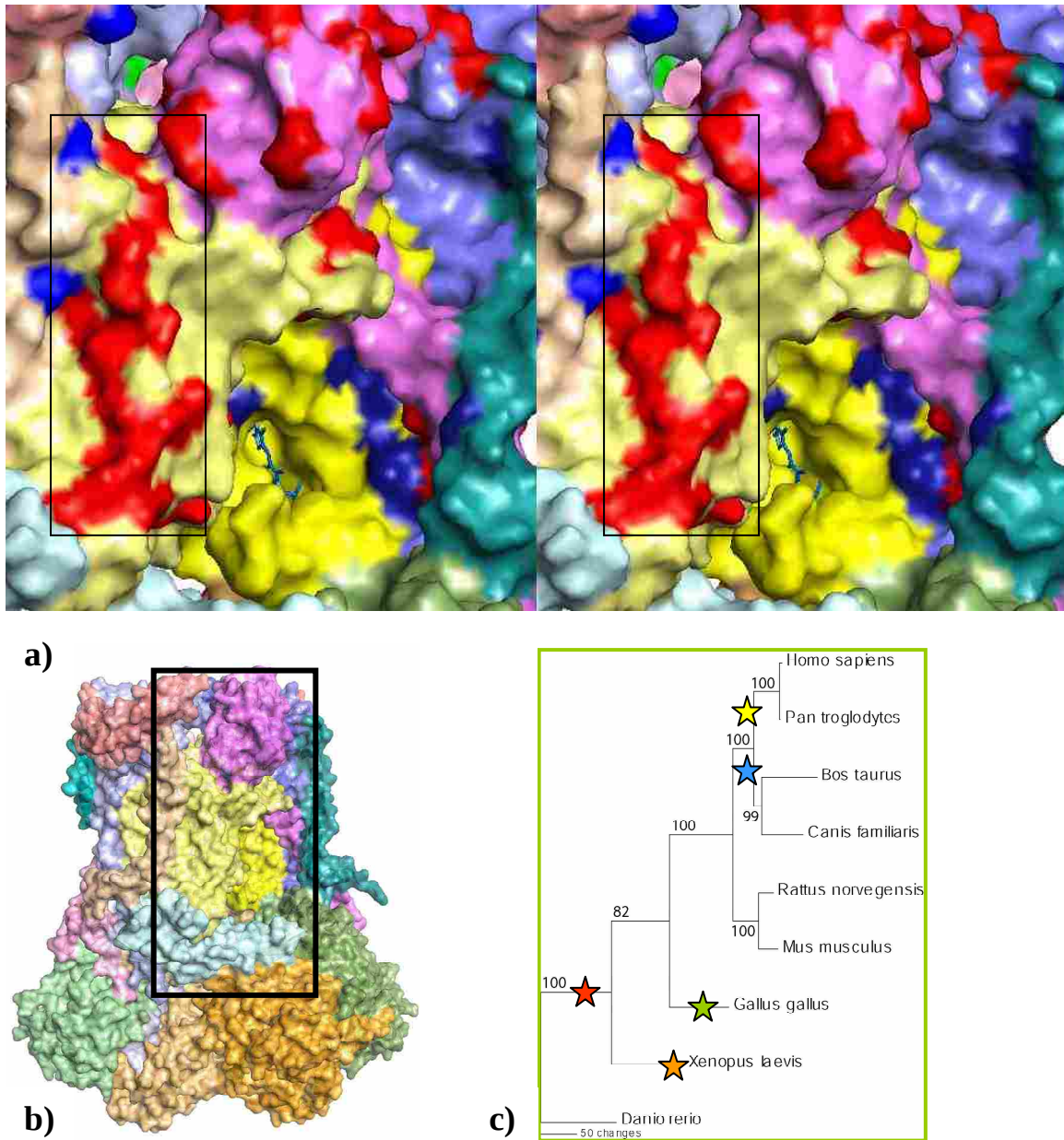
Figure 19: The box indicates those sites that are under selection on and around helix H of cyt b . Selection on cyt b is shown in red, as well as selection on ISP. Subunit 7 selection is shown in bright blue. This region is undergoing heavy selection with many examples of coadaptation occurring here. The changes L361I, V364I, L372I, A376I (cyt b ) all decrease equilibrium constant (red star). The changes I356V & I371L (cyt b ) increase equilibrium constant while I361T (cyt b ) decreases SARR (yellow star). The changes I353L (cyt b ) & I58V (sub 7) increase equilibrium constant while I368T & I334T (cyt b ) decrease SARR (blue star). The terminal branches to Xenopus laevis and Gallus gallus show more examples of coevolution and coadaptation. Xenopus shows six sites that increase and three that decrease equilibrium constant, while two sites decrease and one site increases SARR in this 'stripe' region (orange star). Gallus shows three sites that increase equilibrium constant, while two sites decrease and one site increases SARR (green star). (b) Shows the region of the protein viewed in (a). (c) Shows phylogenetic tree with locations of changes discussed above.
