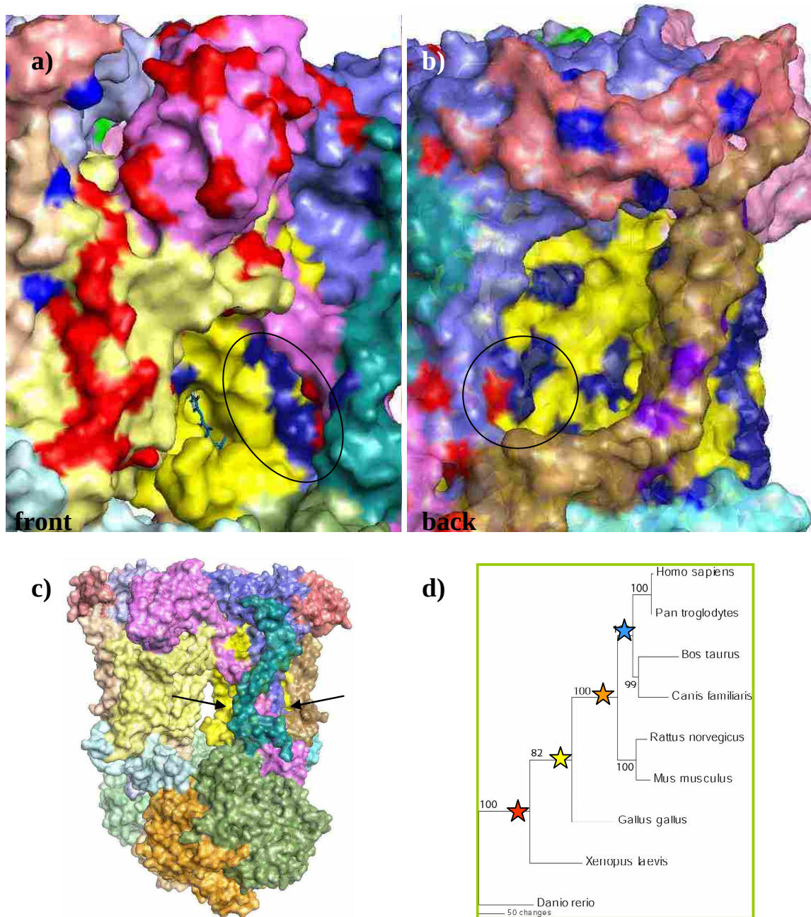
Figure 20: The selection on cyt b is shown in indigo, while the selection on ISP and cyt c 1 is shown in red. Selection on subunit 10 is shown in dark blue, while selection on subunit 7 is shown in purple. This view is of selection on helix E of cyt b , which is located adjacent to the Q i site (shown with heme) and directly behind the transmembrane helices of cyt c 1 , ISP and subunit 10. (a) Shows the front face of helix E, while (b) shows the back face of helix E. Selection on the front shows one example of coadaptation, I82L (cyt b ) & I122M (cyt c 1 ) both increase equilibrium constant (red star). Also on the front side of this helix, changes from different amino acids of cyt b all to isoleucine cause shifts in different properties: 226I decrease in coil tendency, L229I decrease in equilibrium constant, T240I increase in buriedness, SARR and thermodynamic transfer hydrophobicity (yellow star). While the back side of this helix shows reversals of these changes from isoleucine to leucine: I235L and I234L increase in equilibrium constant (cyt b ) (orange star), and I216L increase in equilibrium constant (cyt c 1 ) (blue star). (c) Indicates the location of helix E via the arrows. (d) Phylogenetic tree showing locations of changes discussed above.
