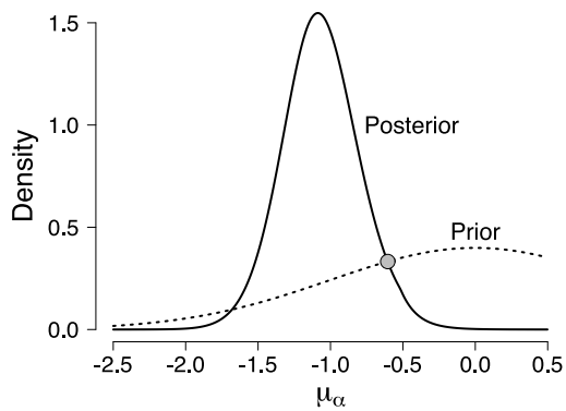
Fig. 7. Prior and posterior distribution of the group-level mean \mu_\alpha in the Busemeyer and Stout (2002) data set. The figure shows the posterior distribution (solid line) and the prior distribution (dotted line). The gray dot indicates the intersection of the prior and the posterior distributions, for which the Savage–Dickey Bayes factor equals 1. Available at https://tinyurl.com/y7cyxclq under CC license https://creativecommons.org/licenses/by/2.0/ .
