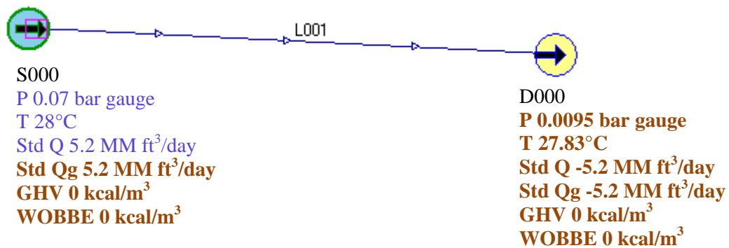
Figure 5. Pipe phase model of the cold vent compression project. Source: Chevron Nigeria Limited.
