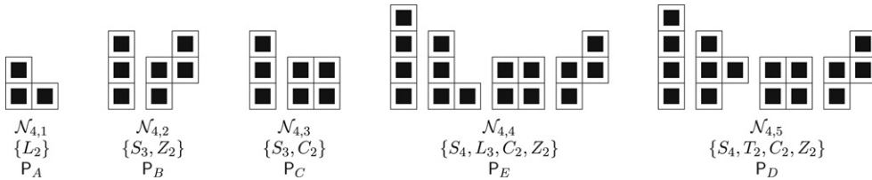
Fig. 6.6. Characterizing teams for size 4. Killer 2-pavings are listed for losing teams. No winning team is required.
