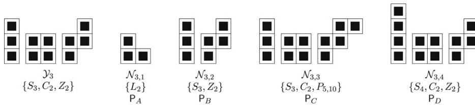
Fig. 6.3. Characterizing families for size 3. Killer 2-pavings are listed for losing families.
