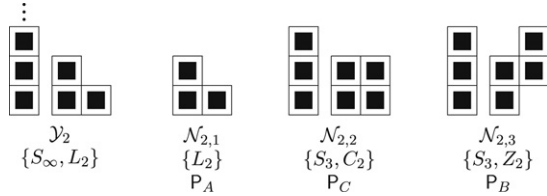
Fig. 6.2. Characterizing families for size 2. Killer 2-pavings are listed for losing families.
