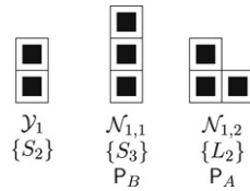
Fig. 6.1. Characterizing families for size 1. Killer 2-pavings are listed for losing families.
