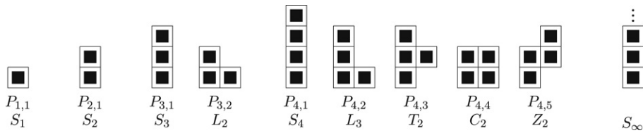
Fig. 2.1. All polyominoes up to size 4 together with infinite skinny.
