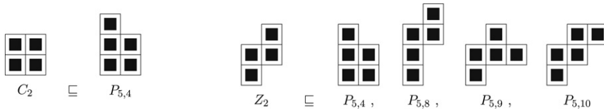
Fig. 6.4. Descendants of C_2 and Z_2 with size 5.
