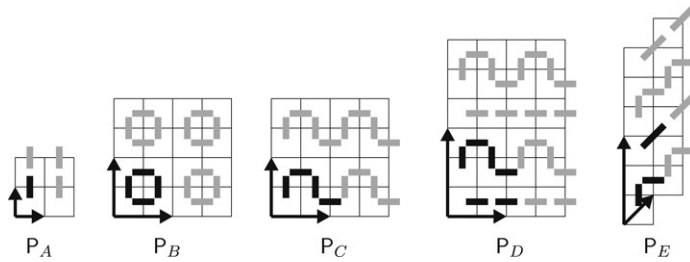
Fig. 5.1. 2-pavings. Each picture shows four copies of the fundamental set of tiles.
