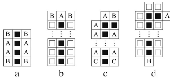
Fig. 4.2. Situations to achieve \mathcal{W}_n .
