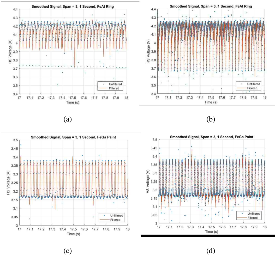
Figure 4.14: Peak FeAl Ring output experiences minimal reduction in response due to the implementation of a span-three moving average filter at a speed of 2000 RPM and a sampling rate of (a) 1000 Hz and (b) no reduction at 10000 Hz. Peak signal for a FeGa paint sample experiences minimal reduction due to implementation of a moving average filter at a sampling rate of (c) 1000 Hz and (d) no reduction at 10000 Hz.
