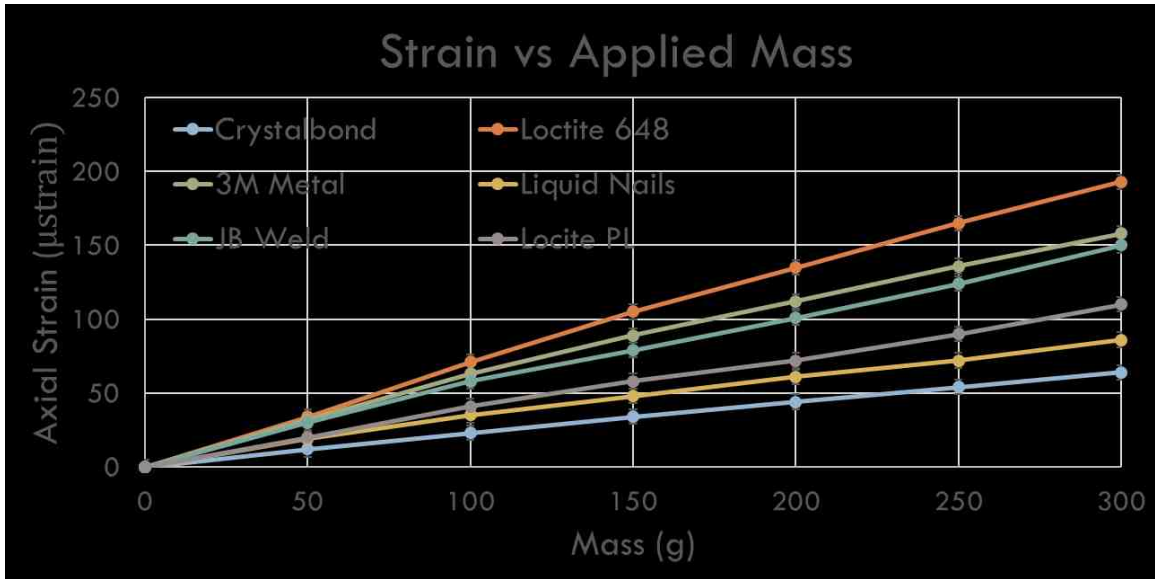
Figure 3.12: Initial bending tests on a thin aluminum sheet demonstrated the superior performance of Loctite 648.
