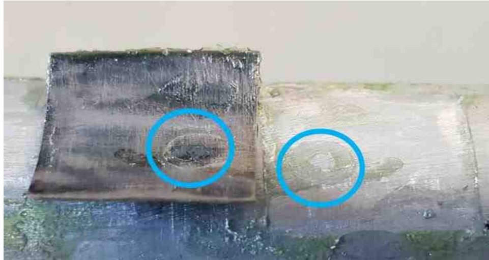
Figure 3.17: A non-uniform bond layer, with adhesive pooling around an air bubble, formed due to imperfect sanding of the shaft and shim sample.
