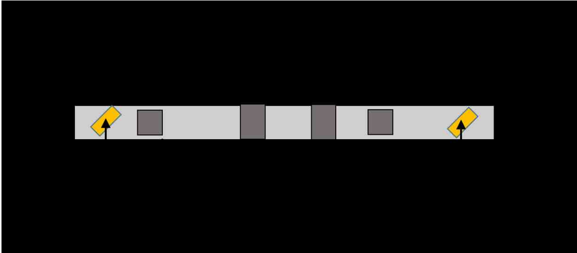
Figure 3.2: Magnetostrictive patches and rings were positioned along the 12 in long test section according to positions listed in Table 3.2 during quasi-static testing.
