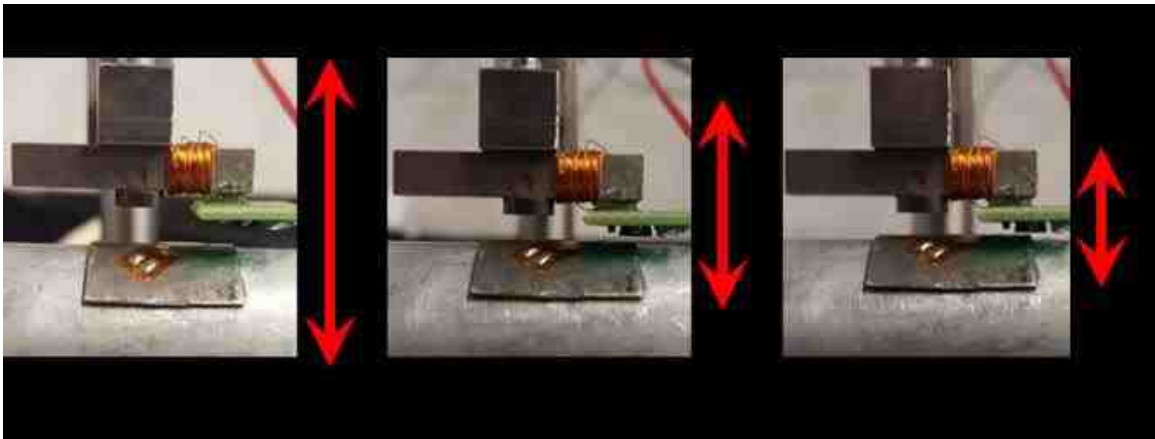
Figure 3.9: Hall effect sensor was mounted above the magnetostrictive patch at a height of (a) 0.05 in (b) 0.025 in (c) 0.01 in (arrows indicate trends, as actual air gaps are just barely discernable in this image).
