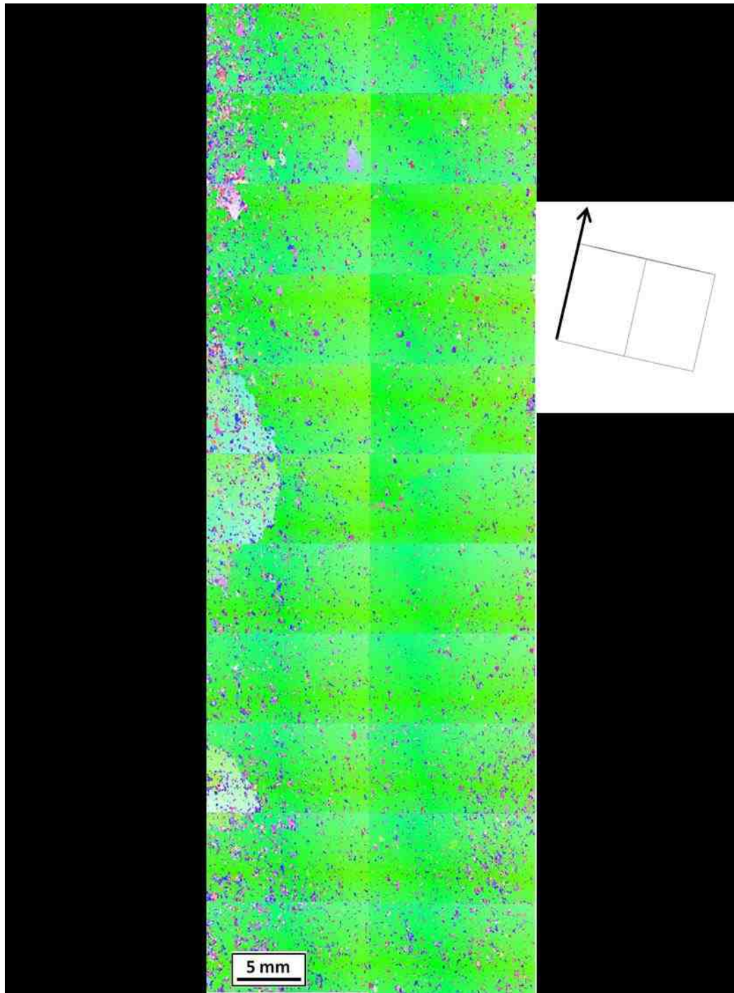
Figure A.2: EBSD-scanned image of FeAl rolled sheet that was used to create “FeAl Patch” sample for WiMET testing with a \langle 100 \rangle orientation along the circumference of the shaft.
