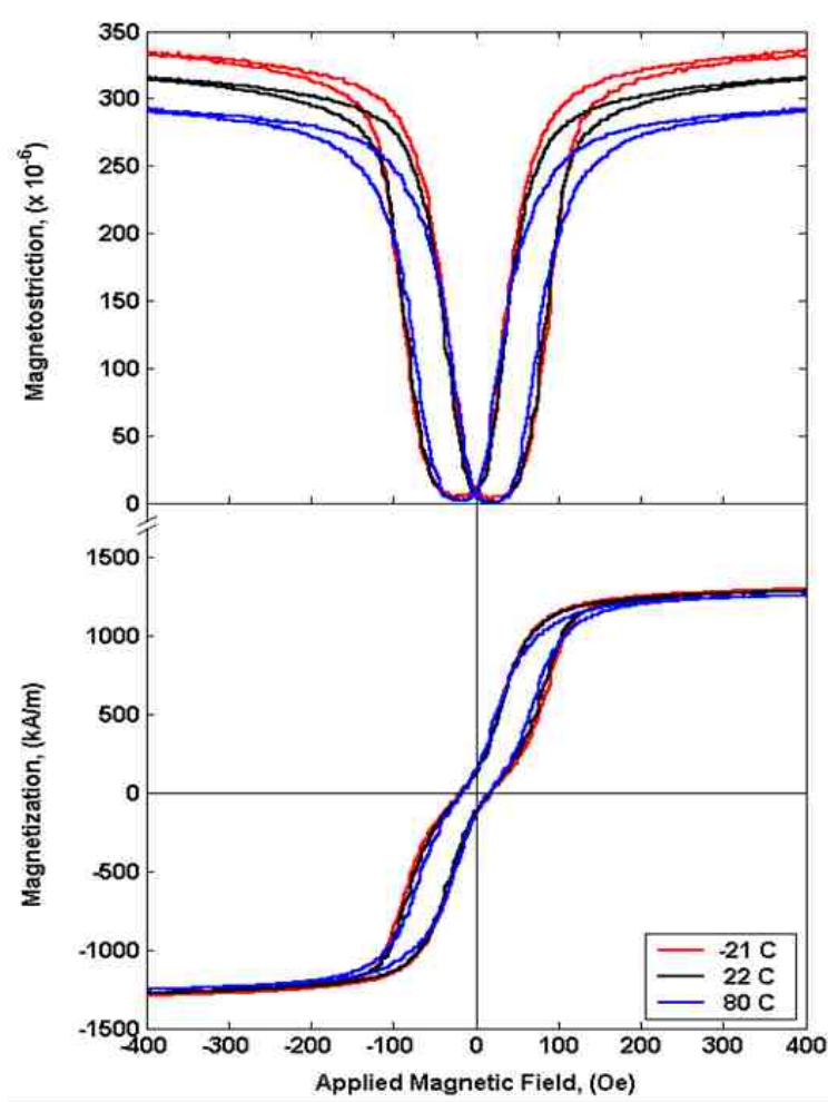
Figure 1.6: Magnetostriction (top) and magnetization (bottom) vary in a FeGa sample as applied magnetic field (Oe) is increased at -21°C, 22°C, and 80°C [26].
