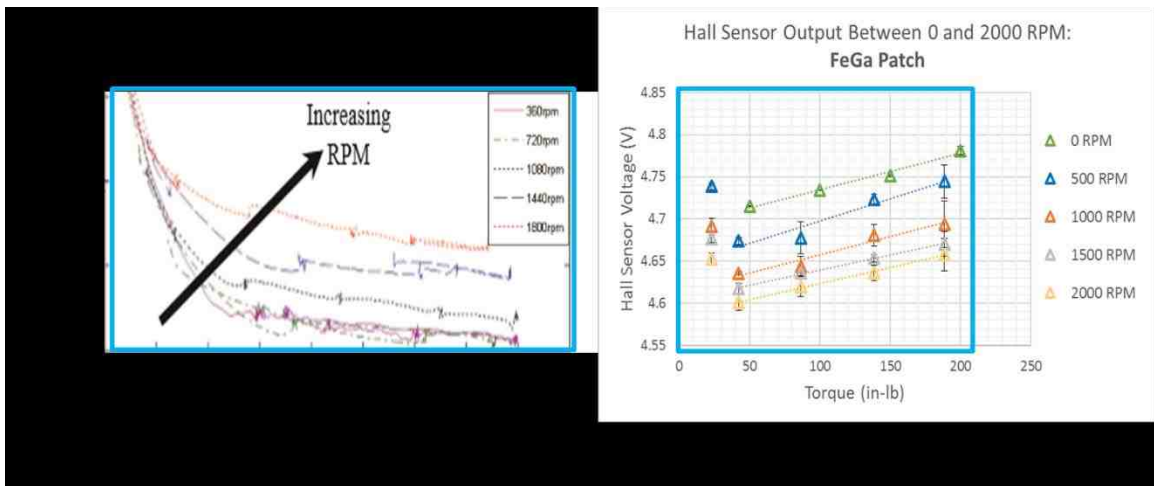
Figure 4.31: The updated WiMET configuration provided an output magnitude and sensitivity ~10 times greater than the prototype between ~ 44 and 188 in-lb.
