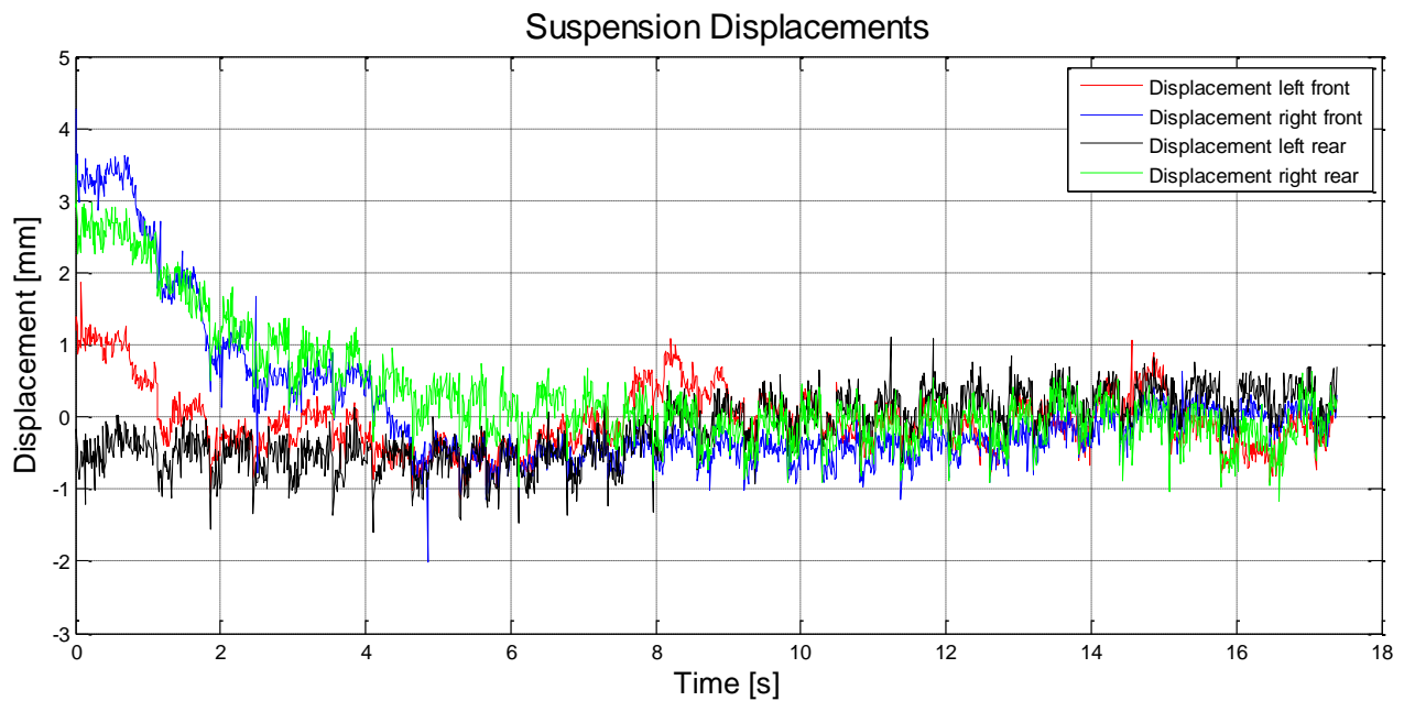
Figure 71 Suspension displacements
