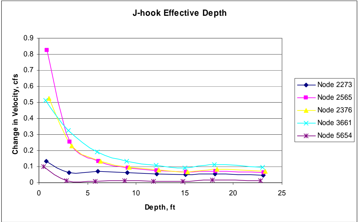
Figure 3-20. J-Hook Effective Depth from Change in Velocity Magnitude.
