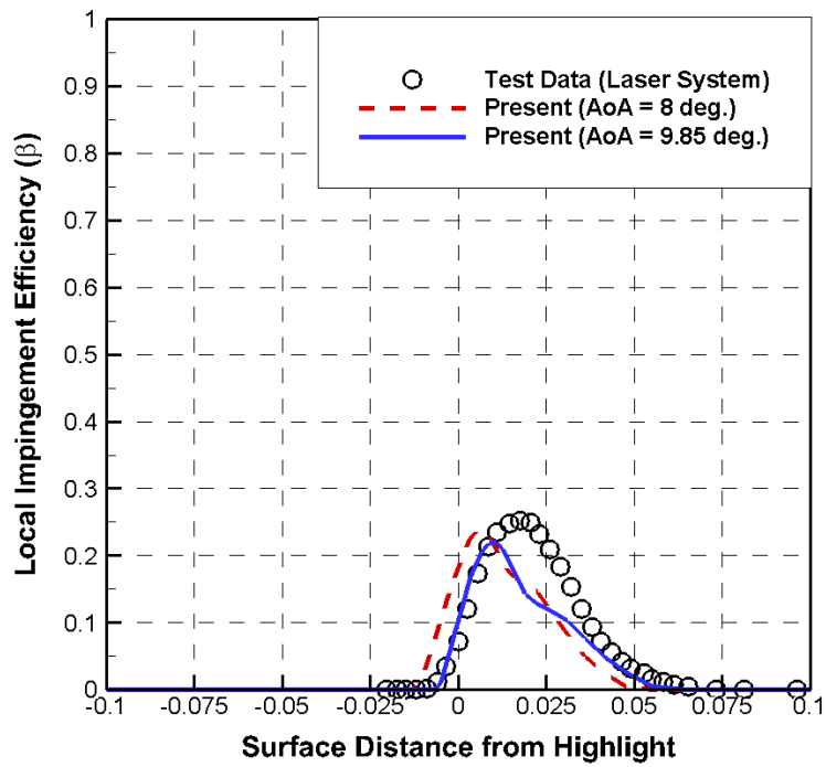
a) MVD = 11.5
