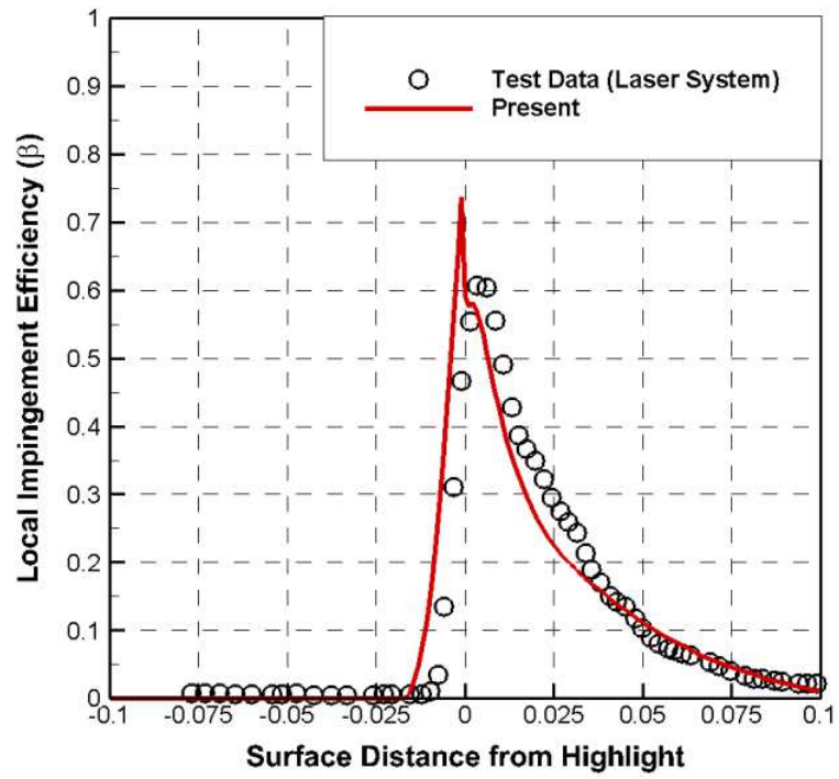
Figure 3.30: Comparison of Collection efficiency for NACA64A008 Swept Tail Section at 6 Degrees Angle of Attack (MVD=21).
