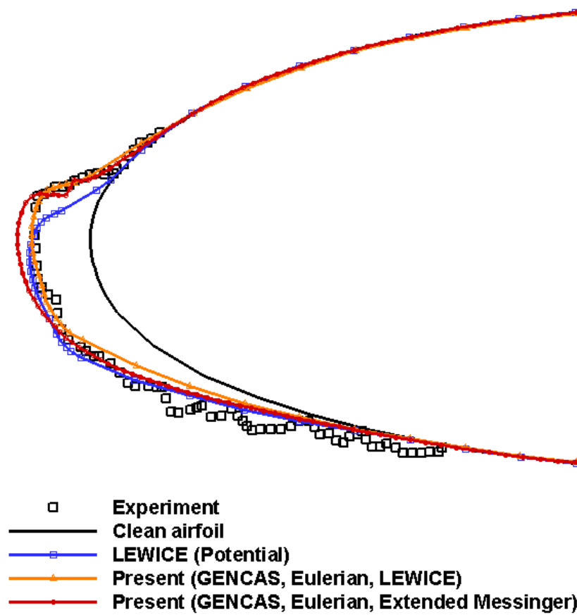
Figure 3.32: Predicted Ice Shape for NACA0012 (Run404).
