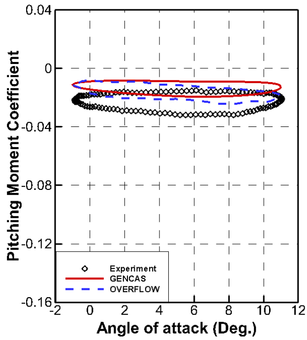
a) Clean Airfoil
