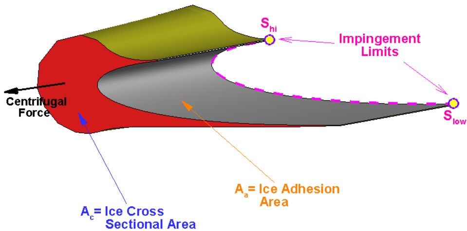
Figure 5.2: Ice Cohesion and Adhesion Forces Details.
