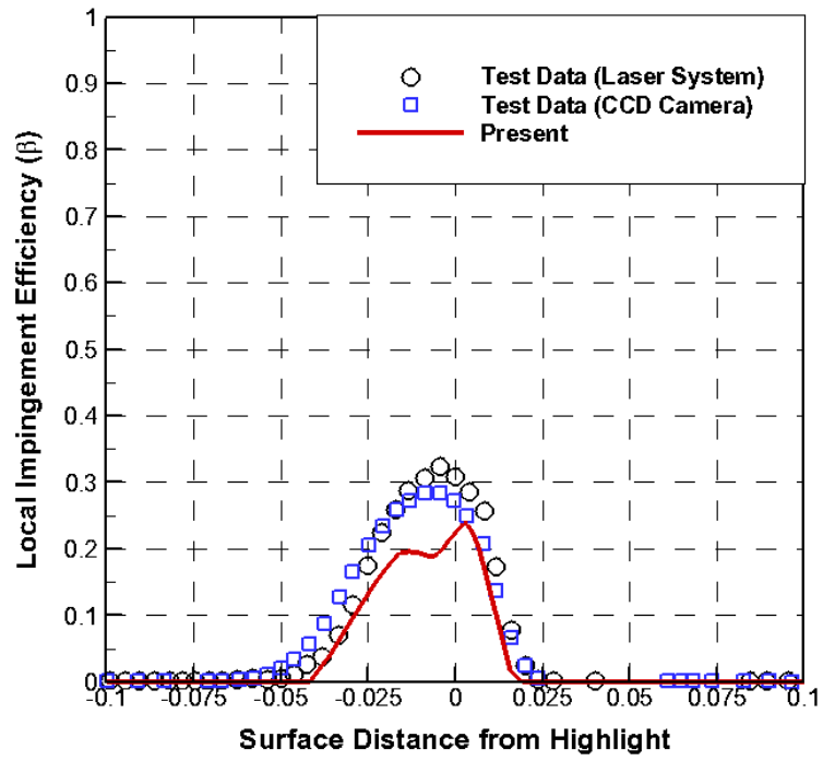
a) MVD = 11.5
