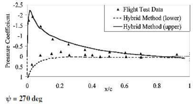
b) 91% Span ( Left : Present, Right : Ref. [82] )
