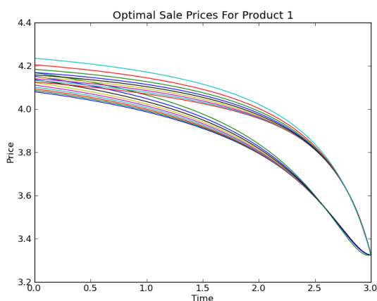
Figure 6.10: Optimal sales price strategy in a monopolistic market with differentiated, substitutes. Let \lambda_1(p_1, p_2) = 15 - 4p_1 + 1p_2 , \lambda_2(p_1, p_2) = 10 + 2p_1 - 7p_2 , C_{a,0} = 3.5 , C_{b,0} = 1 , C_{a,T} = 2 , and C_{b,T} = 0.5 , and T = 3 .
