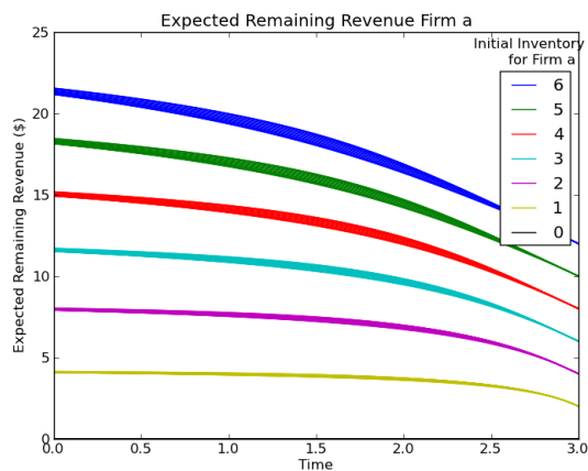
Figure 6.18: Expected remaining revenue of firm one in a duopolistic market with differentiated, complementary goods. Let \lambda_1(p_1, p_2) = 15 - 3p_1 - 1p_2 , \lambda_2(p_1, p_2) = 20 - 2p_1 - 7p_2 , C_{a,0} = 3 , C_{b,0} = 1 , C_{a,T} = 2 , and C_{b,T} = 0.5 , and T = 3 .
