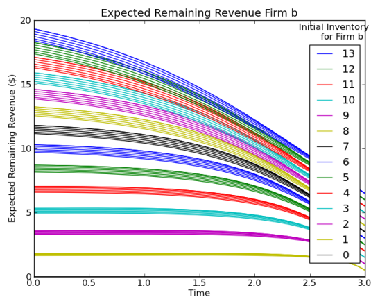
Figure 6.19: Expected remaining revenue of firm two in a duopolistic market with differentiated, complementary goods. Let \lambda_1(p_1, p_2) = 15 - 3p_1 - 1p_2 , \lambda_2(p_1, p_2) = 20 - 2p_1 - 7p_2 , C_{a,0} = 3 , C_{b,0} = 1 , C_{a,T} = 2 , and C_{b,T} = 0.5 , and T = 3 .
