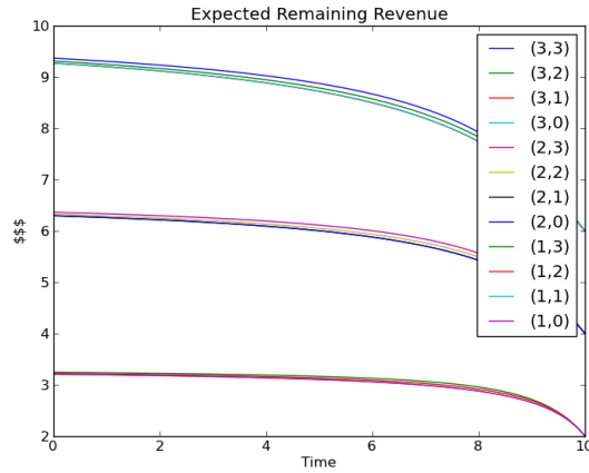
Figure 4.4: Expected remaining revenue for complementary goods in a duopolistic market. Assume I_{a,0} = I_{b,0} = 3 , \lambda_1(p_1, p_2) = 10 - 2p_1 - p_2 , \lambda_2(p_1, p_2) = 10 - p_1 - 2p_2 , C_{a,0} = C_{b,0} = 3 , C_{a,T} = C_{b,T} = 2 , and T = 10 .
