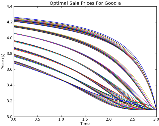
Figure 6.21: Optimal sales price strategy of firm one in a monopolistic market with differentiated, complementary goods. Let \lambda_1(p_1, p_2) = 15 - 3p_1 - 1p_2 , \lambda_2(p_1, p_2) = 20 - 2p_1 - 7p_2 , C_{a,0} = 3 , C_{b,0} = 1 , C_{a,T} = 2 , and C_{b,T} = 0.5 , and T = 3 .
