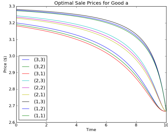
Figure 5.3: Optimal sale prices in a monopolistic market for complementary goods. Assume I_{a,0} = I_{b,0} = 4 , \lambda_1(p_1, p_2) = 10 - 2p_1 - p_2 , \lambda_2(p_1, p_2) = 10 - p_1 - 2p_2 , C_{a,0} = C_{b,0} = 3 , C_{a,T} = C_{a,T} = 2 , and T = 10 .
