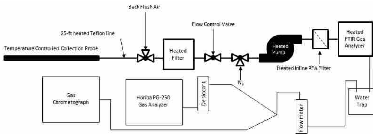
Figure 9: Schematic Diagram of the Components and Analyzers of the Gas Sampling System.
