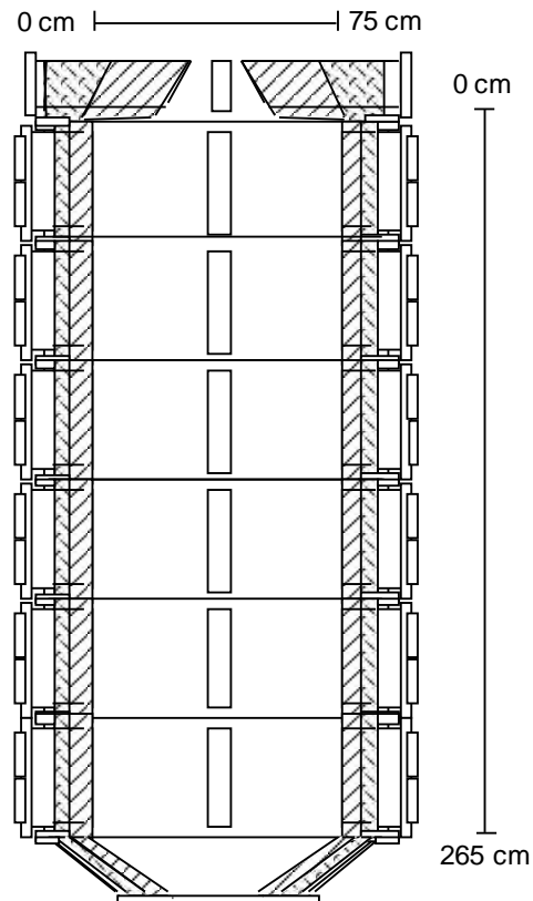
Figure 41: Dimensions of the BFR for Use in Analyzing Data.
