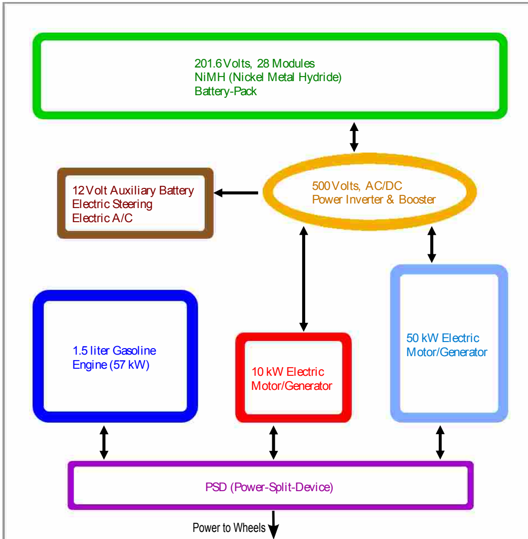
Figure 2.7: Power Flow For Prius Powertrain [17]
