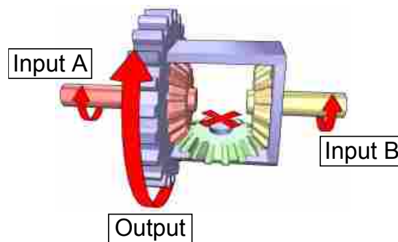
Figure 3.2: Simplified Differential - 2 Inputs, 1 Output [6]
