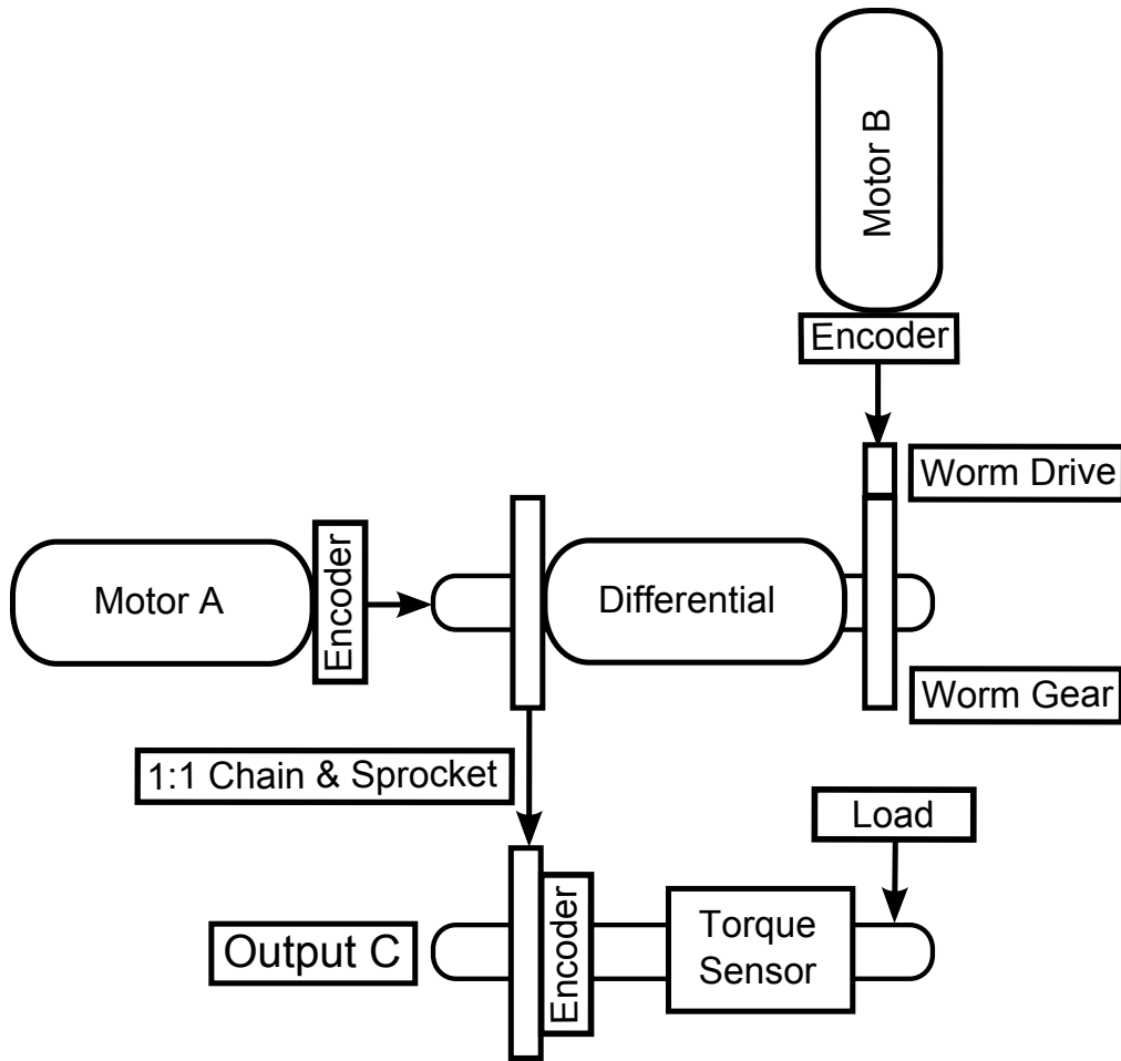
Figure 5.15: Minimizing Backdrive - Worm Drive
