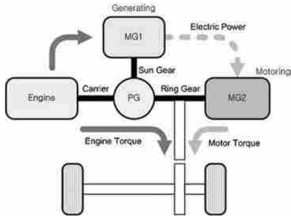
Figure 2.8: Prius Powertrain [3]
