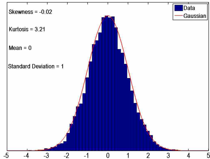
Figure 3.10 A histogram plot for an array of random numbers plotted against a Gaussian curve. The first four standard moments are shown for the array of random numbers, with the skewness and kurtosis values confirming numerically its Gaussian nature.
