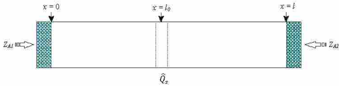
FIG. 4.1. A theoretical one dimensional tube model. The tube is terminated at x=0 and x=l with acoustic impedances Z_{A1} and Z_{A2} respectively. The sound field is excited by a plane monopole source at x=l_0 .
