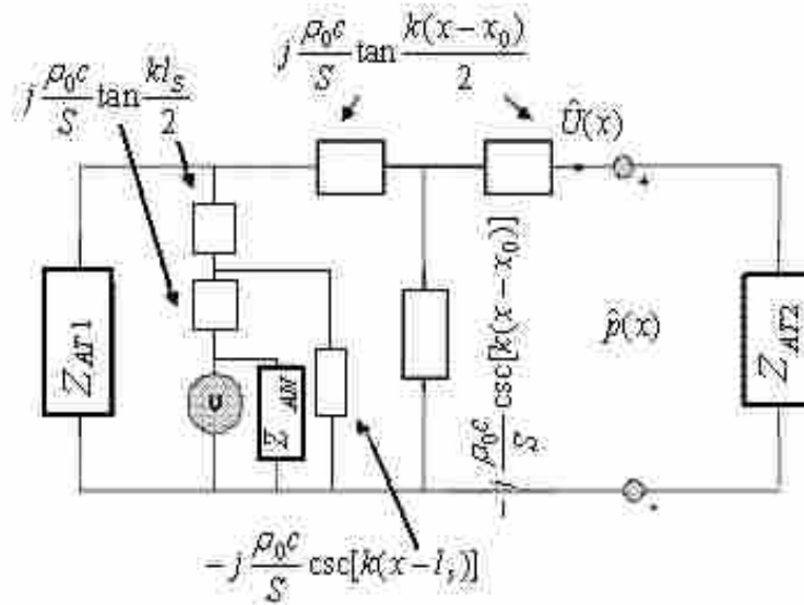
FIG. 4.3. The equivalent circuit after the impedance translation.
