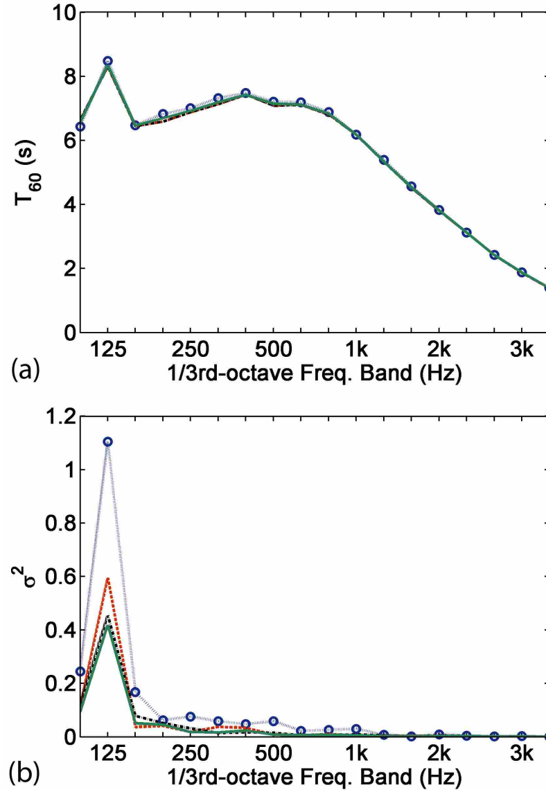
Figure 4.3 Reverberant time measurements using GED. (a) The averaged T_{60} estimation based on different GED quantities for a reverberation chamber. (b) Comparison of the variances of the T_{60} estimations due to the different source-receiver locations. “ \cdots \bigcirc \cdots ”: E_{G(1)}(E_P) ; “ --- ”: E_{G(0)}(E_K) ; “ -.- ”: E_{G(1/2)}(E_T) ; “ --- ”: E_{G(1/4)} .
