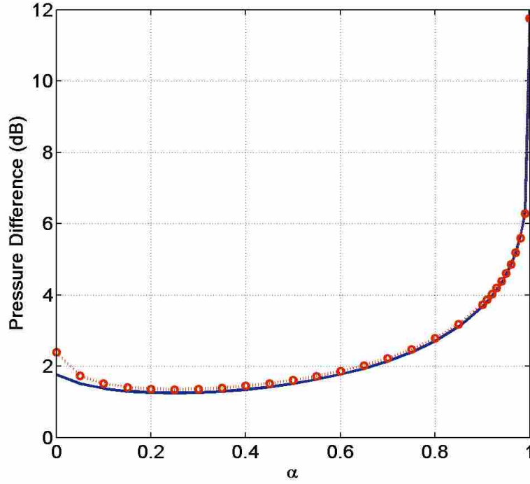
Figure 5.4 Averaged mean squared pressure at the remote location from the error sensor when GED is minimized. Eq. (5.26) is evaluated numerically and 10\log(1 + \frac{\mu_s^2}{\mu_p^2}) is plotted. “—”: analytical results; “ \cdot \cdot \bigcirc \cdot \cdot ”: numerical simulation.
