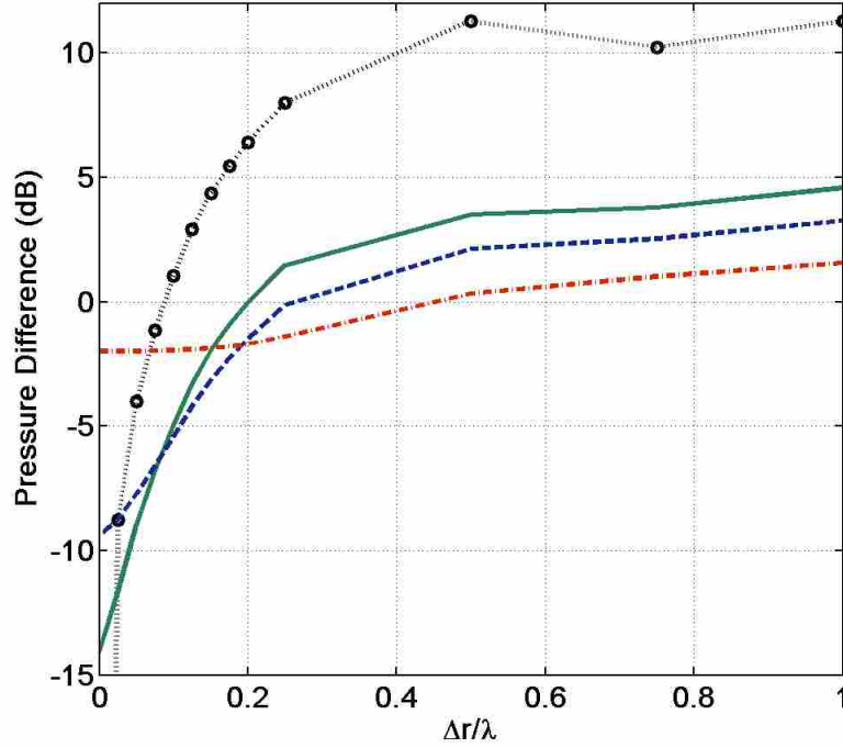
Figure 5.6 Averaged mean square pressure in the near-field of the error sensor when GED is minimized. This is a computer simulation result. “ \cdot \cdot \bigcirc \cdot \cdot ”: E_{G(1)} ( E_P ); “—”: E_{G(0.95)} ; “- -”: E_{G(0.85)} ; “- . - .”: E_{G(1/4)} .
