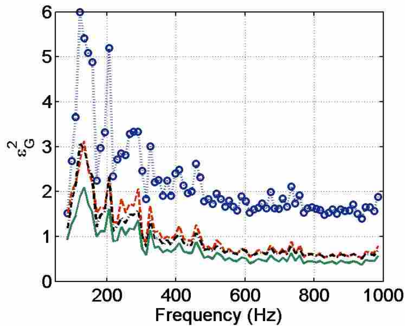
Figure 3.7 Numerical simulation results for the ensemble variance of different GED quantities for a lightly damped room. “ \cdot \cdot \bigcirc \cdot \cdot ”: E_{G(1)}(E_P) ; “ - - ”: E_{G(0)}(E_K) ; “ - \cdot - ”: E_{G(1/2)}(E_T) ; “ - ”: E_{G(1/4)} .
