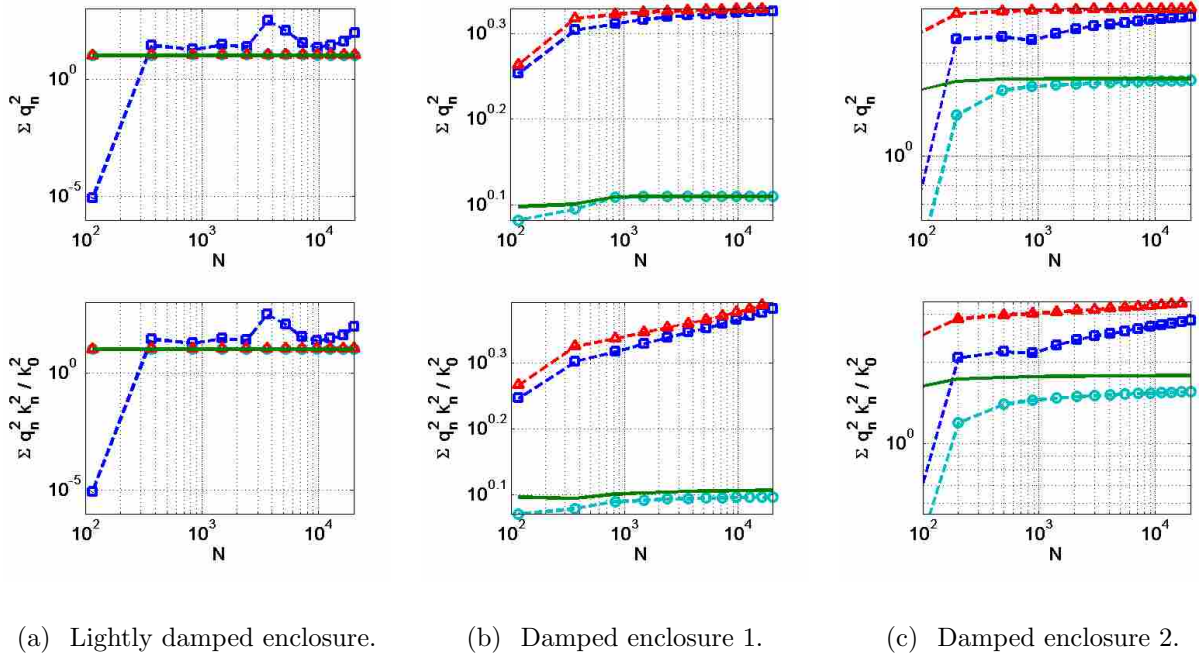
Figure 2.4 Convergence speed of the coupled modal expansion models for enclosures with different boundary conditions [(a) lightly damped, (b) damped 1, and (c) damped 2] at 400 Hz. “—□—”: CMA; “—○—”: GCMA; “—△—”: MMA; “—”: GMMA.
