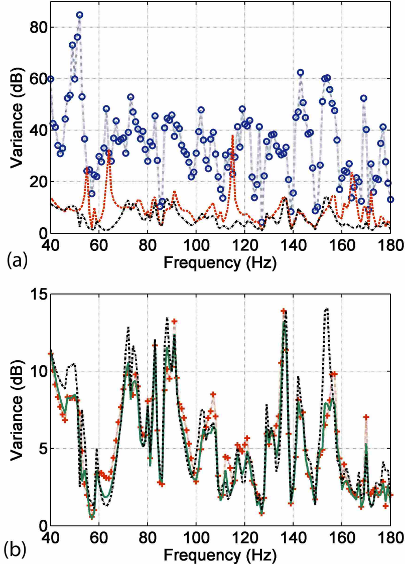
Figure 5.2 Variance of the attenuation. (a) Variance of the attenuation for E_{G(1)} ( E_P , “ \cdot\cdot\bigcirc\cdot\cdot ”), E_{G(0)} ( E_K , “ - - ”) and E_{G(1/2)} ( E_T , “ - \cdot - ”). (b) Variance of the attenuation for E_{G(1/2)} (“ - \cdot - ”), E_{G(1/4)} (“ - ”) and E_{G(1/10)} (“ \cdot\cdot + \cdot\cdot ”).
