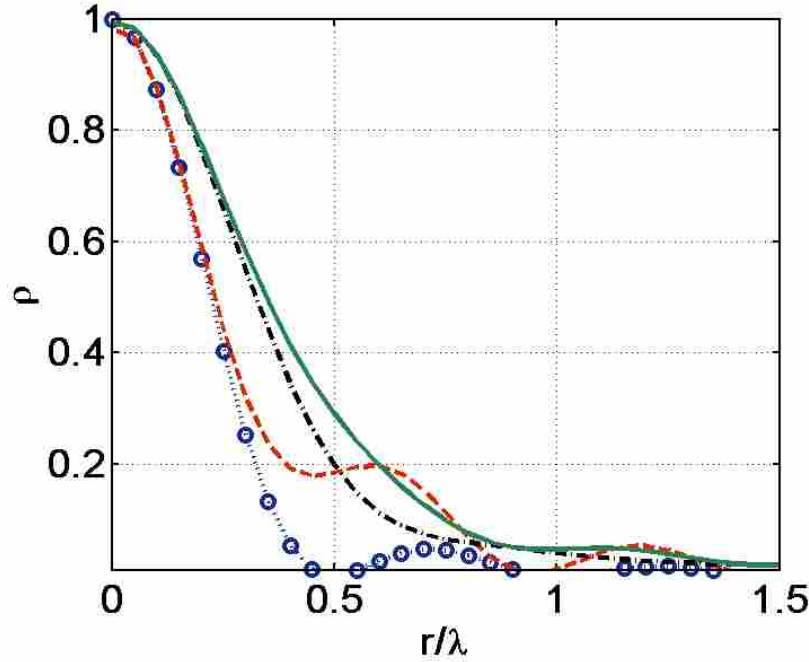
Figure 3.3 Spatial correlation coefficient \rho of different GED quantities in a diffuse field. “ \cdot \cdot \bigcirc \cdot \cdot ”: E_{G(1)} ( E_P ); “ - - ”: E_{G(0)} ( E_K ); “ - \cdot - ”: E_{G(1/2)} ( E_T ); “ - ”: E_{G(1/4)} .
