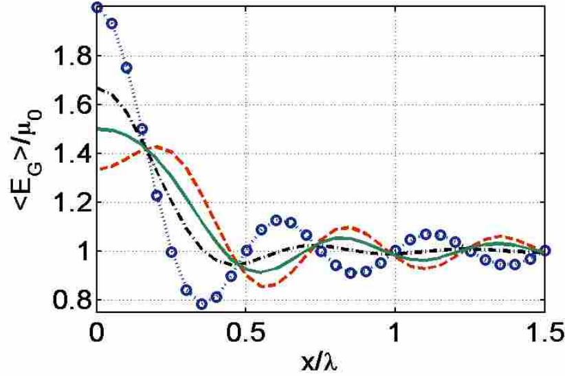
Figure 3.4 Mean values of different GED quantities as a function of the distance, x , from a flat rigid boundary in a diffuse field. “ \cdots \bigcirc \cdots ”: E_{G(1)} ( E_P ); “ --- ”: E_{G(0)} ( E_K ); “ -\cdot- ”: E_{G(1/2)} ( E_T ); “ — ”: E_{G(1/4)} .
