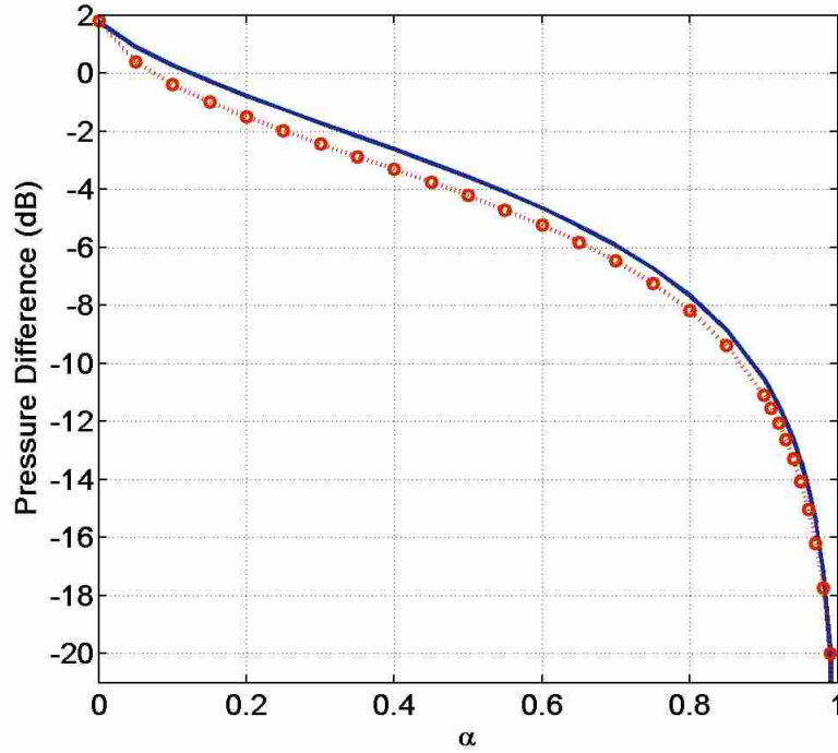
Figure 5.3 Averaged mean square pressure at the error sensor location when GED is minimized. Eq. (5.20) is evaluated numerically and 10\log(\overline{p^2(\mathbf{r}_0)} / \overline{p_p^2}) is plotted. “—”: analytical results; “ \cdot\cdot\bigcirc\cdot\cdot ”: numerical simulation.
