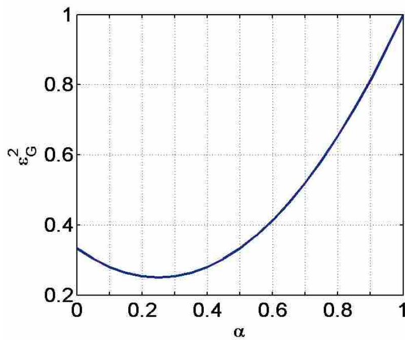
Figure 3.2 Relative spatial variance of GED in a diffuse field. The minimum variance is reached at \alpha = 1/4 .
