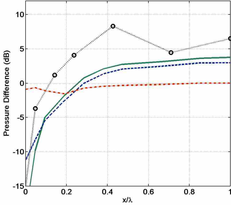
Figure 5.8 Experimental results for averaged mean square pressure in the near-field of the error sensor when GED is minimized. “ \cdots \bigcirc \cdots ”: E_{G(1)} (E_P) ; “—”: E_{G(0.95)} ; “— —”: E_{G(0.85)} ; “-.-.-”: E_{G(1/4)} .
