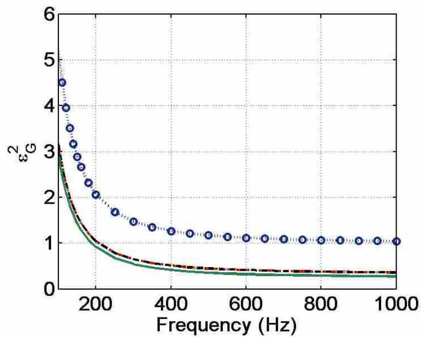
Figure 3.6 Ensemble variance of different GED quantities for a reverberation chamber with V = 136.6 \text{ m}^3 and uniform T_{60} = 6.2 \text{ s} . “ \cdot \cdot \bigcirc \cdot \cdot ”: E_{G(1)} (E_P) ; “ -\cdot - ”: E_{G(0)} (E_K) ; “ - \cdot - ”: E_{G(1/2)} (E_T) ; “ - ”: E_{G(1/4)} .
