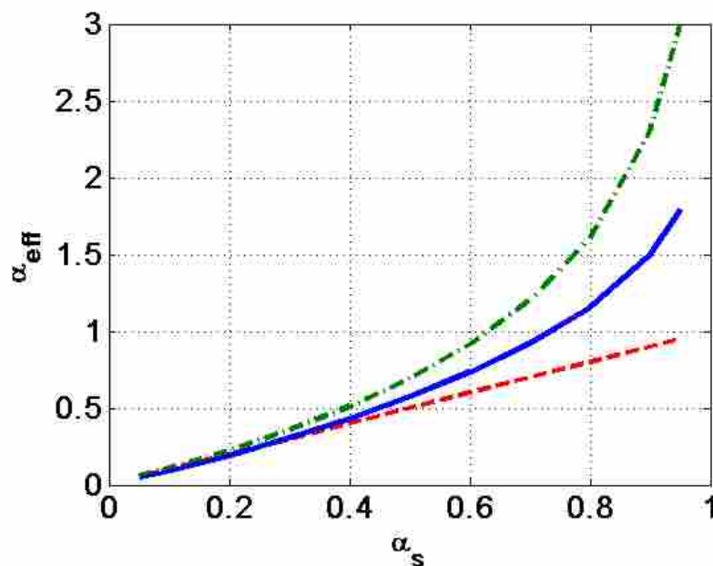
Figure 2.9 Effective absorption coefficient as a function of Sabine’s absorption coefficient calculated in a rectangular room for the 630 Hz one-third octave band. “—”: GMMA prediction; “- -”: Sabine’s formula; “- · -”: Eyring’s formula.
