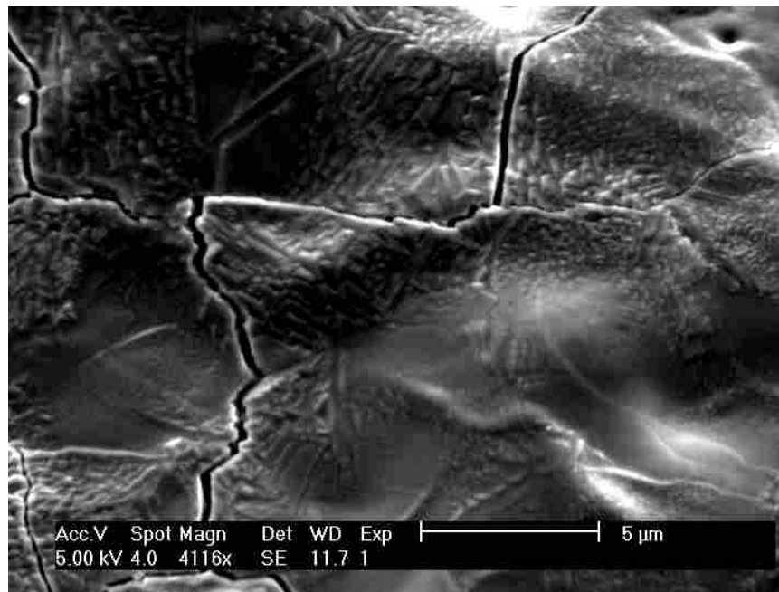
Figure 4.16 SEM photo of the primary ablation region, showing melting, fracturing, and crystal formation.
