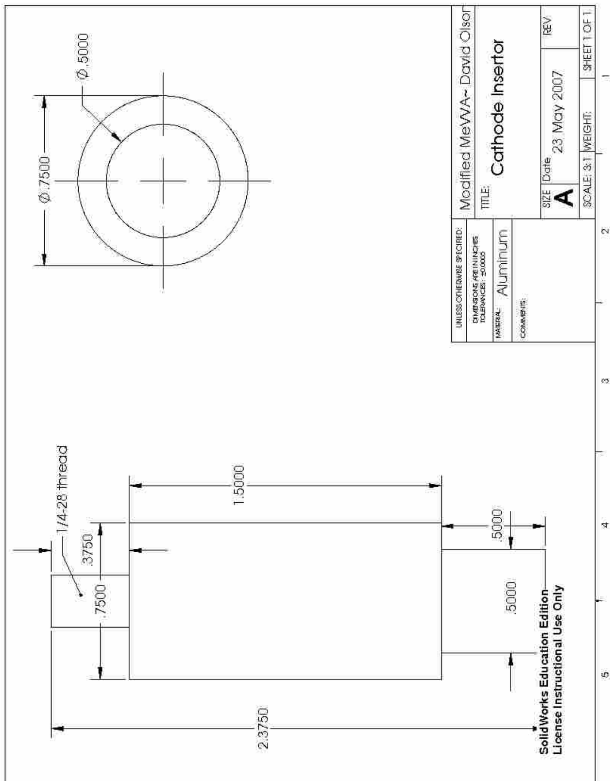
Figure A.12 Insertor Machining Drawing
