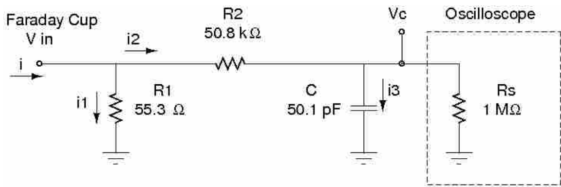
Figure B.2 The Passive Integrator Circuit
