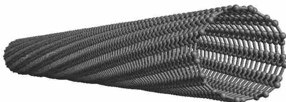
Figure 1.1 A single-walled carbon nanotube. Rendered in Mathematica from coordinate data produced with TubeVBS.
