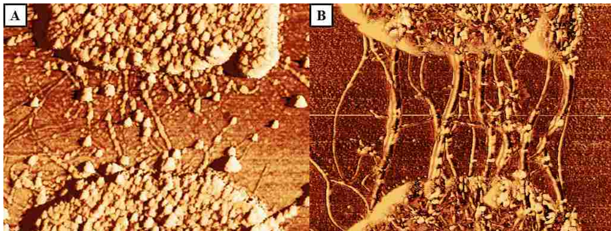
Figure 4.8 AFM phase data showing many localized CNTs. A) Using geometry 6 to decouple the FE from the fluid in an attempt to more closely couple the FEs together after CNT deposition. B) Using highly resistive fluid to have a more dramatic effect upon CNT deposition. These results were typical of many devices, indicating that binary shutoff was not operative under the tested conditions.
