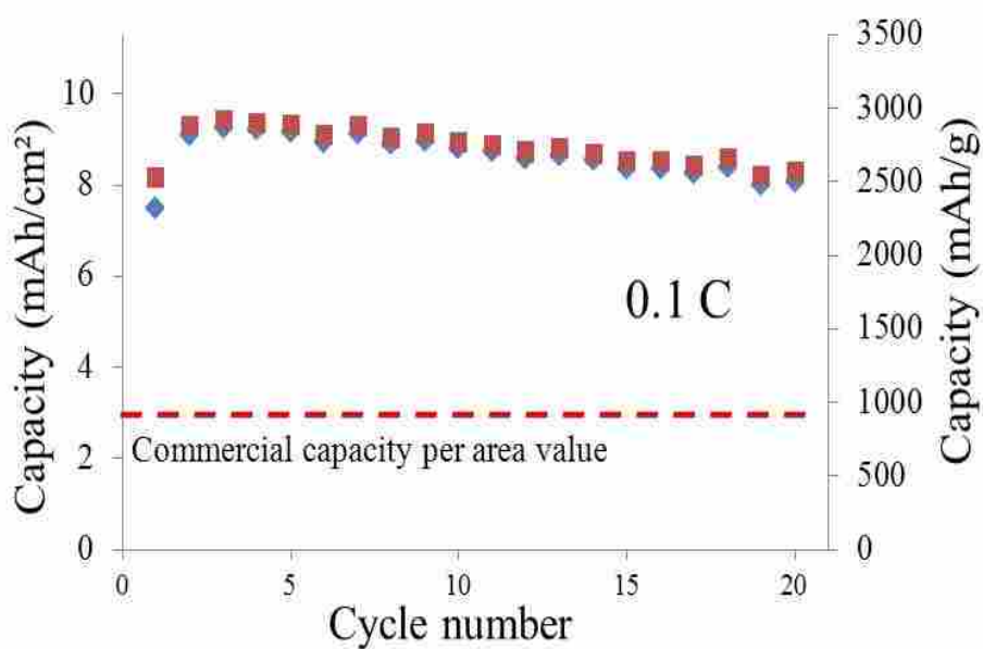
Figure 4.5 The capacity per area of a Si/CNT composite electrode with a thickness of 19.4 \mu\text{m} , a Si:CNT mass ratio of 51:1, and a volumetric silicon loading of 1.6 \text{g}/\text{cm}^3 . Charge (square) and discharge (diamond) capacities at a rate of 0.1 C are shown versus cycle number
