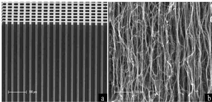
Figure 2.3 SEM images of VACNTs. (a) CVD synthesis of patterned CNTs on a silicon wafer. (b) a close-up view of VACNTs.
