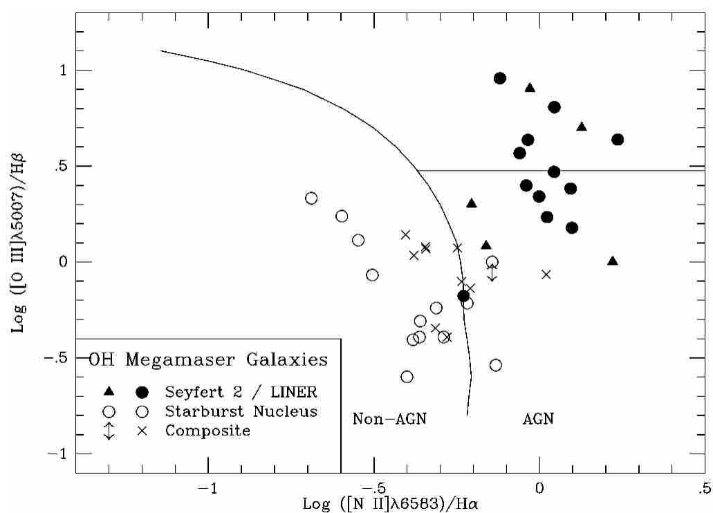
Figure B.2 Diagnostic diagram describing the separation of classifications between AGN, Starburst and composite sources. 45 The two lines indicate the dividing line between AGN, non-AGN and composite sources.
