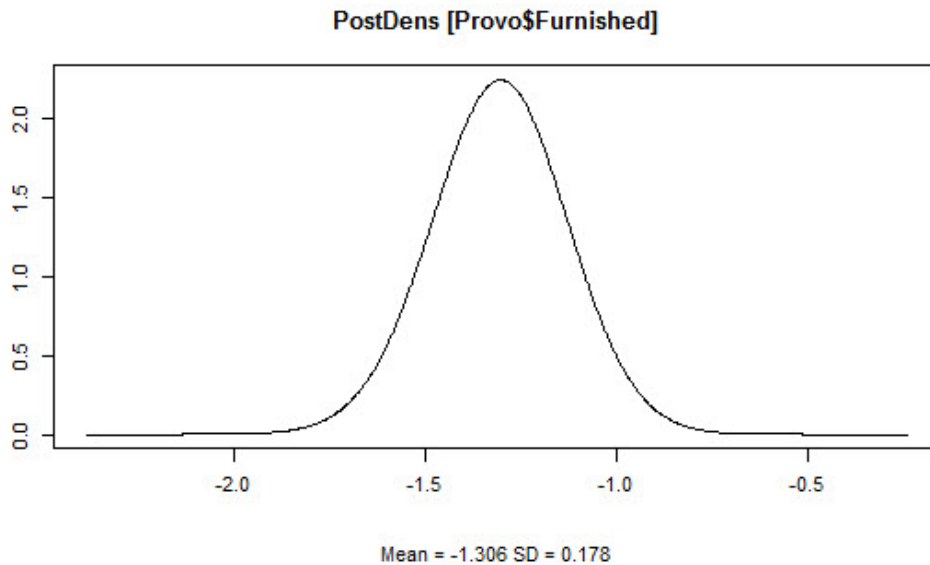
Figure 5.4: Posterior Distribution of Furnished Effect
