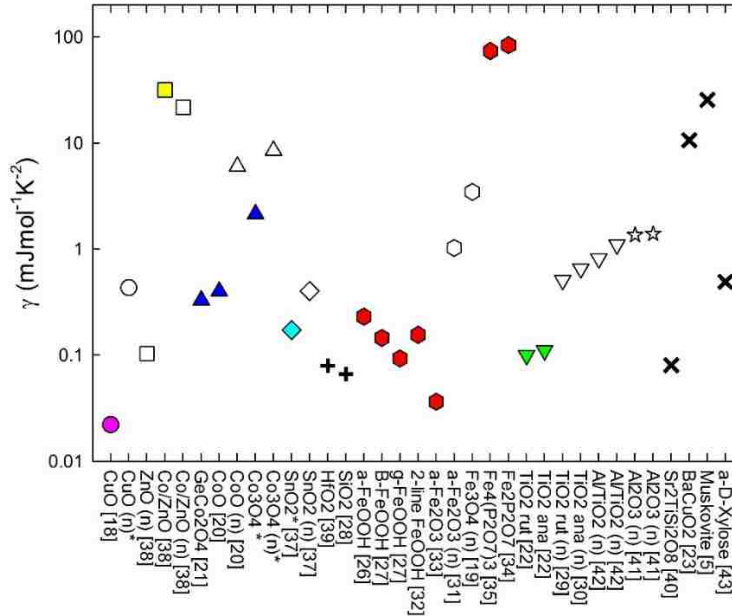
Figure 4-1: Selected Linear Terms, \gamma , from Low-temperature Heat Capacity Fits. Hollow symbols represent the nanophasse of the material; solid symbols represent bulk.
