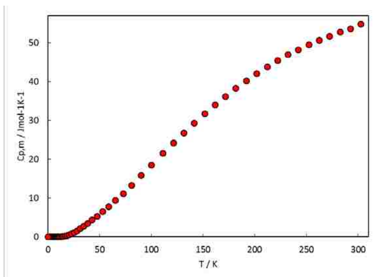
Figure 2-5: Heat Capacity of a Bulk Rutile \text{TiO}_2 Standard Collected on a PPMS
