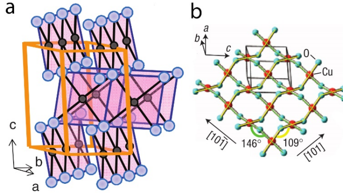
Figure 7-1: Structure of CuO Showing a) Edge-shared Ribbon Chains of CuO 2 (from Wu et al. 15 with permission) and b) Zigzag Chains along the [101] (yellow lines) and [101̄] (green lines) Directions (from Kimura et al. 10 with permission).
