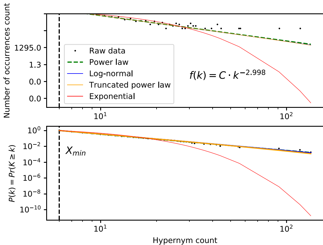
Fig. 7. Hypernym frequency distribution for the PAN 2016 (Age) data set. The equation above the upper plot denotes the coefficients of a power law distribution ( C is a constant). In real world phenomena, the exponent of the rightmost expression was observed to range between \approx 2 and \approx 3 , indicating the hypernym structure of the feature space is subject to a heavy-tailed (possibly best fit—power law) distribution. The X_{min} denotes the hypernym count, after which notable differences in hypernym counts—scale free behavior is observed. Such distribution is to some extent expected, as some hypernyms are more general than others, and thus present in more document-hypernym mappings.
