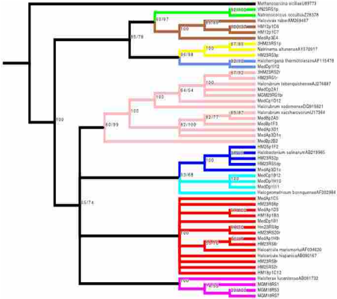
Figure 4. Archaeal phylogenetic tree. Archaeal consensus tree of nodes in agreement between ML trees and Bayesian trees. The first number at the node is the bootstrap probability for ML and the second is a posterior probability for Bayesian. Colors coordinate to different genera, with isolates grouped according to 16S rDNA similarity in GenBank.
