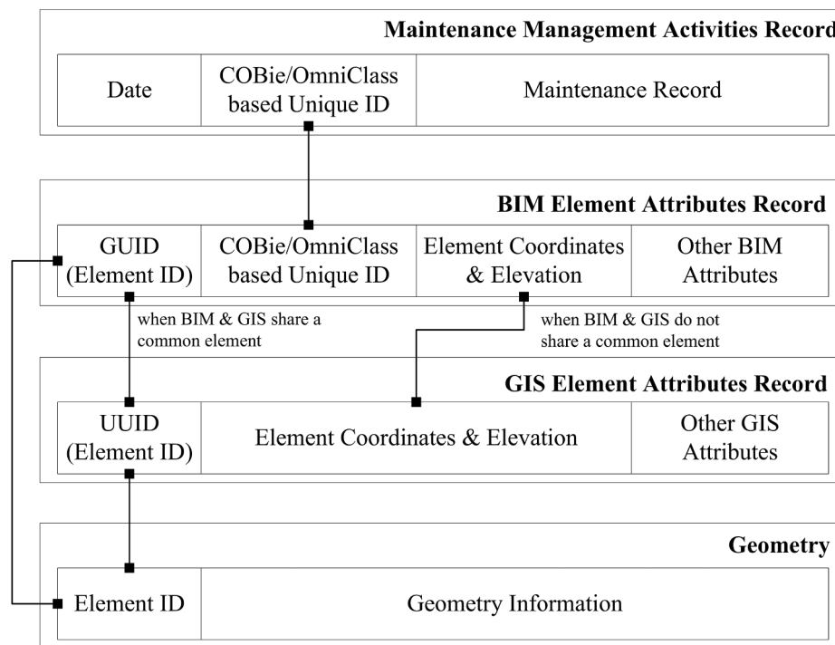
Fig. 3. Data linking layer of the proposed framework.
