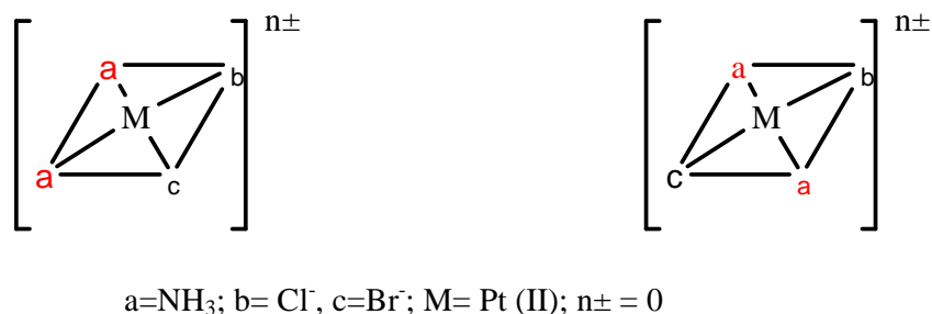
Figure 7.10: cis - and trans - isomers of [Ma 2 bc] n± type compounds
