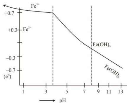
Figure 8.8: Pourbaix diagram of iron
