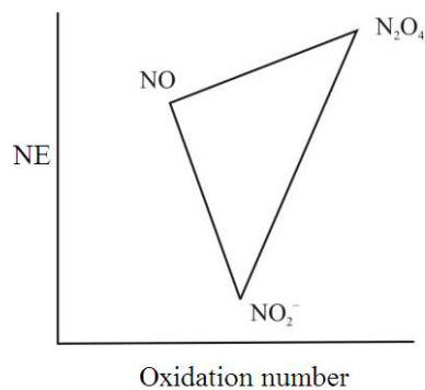
Figure 8.4: Frost diagram showing comproportionation
