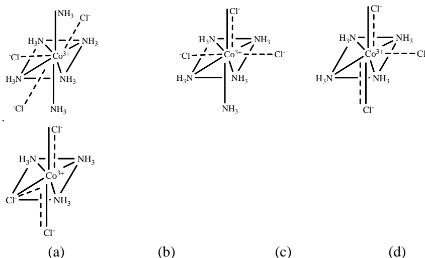
Figure 6.3 Structure of Co(III) amine complexes on the basis of Werner's theory. In all the complexes the primary valency of Co is 3 and secondary valency is 6. (a) CoCl_3 \cdot 6NH_3 [Co(NH_3)_6]Cl_3 (b) CoCl_3 \cdot 5NH_3 [Co(NH_3)_5Cl]Cl_2 (c) CoCl_3 \cdot 4NH_3 [Co(NH_3)_4Cl_2]Cl (d) CoCl_3 \cdot 3NH_3 [Co(NH_3)_3Cl_3]
