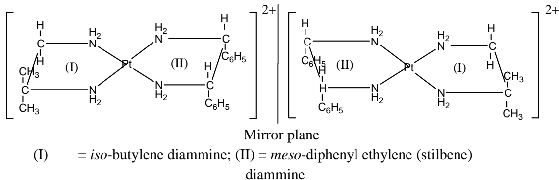
Figure 7.23: Square planar complex showing optical isomerism
