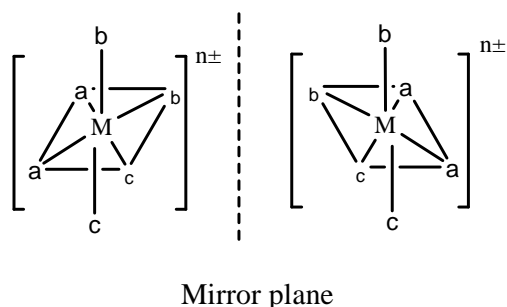
Figure 7.27: Optical isomerism in [Ma_2b_2c_2]^{n\pm} type compounds
